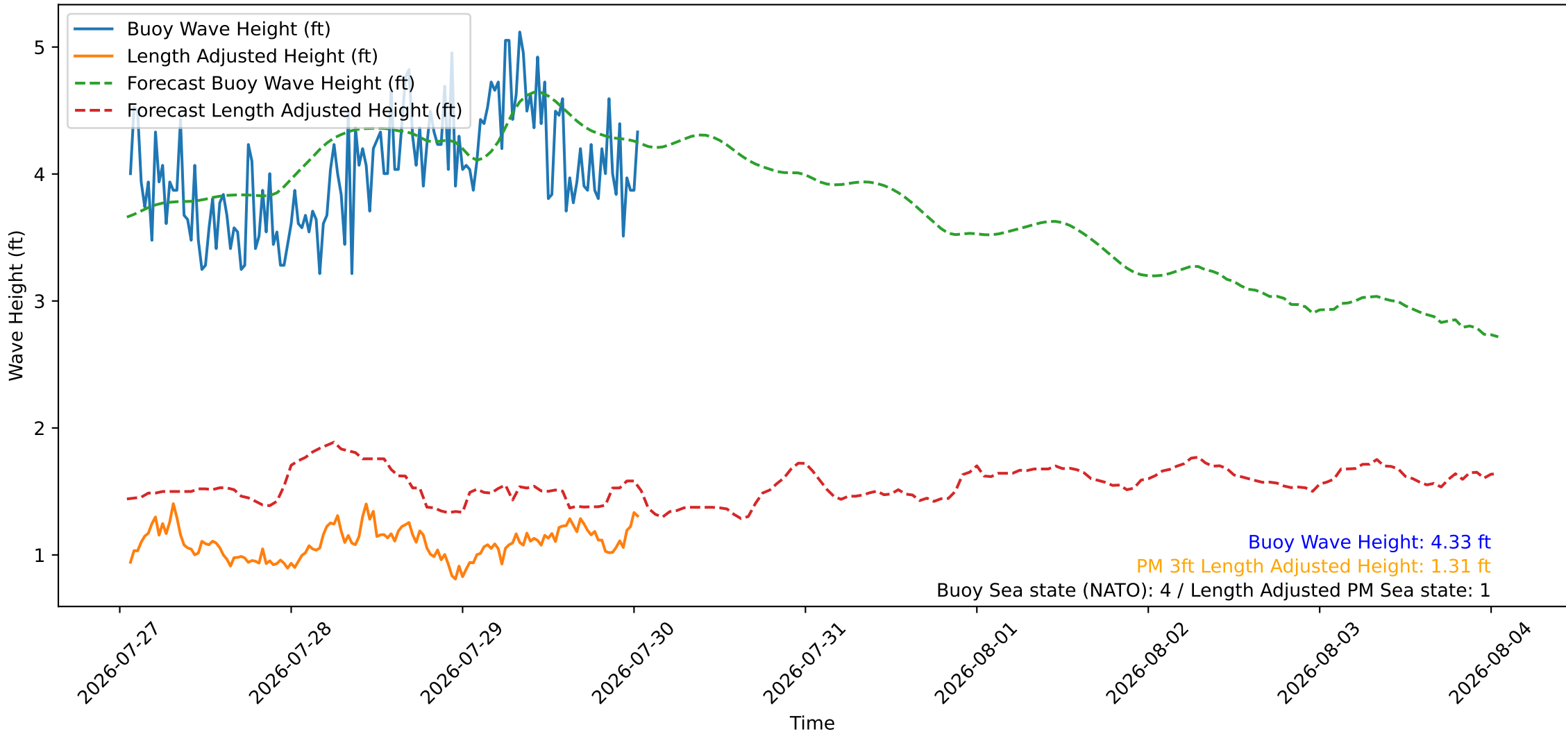
Wave Heights over Time for Red Beach at 2026-07-30 01:10:45
