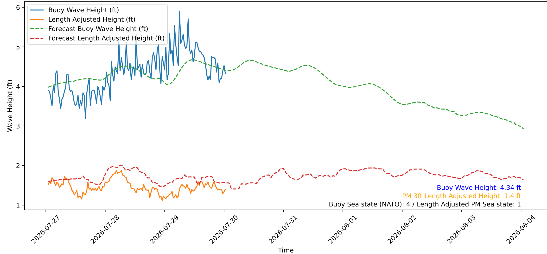
Wave Heights over Time for Oceanside Harbor at 2026-07-30 01:10:26
