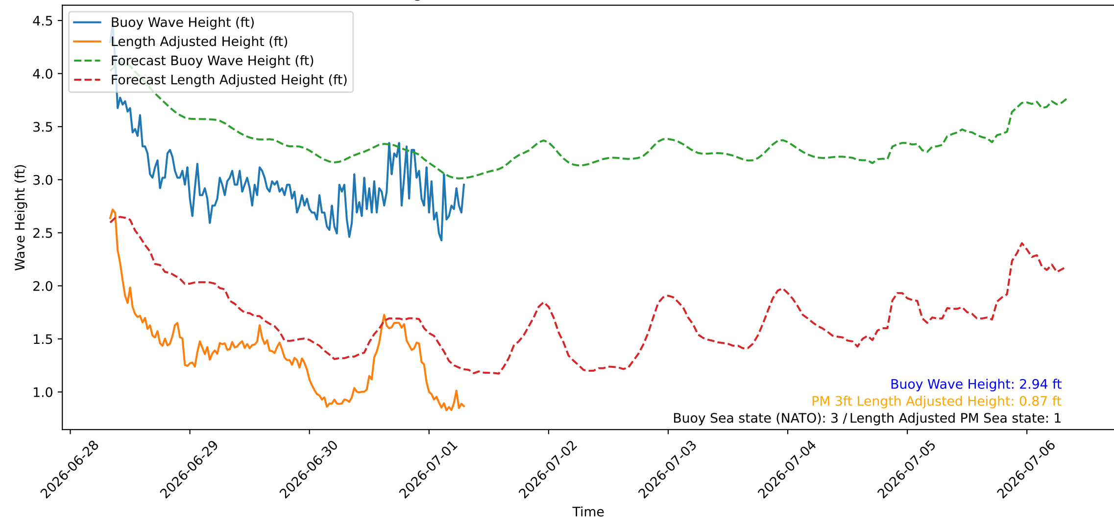
Wave Heights over Time for Red Beach at 2026-07-01 07:50:46
