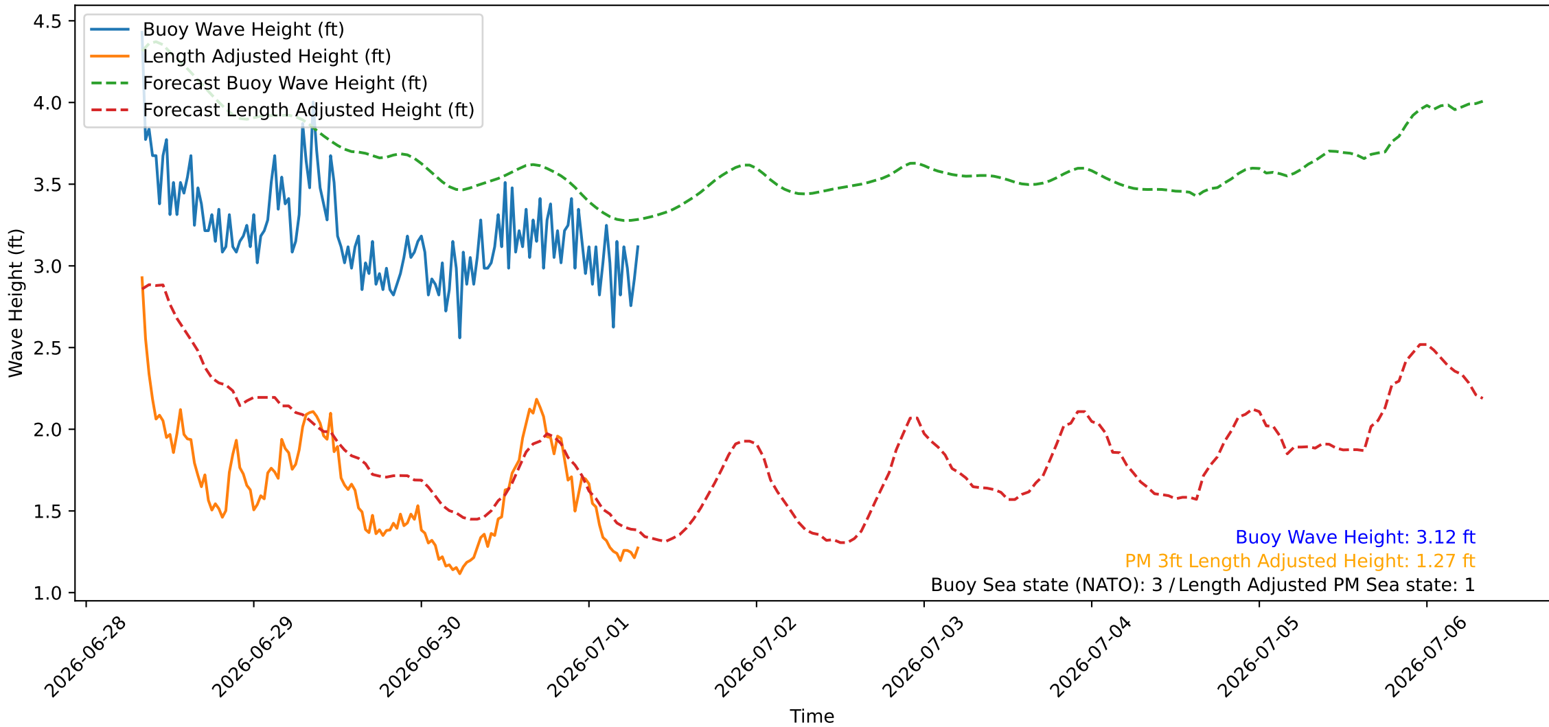
Wave Heights over Time for Oceanside Harbor at 2026-07-01 07:50:26
