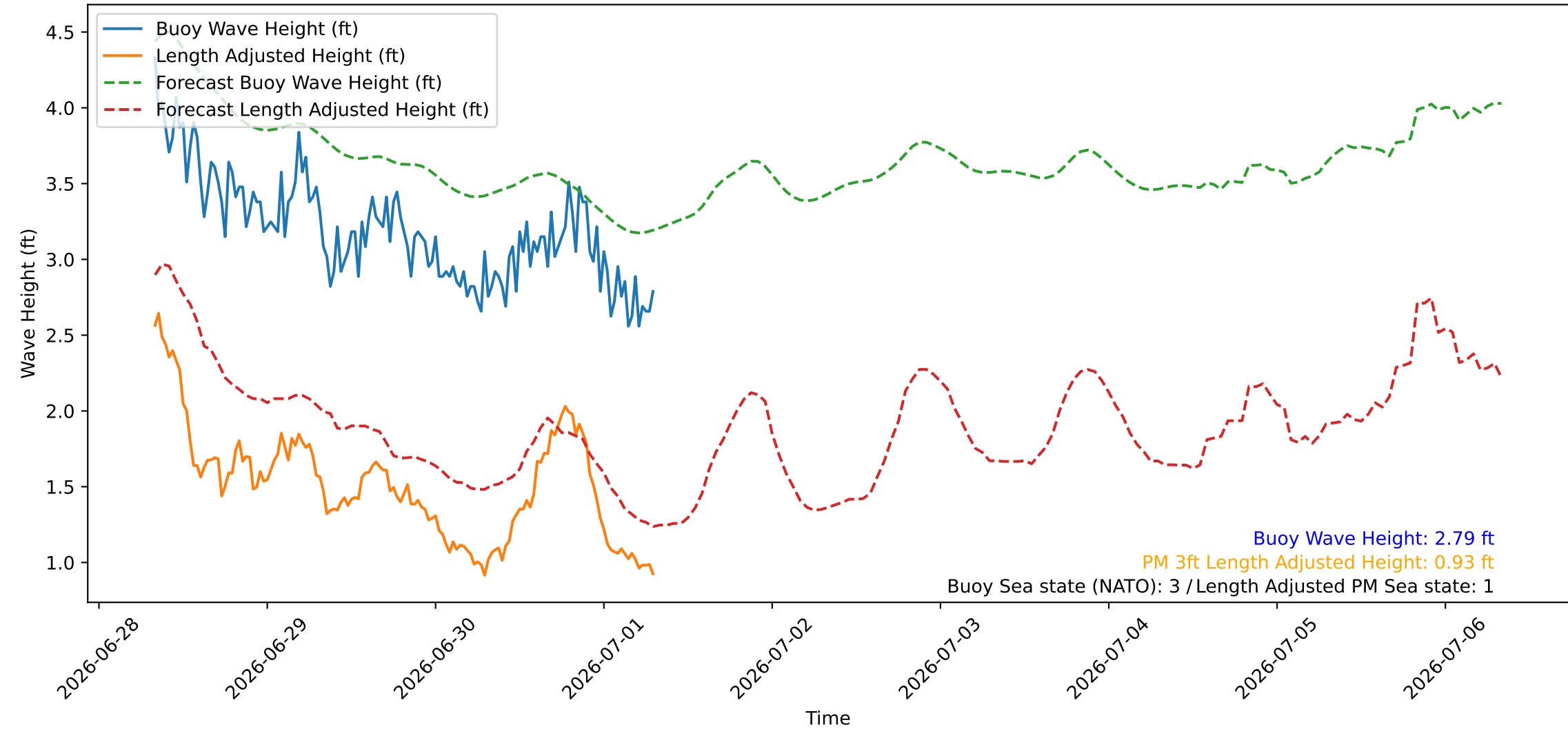
Wave Heights over Time for Green Beach at 2026-07-01 07:51:09
