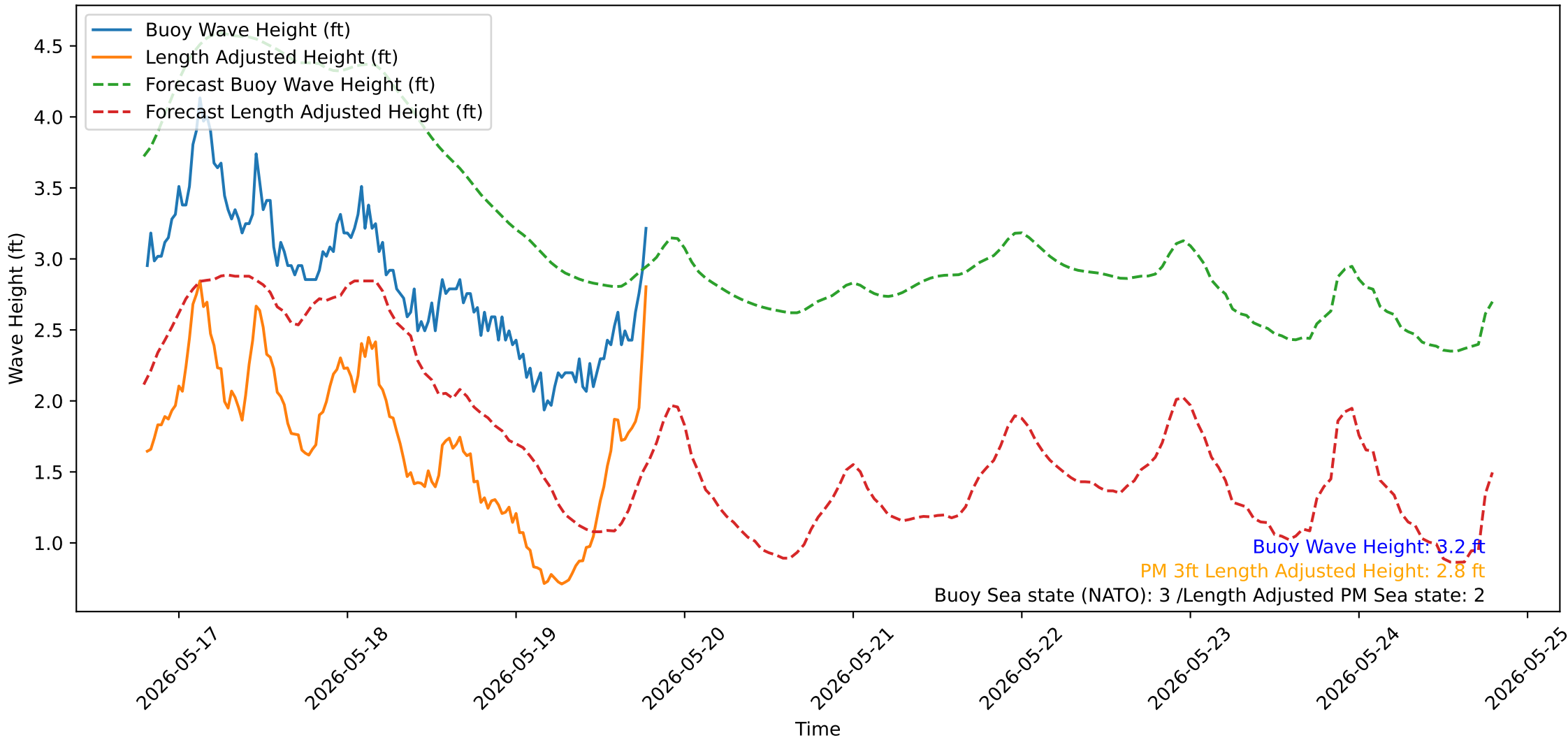
Wave Heights over Time for Red Beach at 2026-05-19 19:20:52
