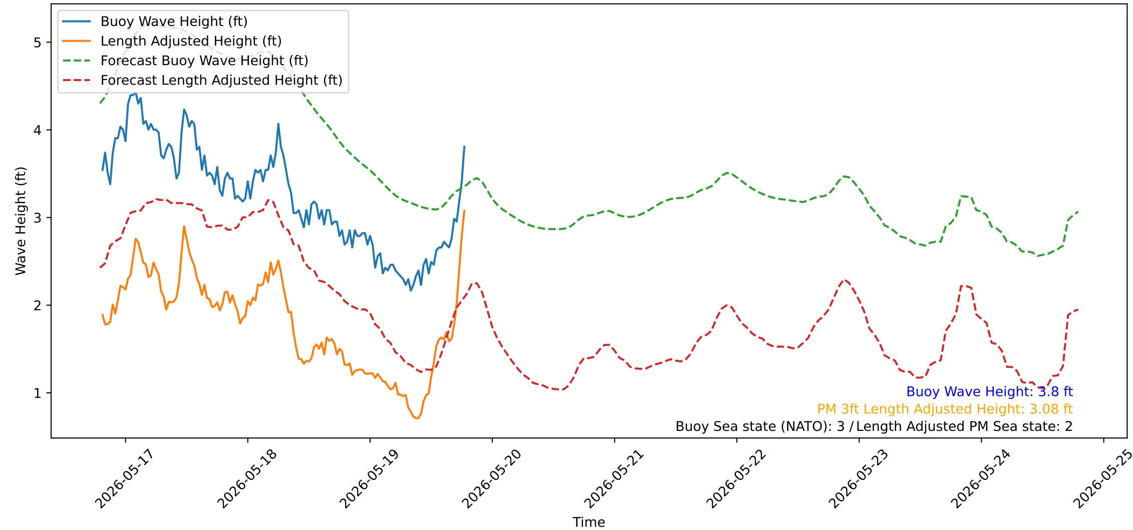
Wave Heights over Time for Green Beach at 2026-05-19 19:21:15
