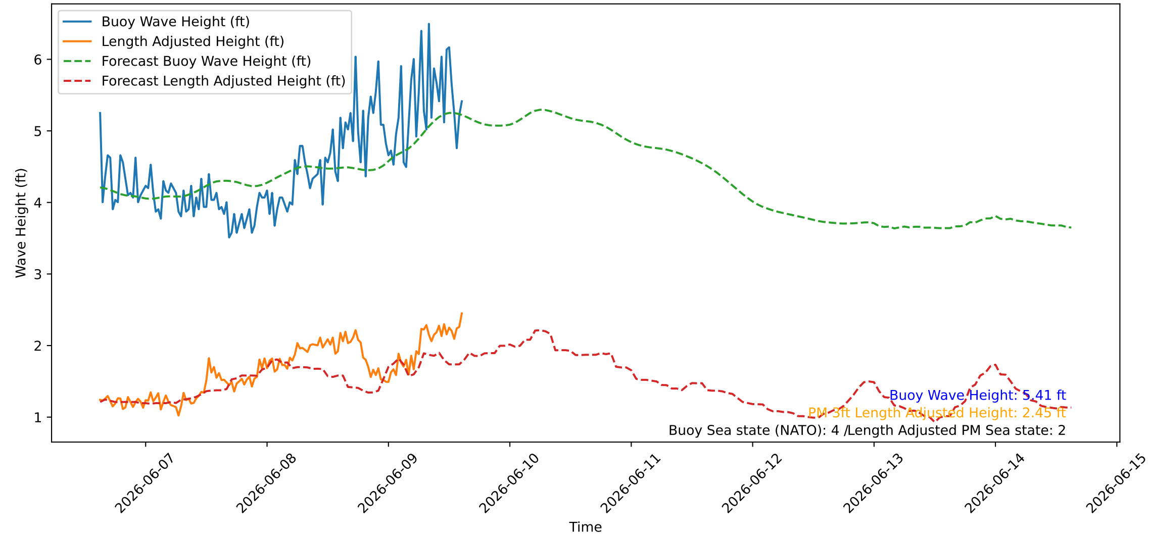
Wave Heights over Time for Oceanside Harbor at 2026-06-09 15:10:26
