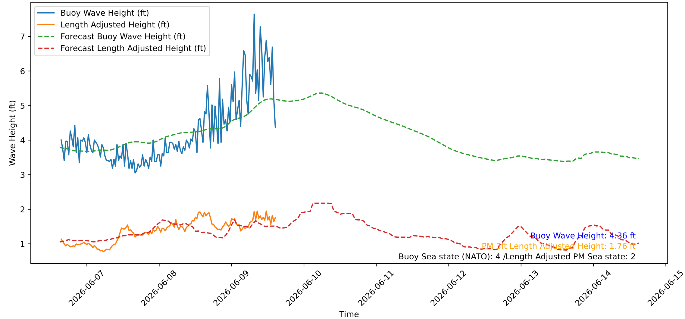
Wave Heights over Time for Red Beach at 2026-06-09 15:10:46
