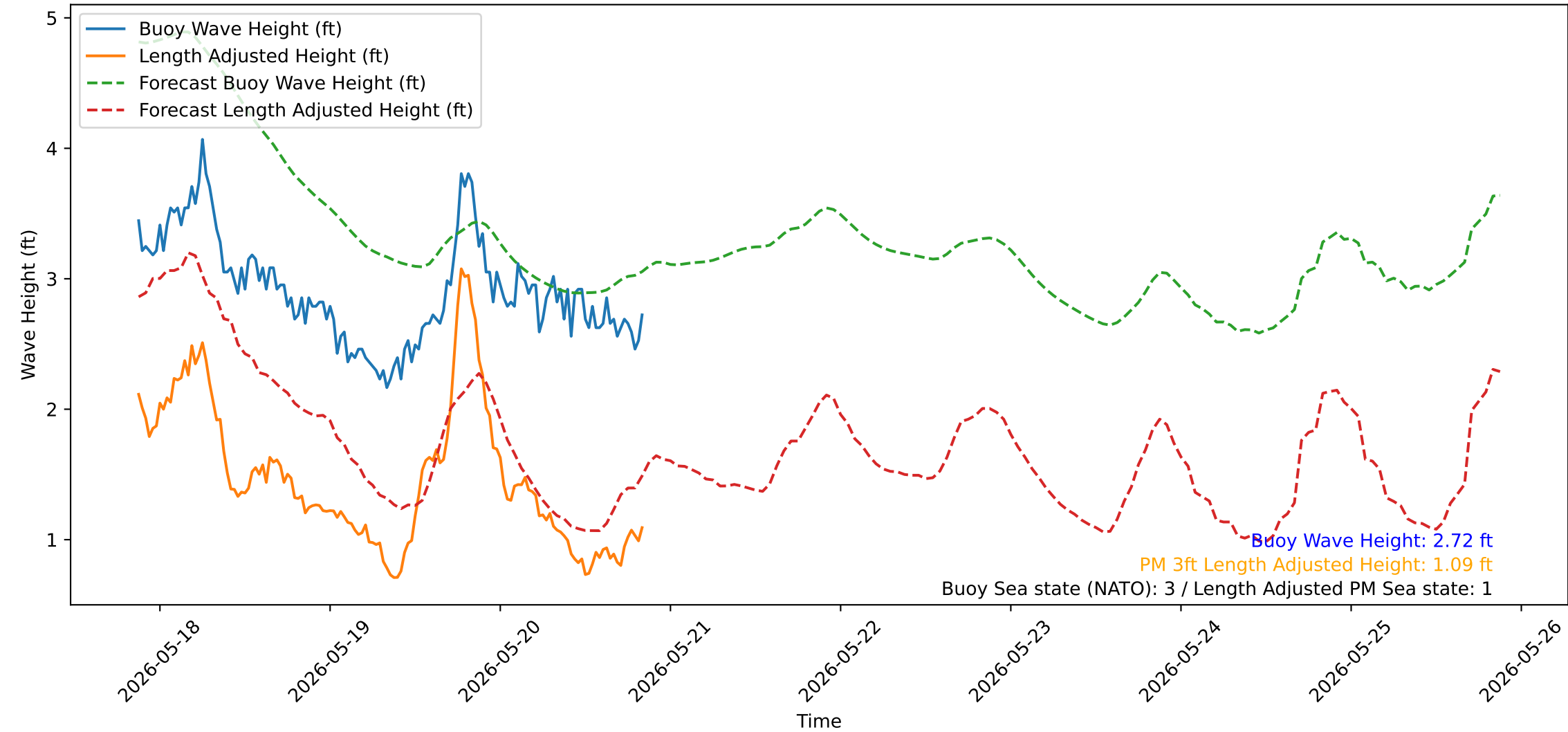
Wave Heights over Time for Green Beach at 2026-05-20 21:01:14
