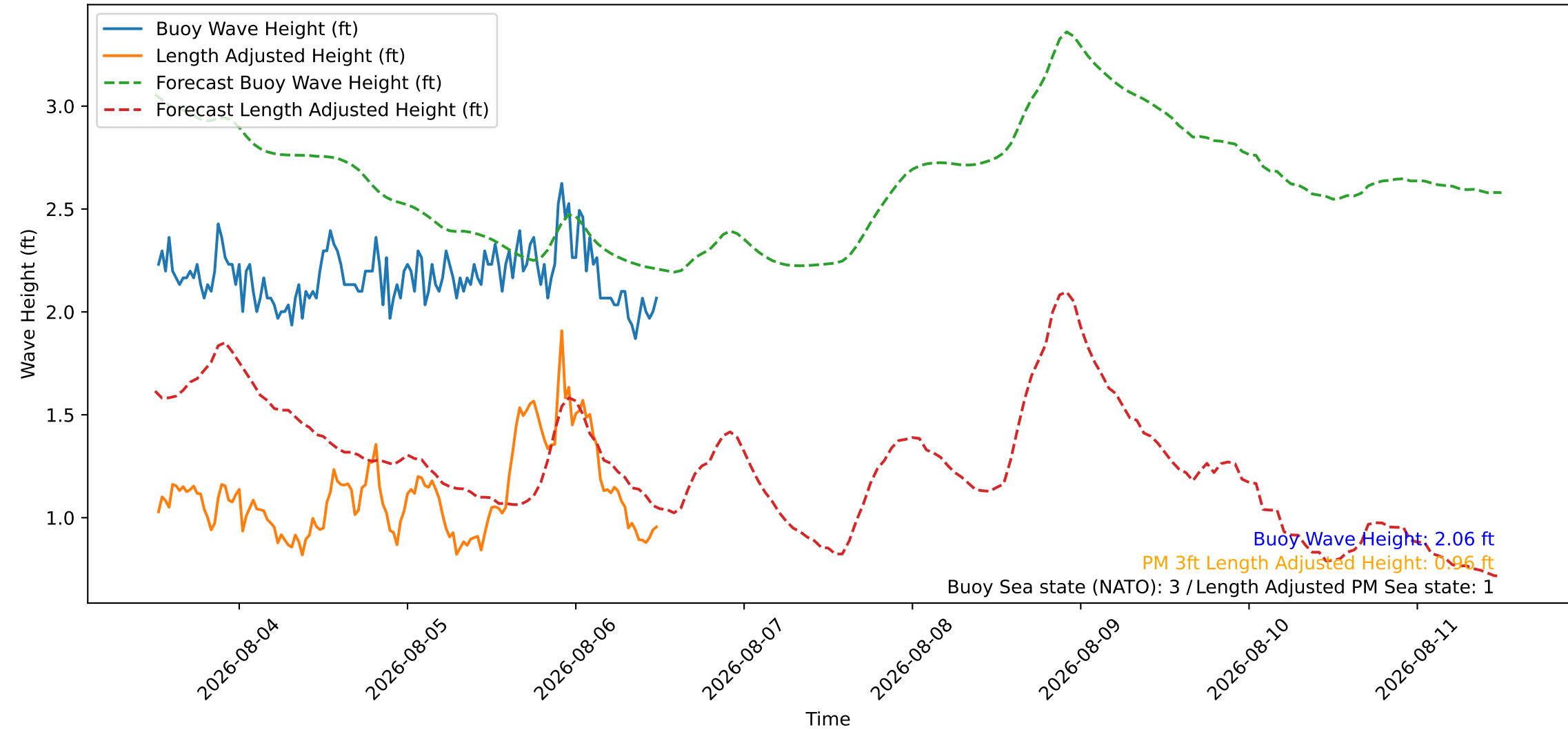
Wave Heights over Time for Green Beach at 2026-08-06 12:21:09
