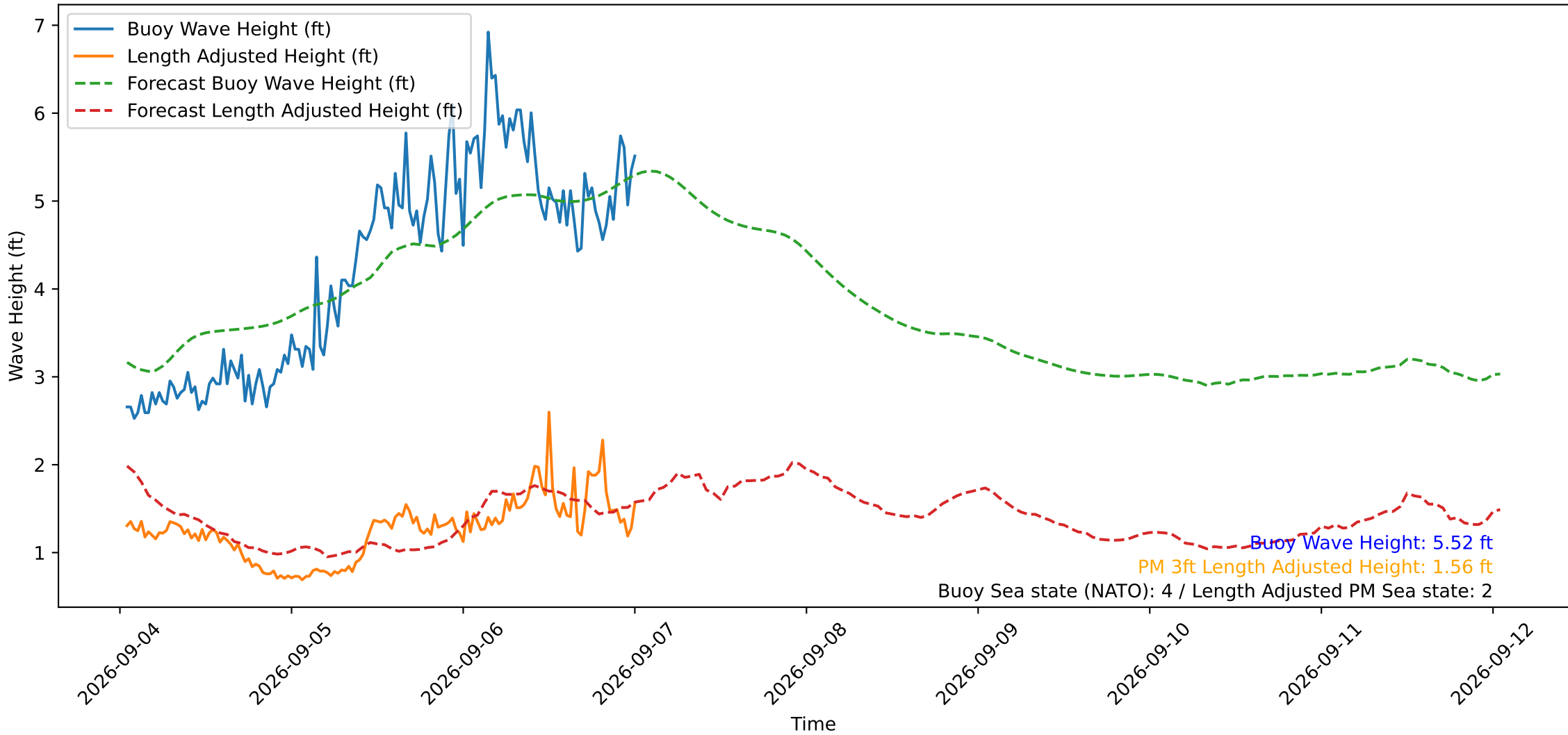
Wave Heights over Time for Red Beach at 2026-09-07 00:50:50
