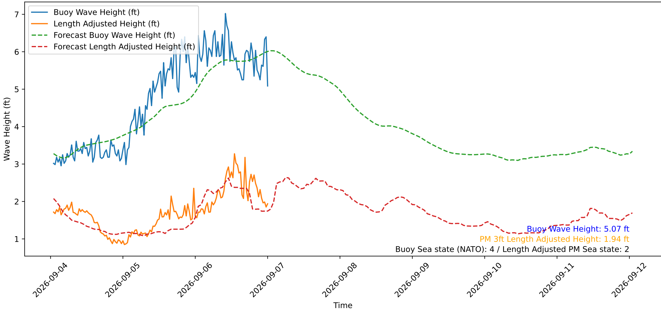
Wave Heights over Time for Oceanside Harbor at 2026-09-07 00:50:29
