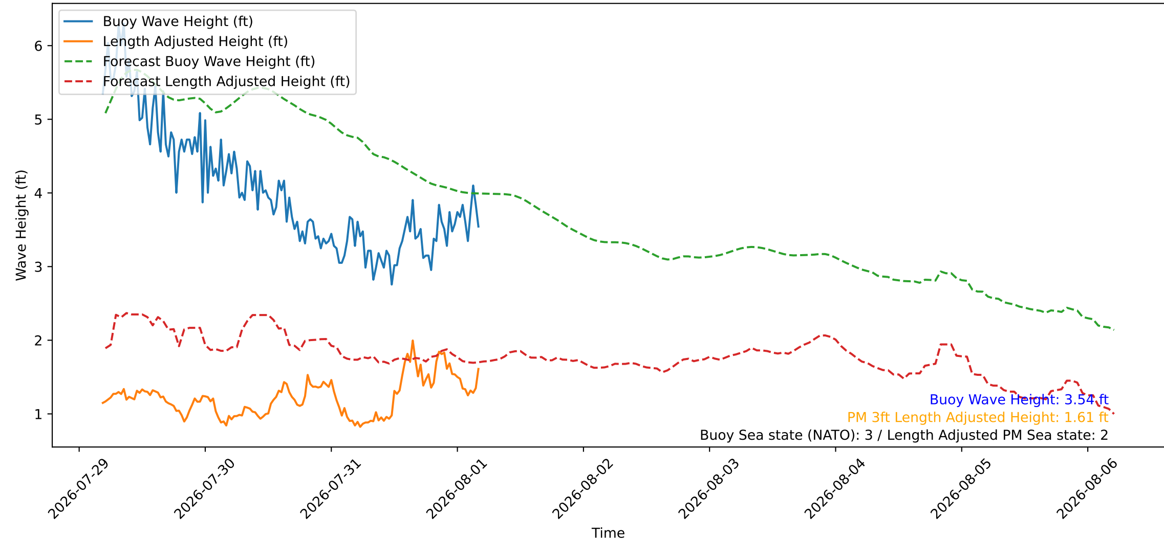
Wave Heights over Time for Green Beach at 2026-08-01 04:41:08
