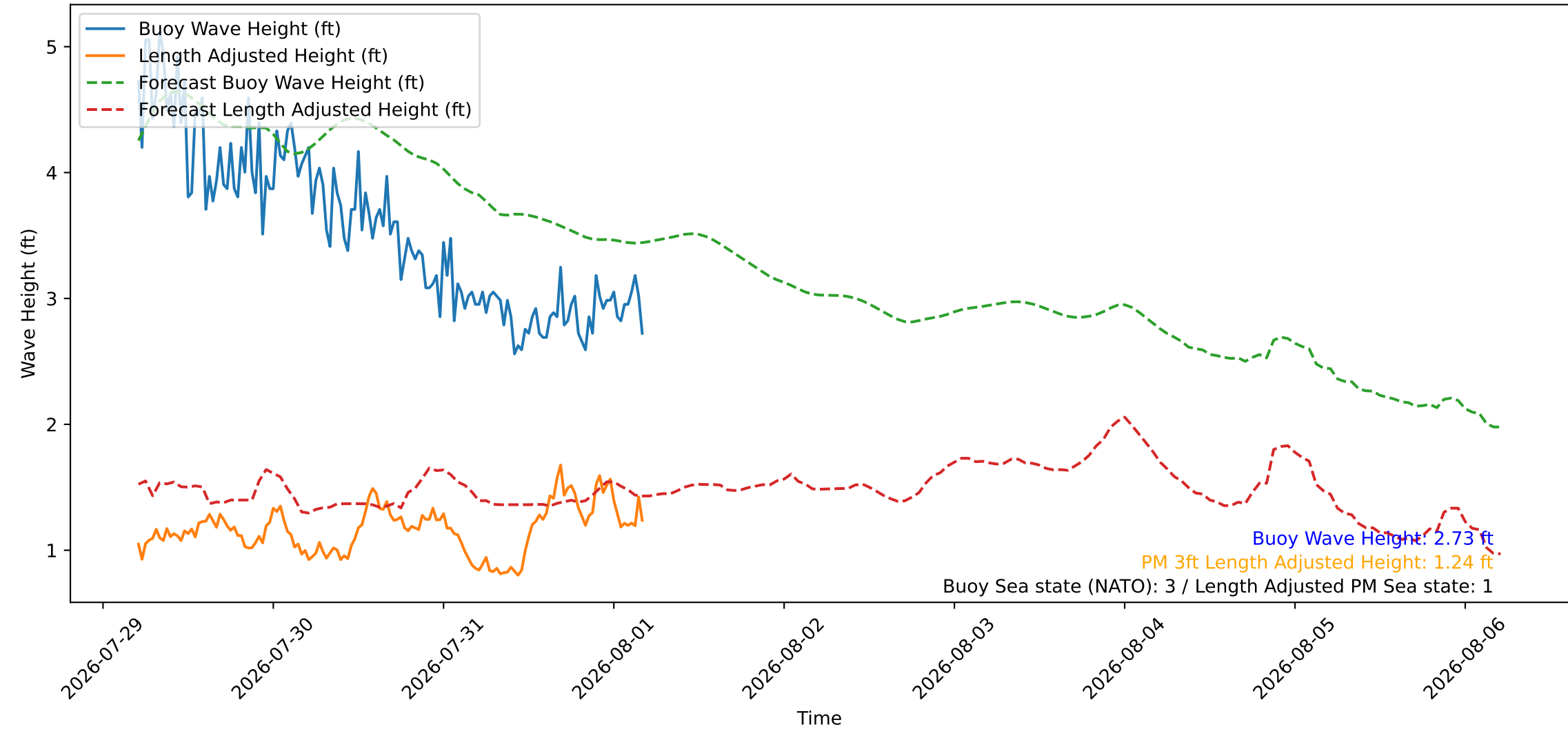
Wave Heights over Time for Red Beach at 2026-08-01 04:40:45
