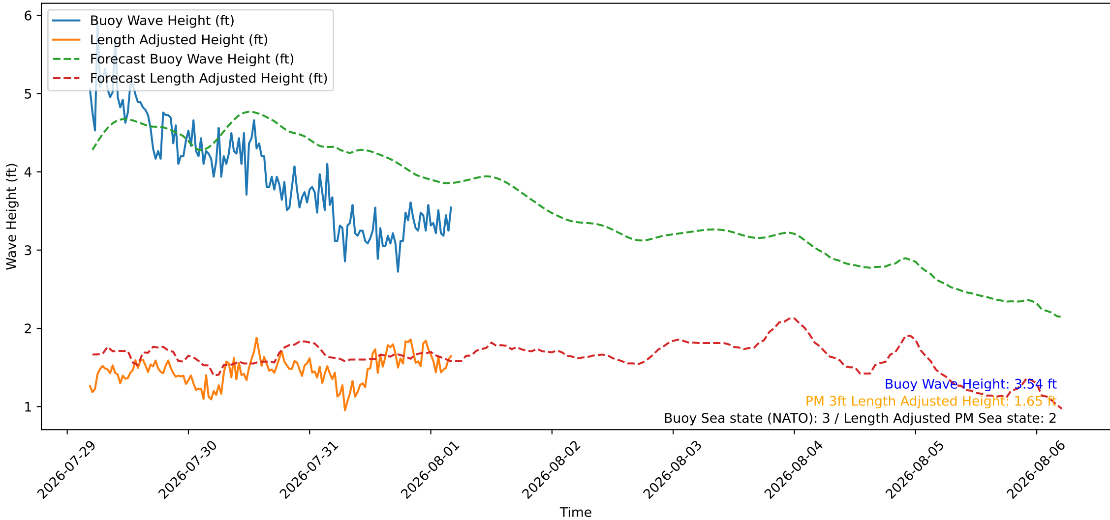
Wave Heights over Time for Oceanside Harbor at 2026-08-01 04:40:26
