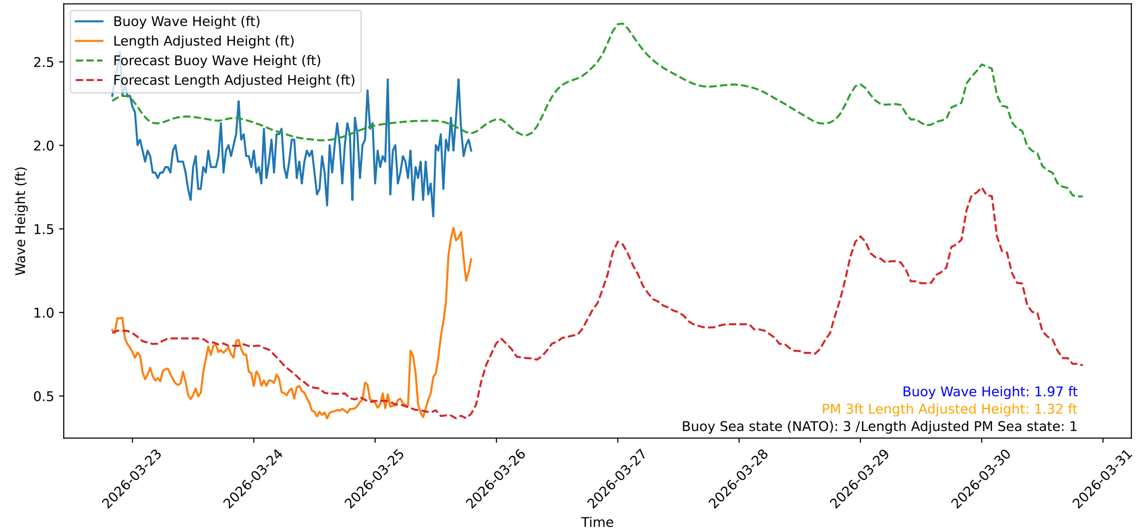
Wave Heights over Time for Red Beach at 2026-03-25 19:50:47
