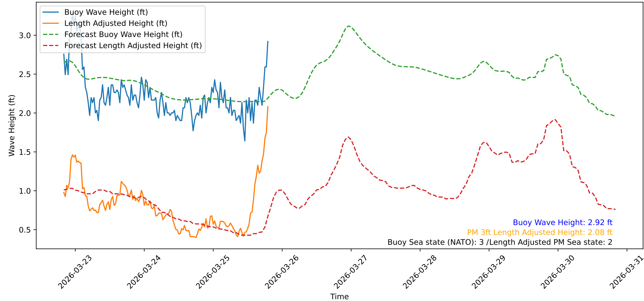
Wave Heights over Time for Green Beach at 2026-03-25 19:51:10
