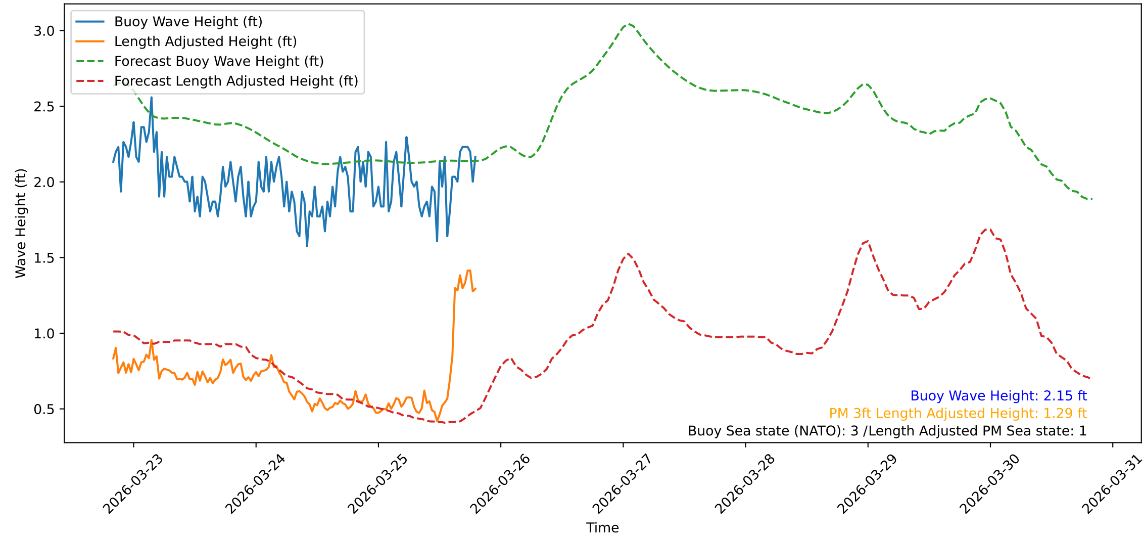
Wave Heights over Time for Oceanside Harbor at 2026-03-25 19:50:31
