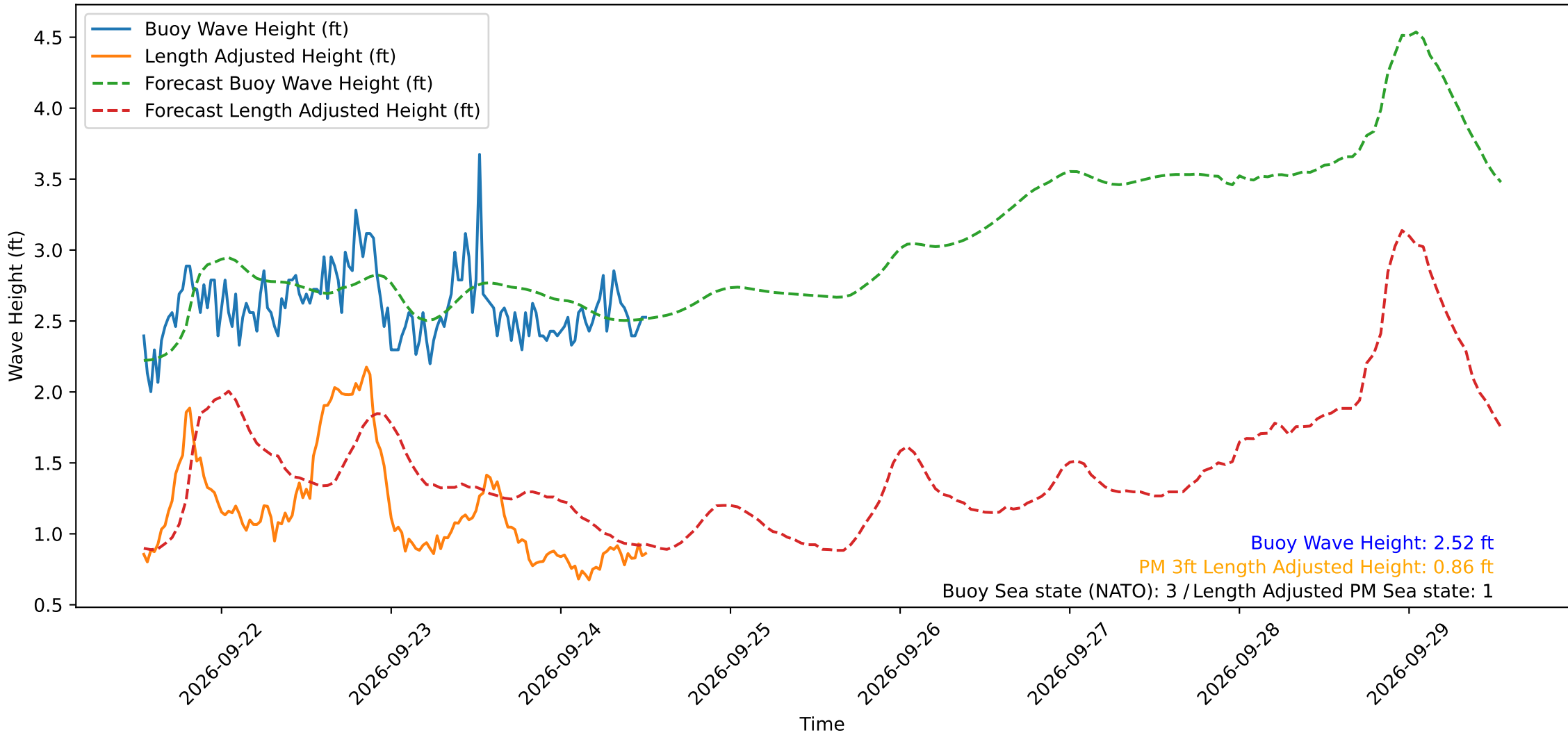
Wave Heights over Time for Red Beach at 2026-09-24 12:40:50
