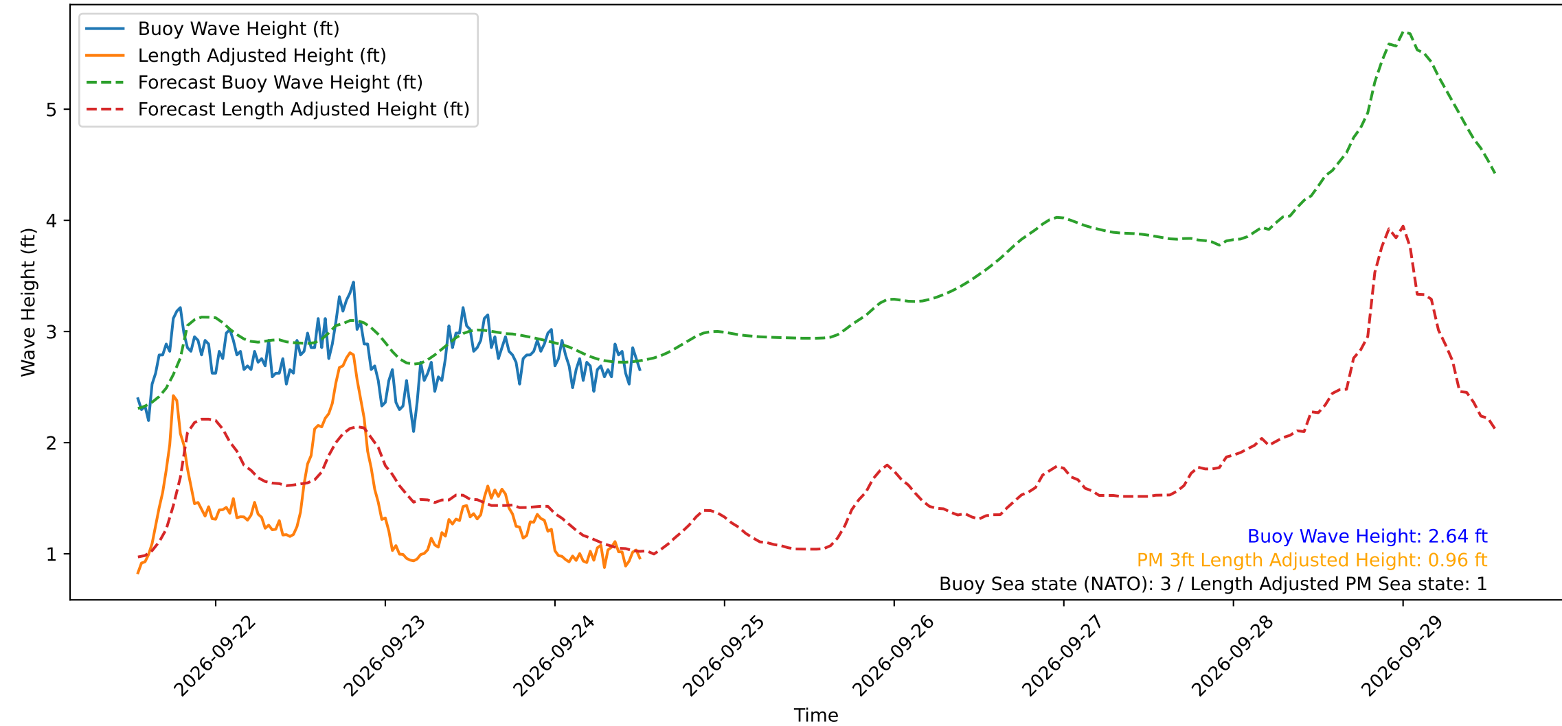
Wave Heights over Time for Green Beach at 2026-09-24 12:41:13
