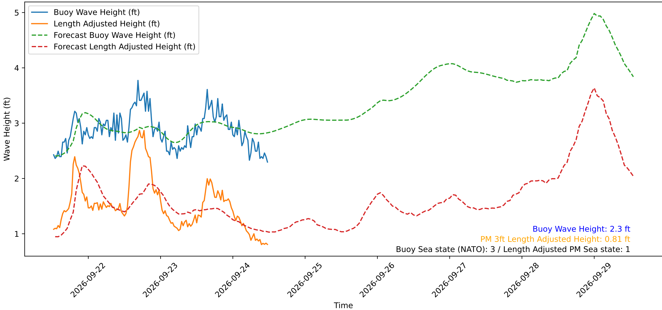
Wave Heights over Time for Oceanside Harbor at 2026-09-24 12:40:30
