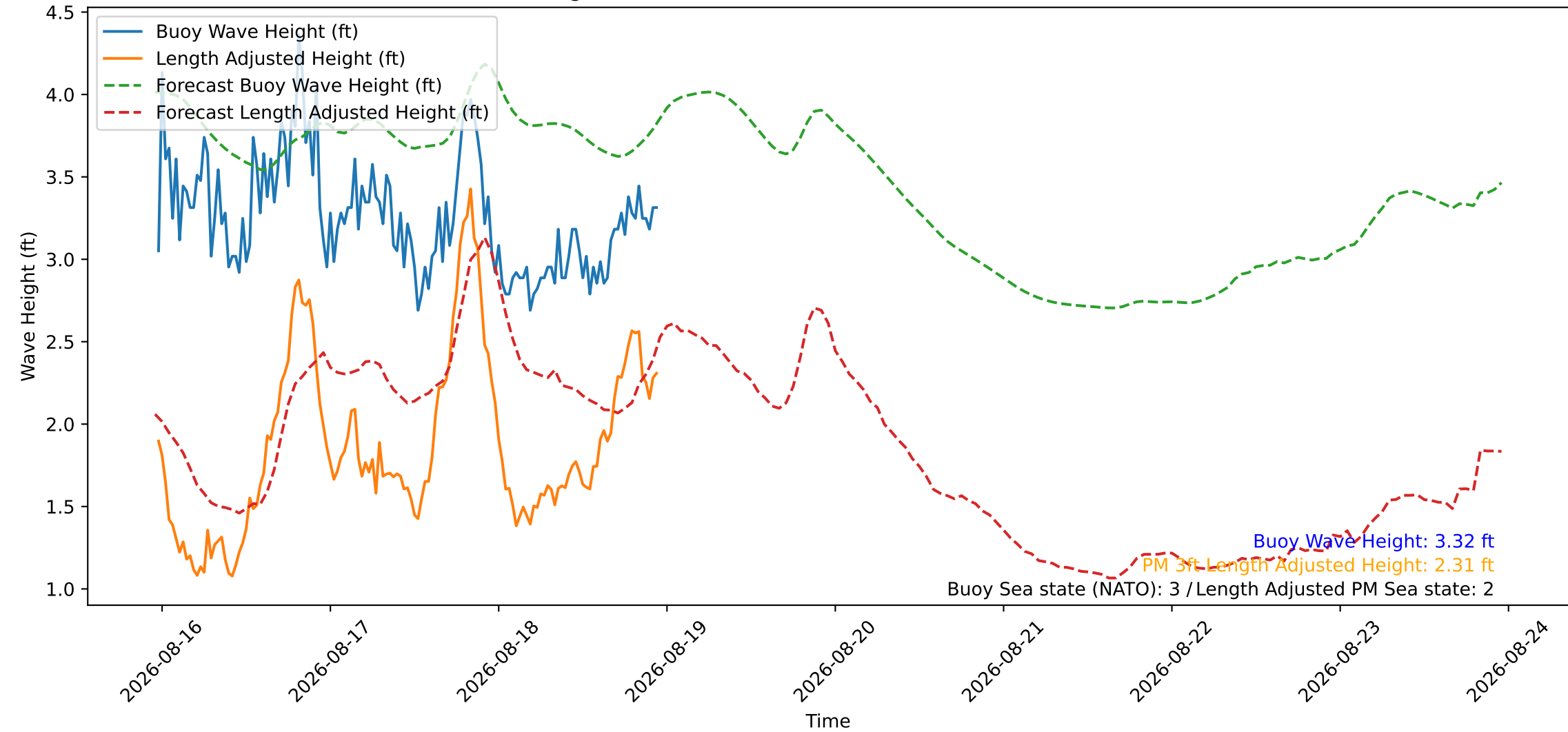
Wave Heights over Time for Green Beach at 2026-08-18 23:11:08
