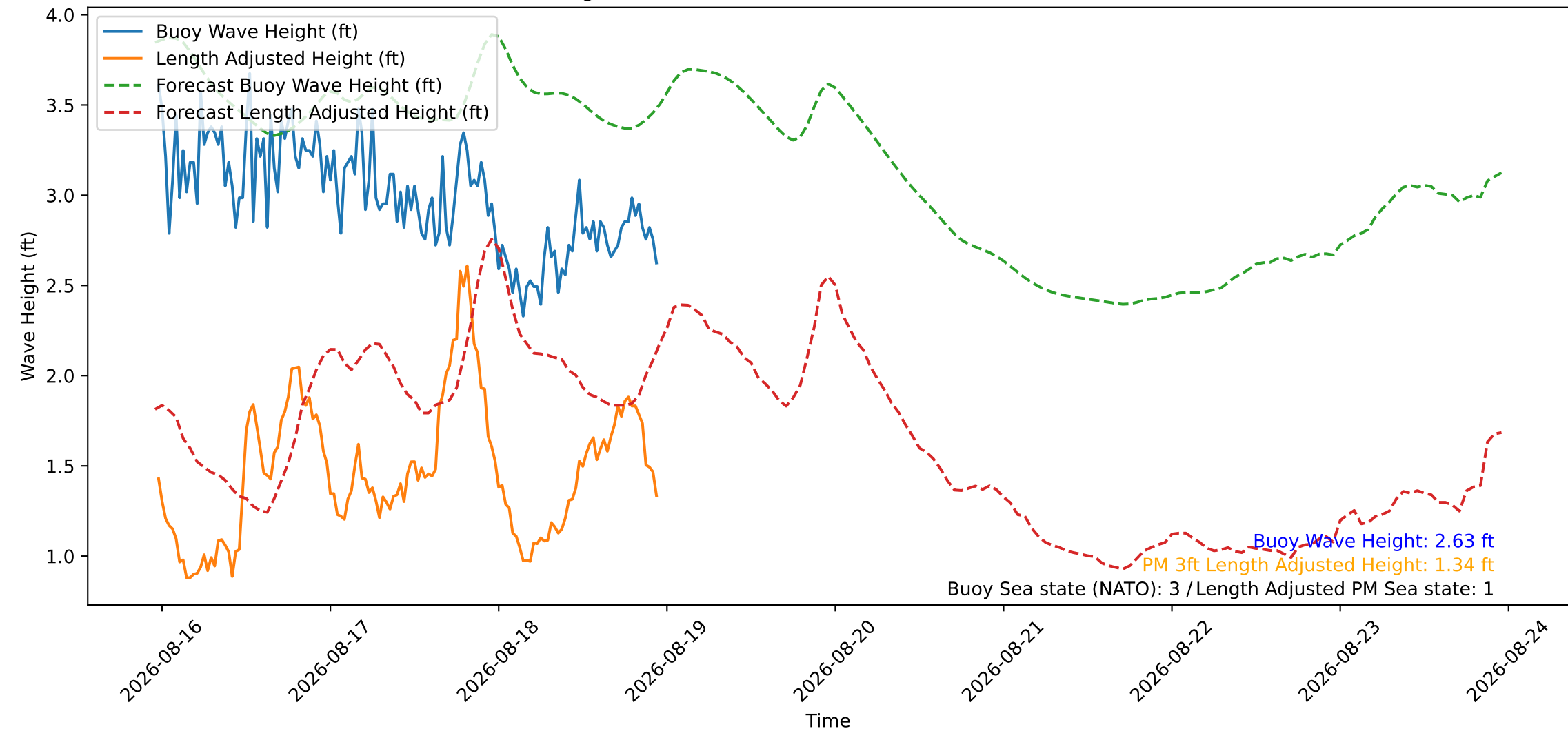
Wave Heights over Time for Red Beach at 2026-08-18 23:10:45
