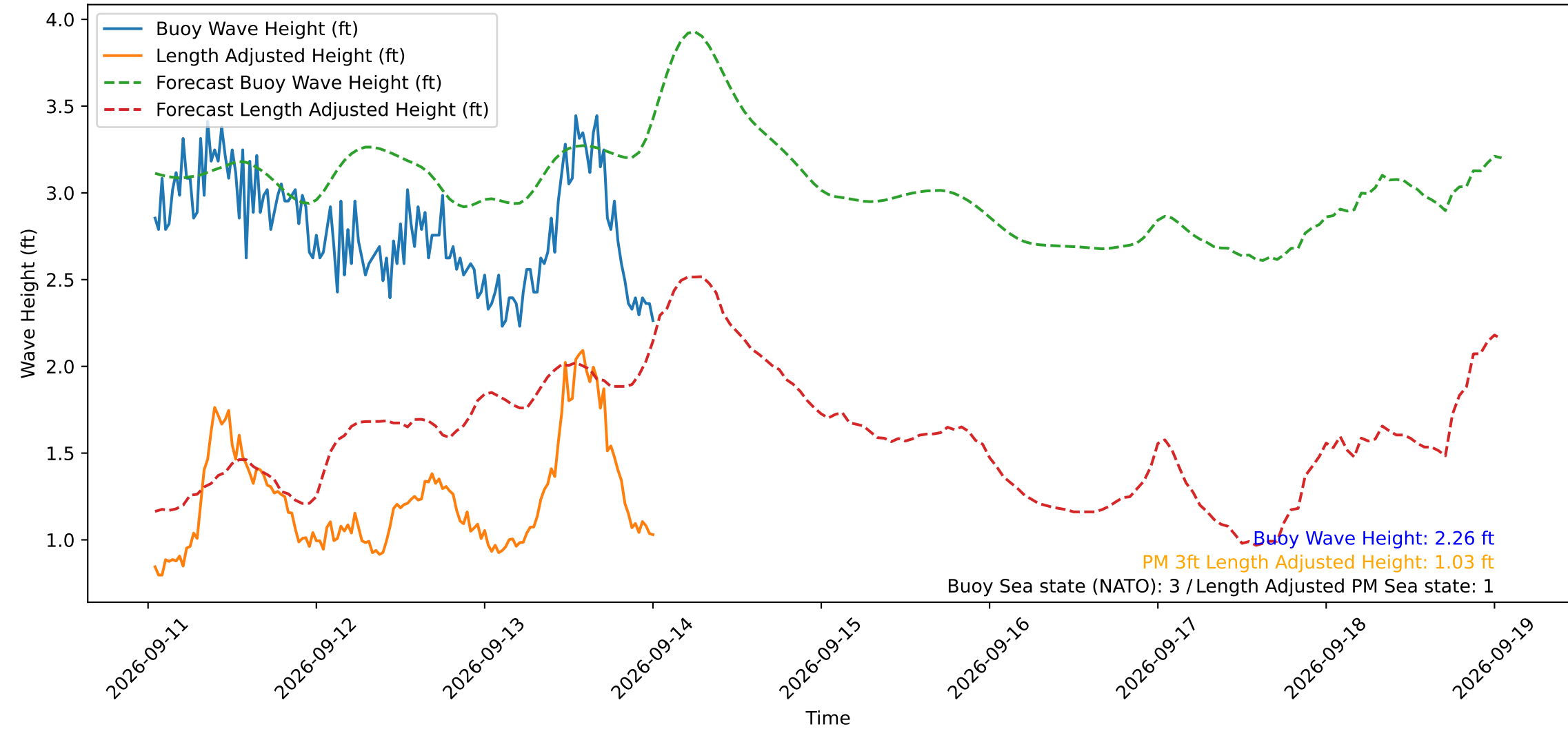
Wave Heights over Time for Red Beach at 2026-09-14 00:50:49
