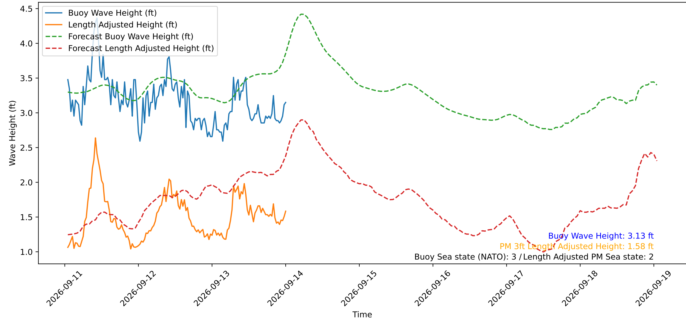
Wave Heights over Time for Oceanside Harbor at 2026-09-14 00:50:29
