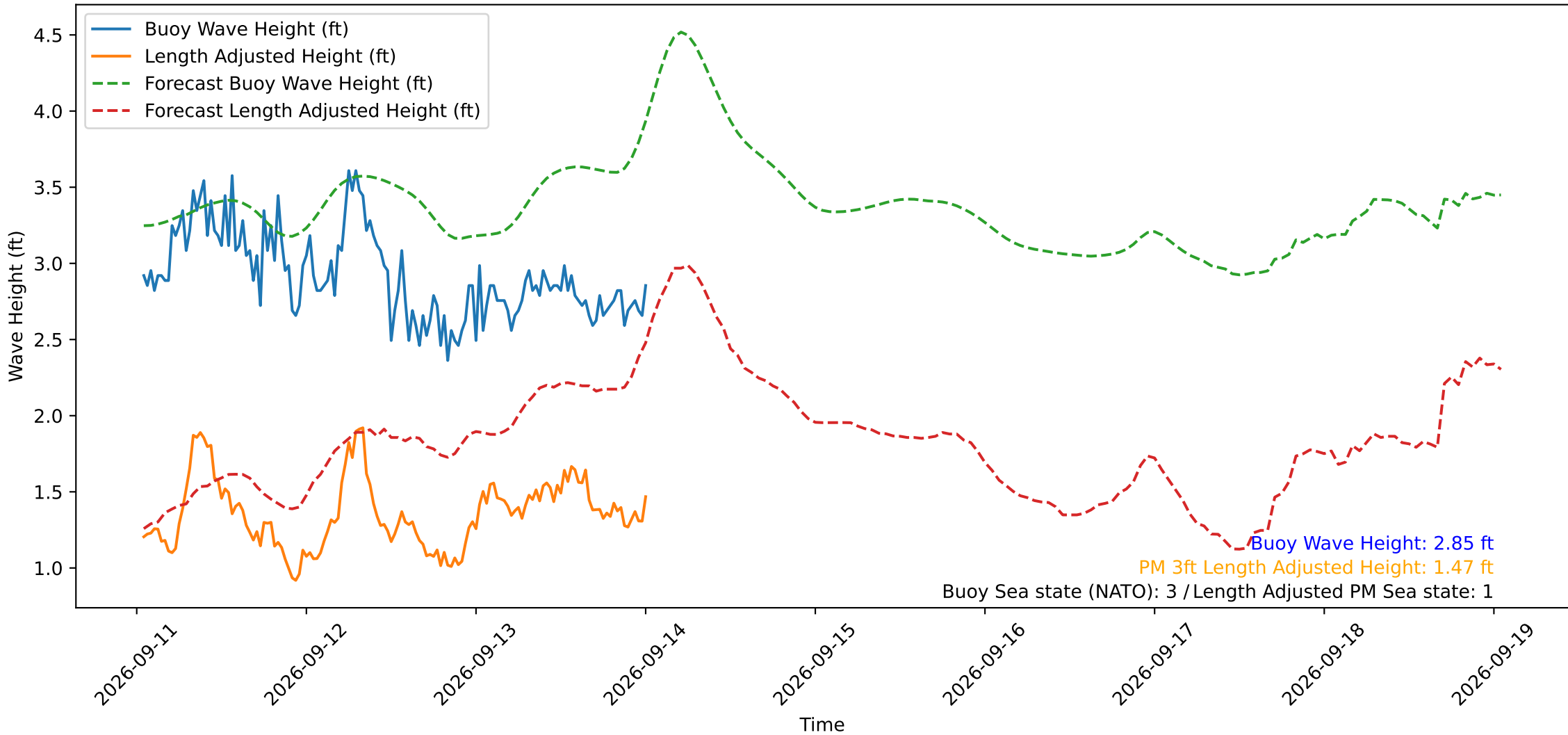
Wave Heights over Time for Green Beach at 2026-09-14 00:51:13
