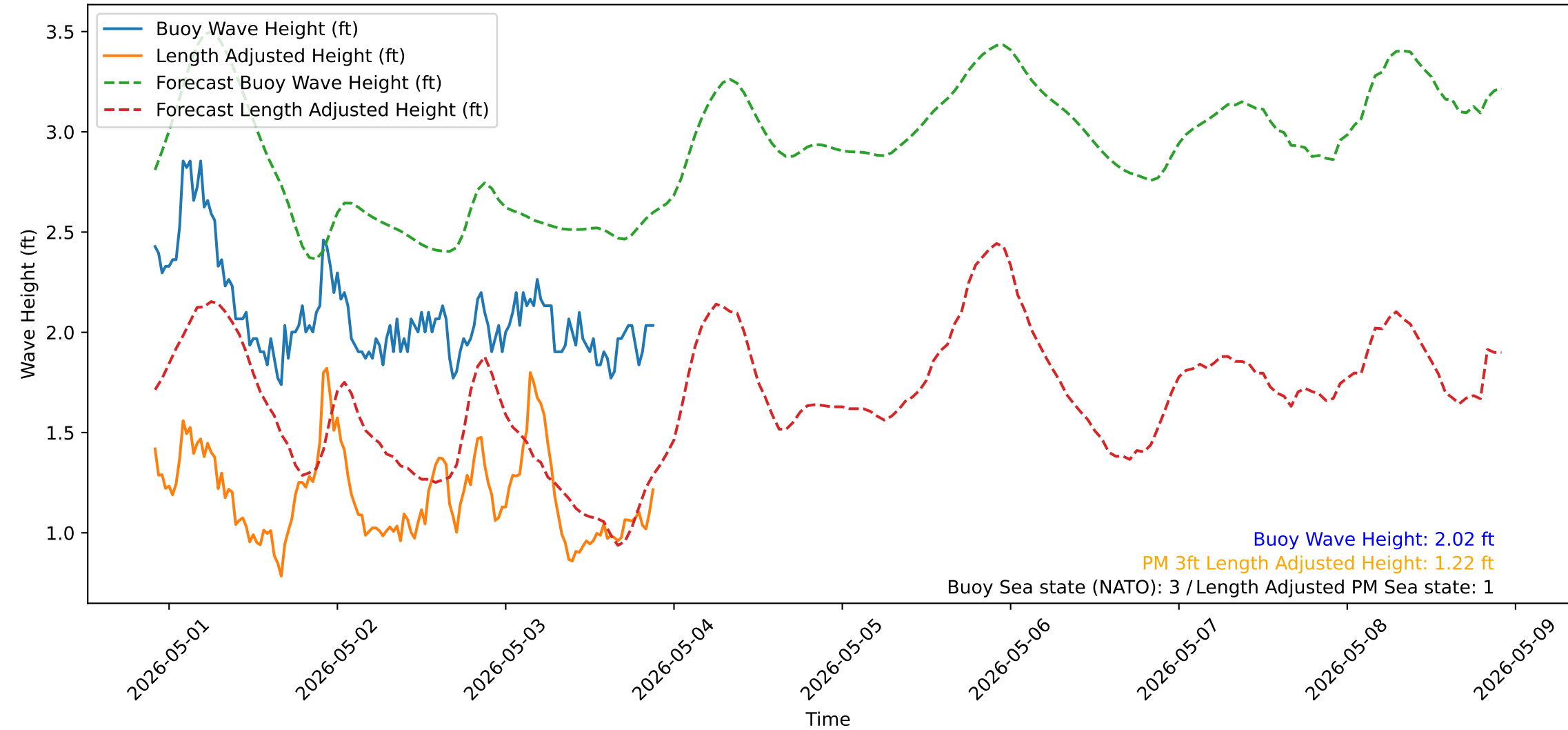
Wave Heights over Time for Green Beach at 2026-05-03 22:01:13
