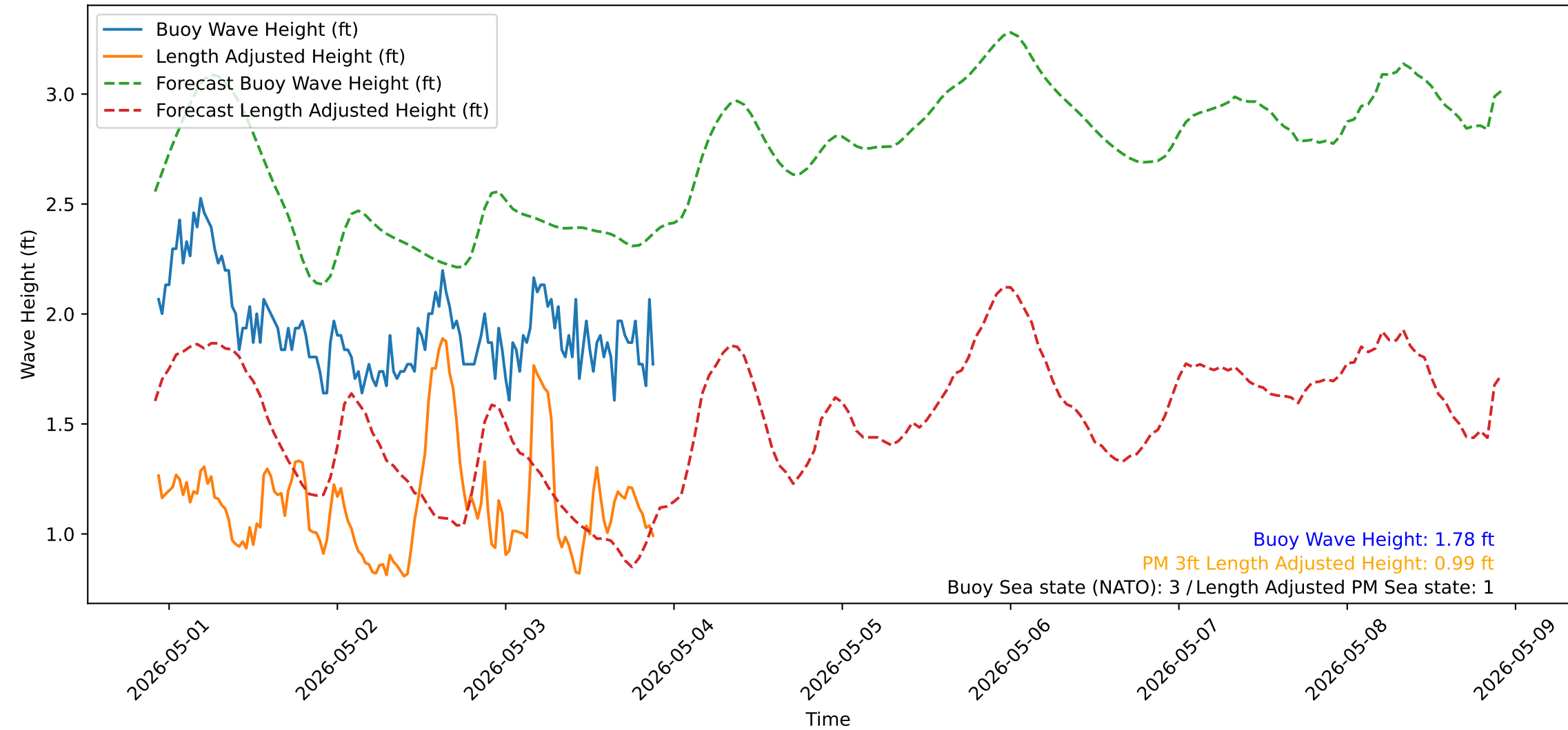
Wave Heights over Time for Red Beach at 2026-05-03 22:00:51
