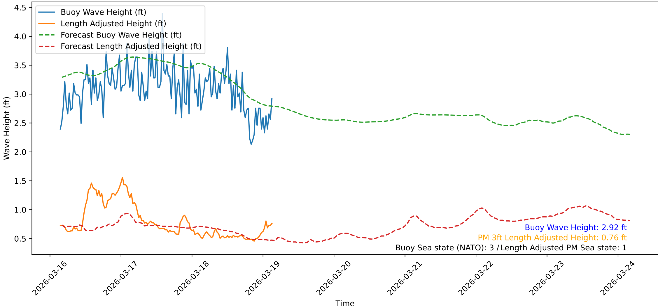
Wave Heights over Time for Oceanside Harbor at 2026-03-19 03:40:31
