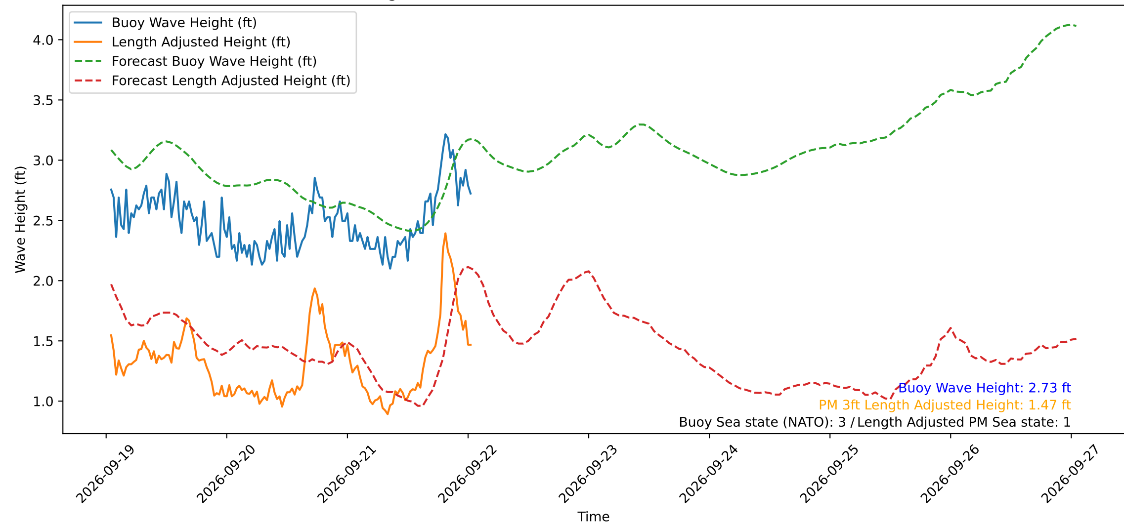
Wave Heights over Time for Oceanside Harbor at 2026-09-22 01:10:30
