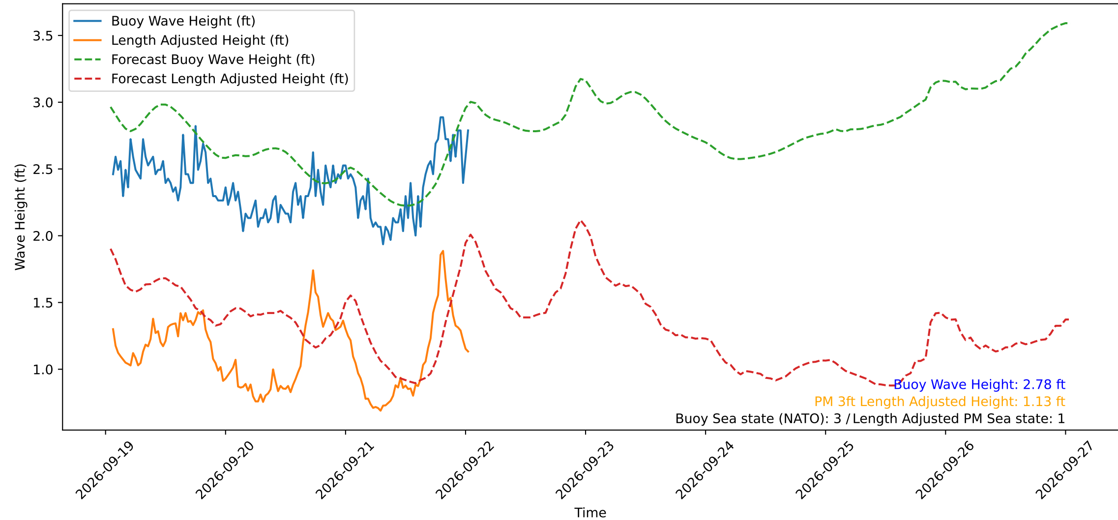
Wave Heights over Time for Red Beach at 2026-09-22 01:10:50
