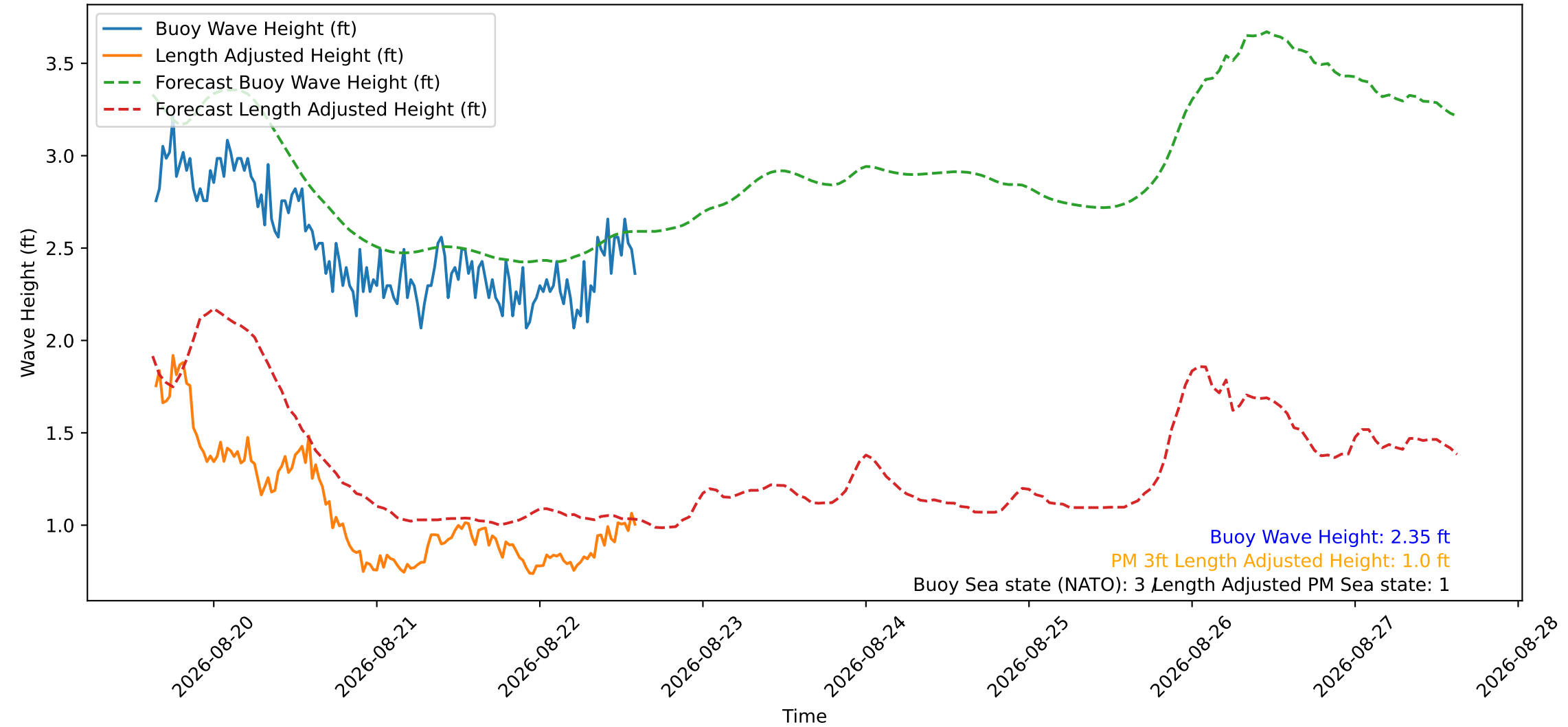
Wave Heights over Time for Red Beach at 2026-08-22 15:00:49
