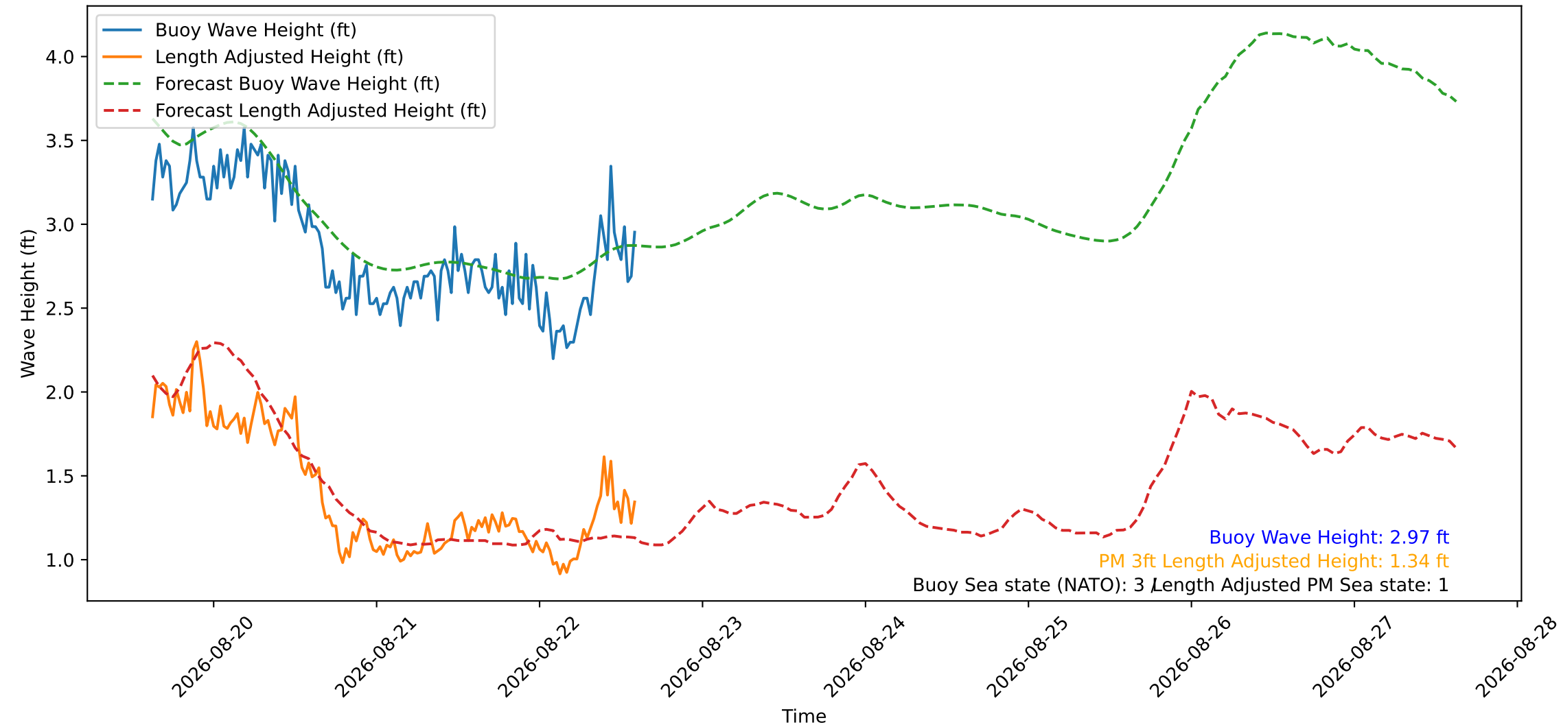
Wave Heights over Time for Oceanside Harbor at 2026-08-22 15:00:29
