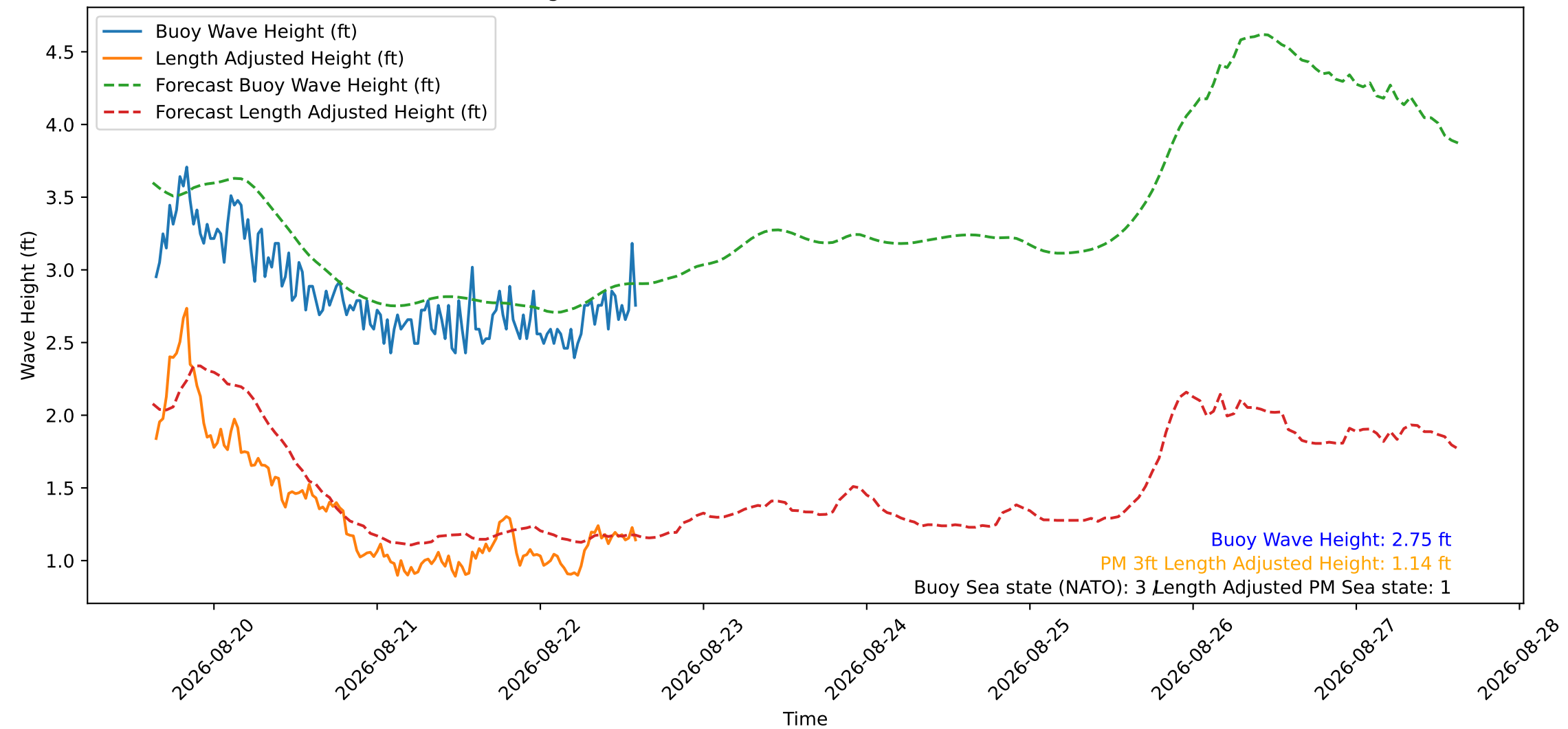
Wave Heights over Time for Green Beach at 2026-08-22 15:01:11
