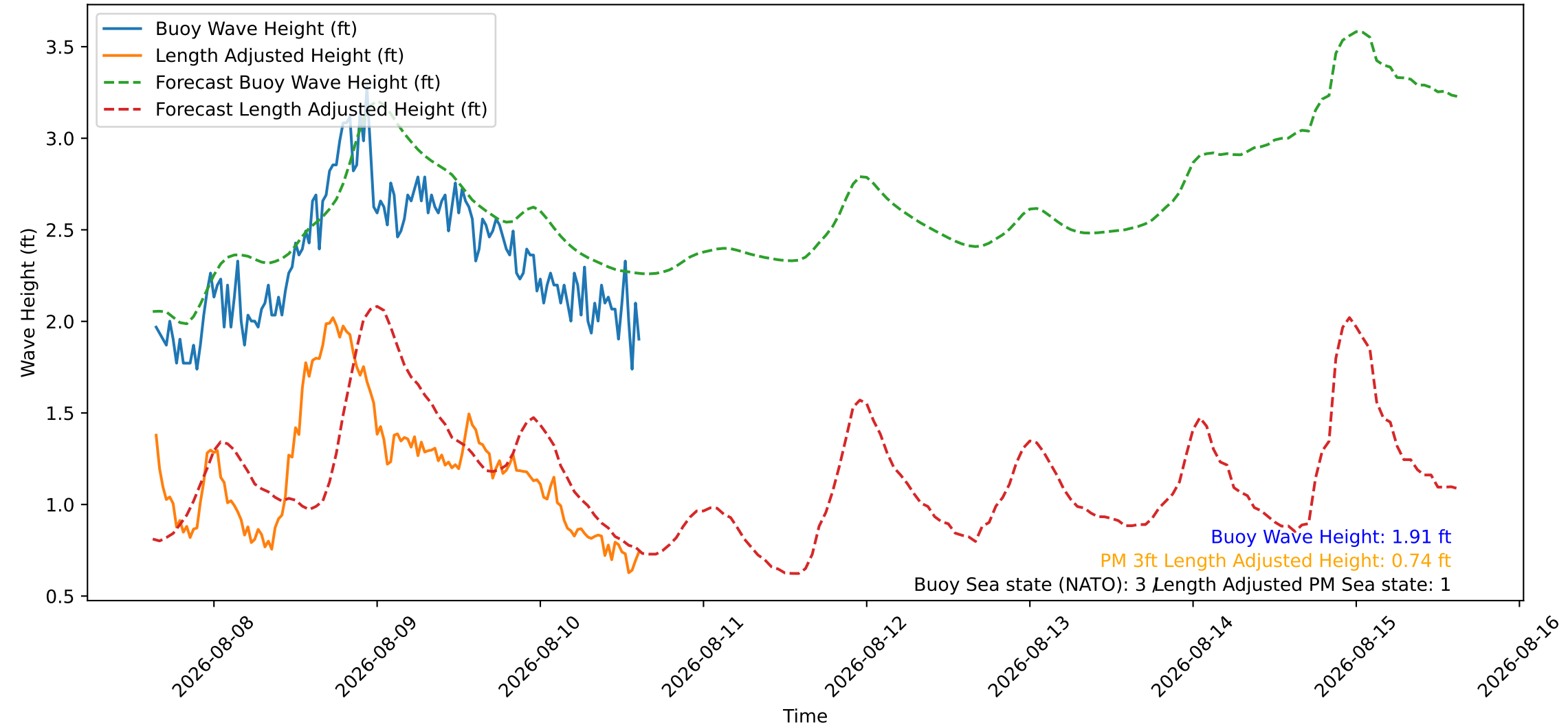
Wave Heights over Time for Red Beach at 2026-08-10 15:10:46
