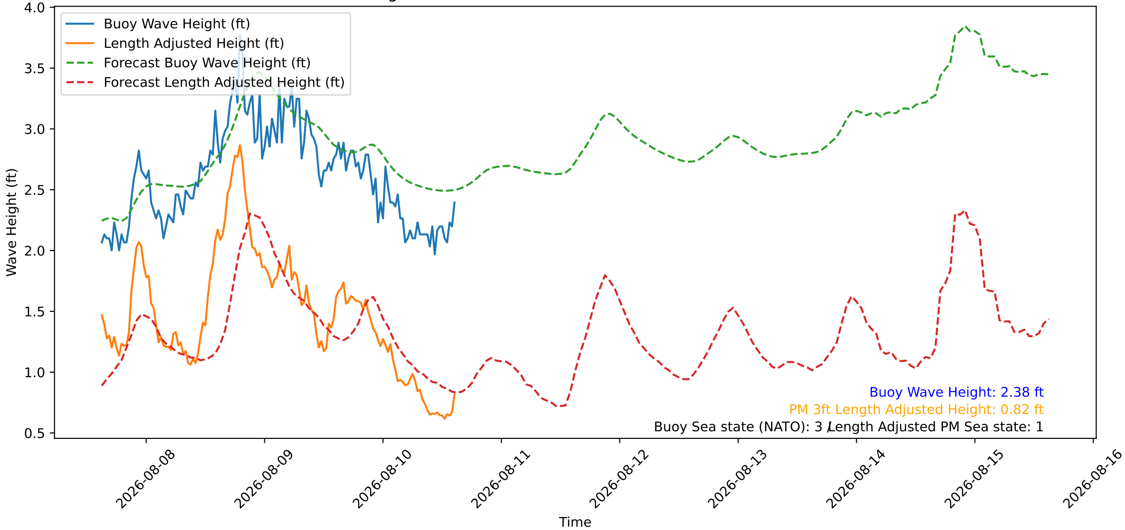
Wave Heights over Time for Green Beach at 2026-08-10 15:11:10
