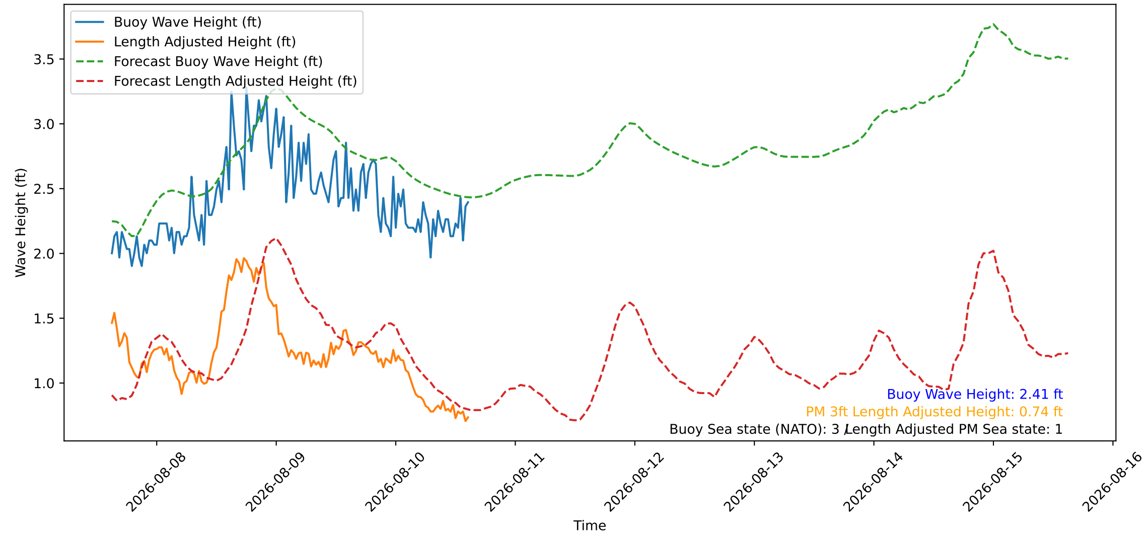
Wave Heights over Time for Oceanside Harbor at 2026-08-10 15:10:27
