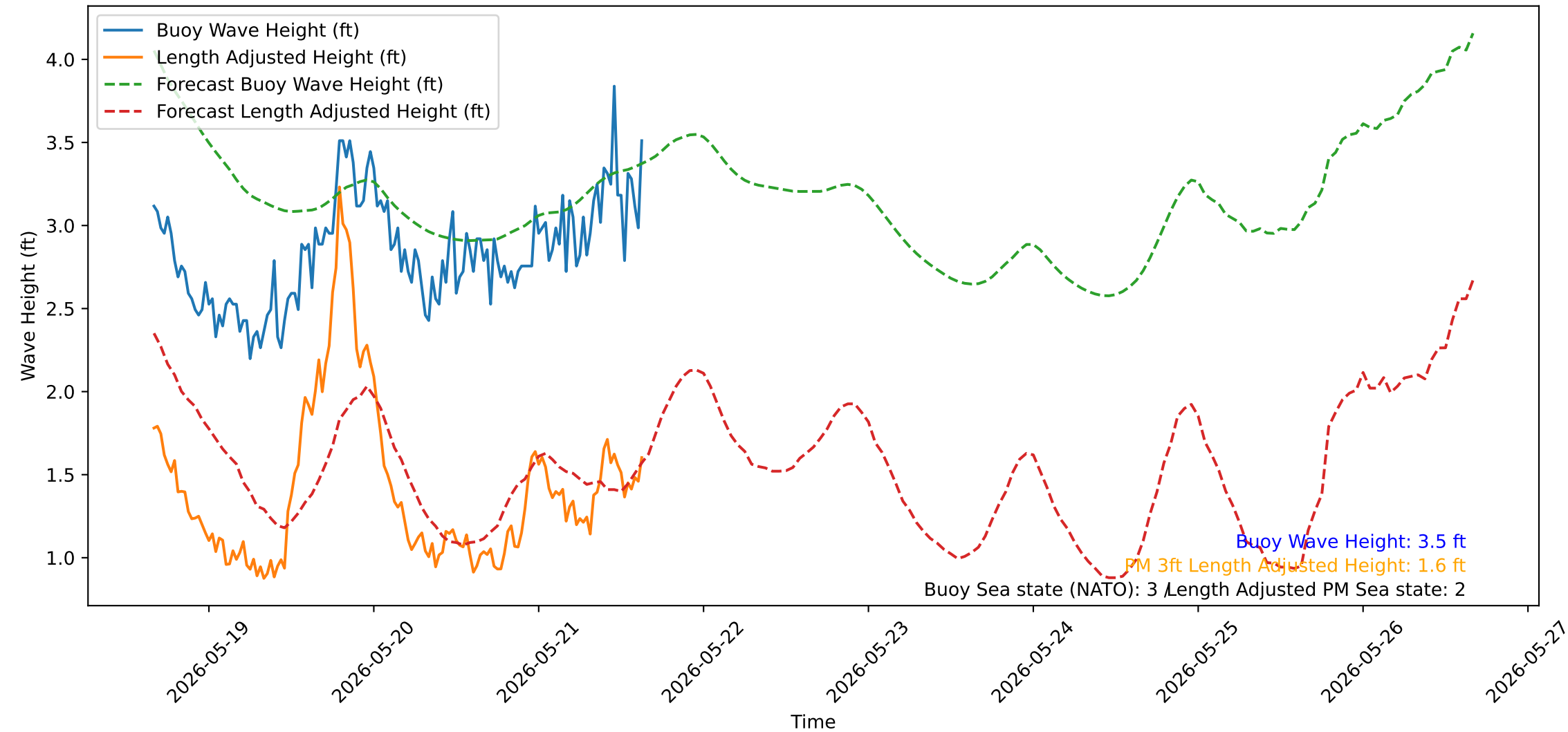
Wave Heights over Time for Oceanside Harbor at 2026-05-21 15:50:32
