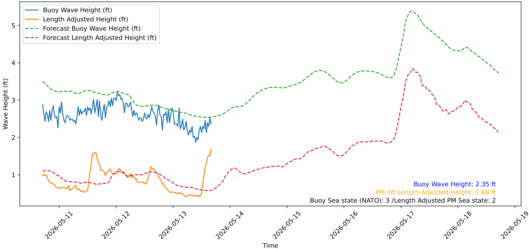
Wave Heights over Time for Red Beach at 2026-05-13 16:40:51
