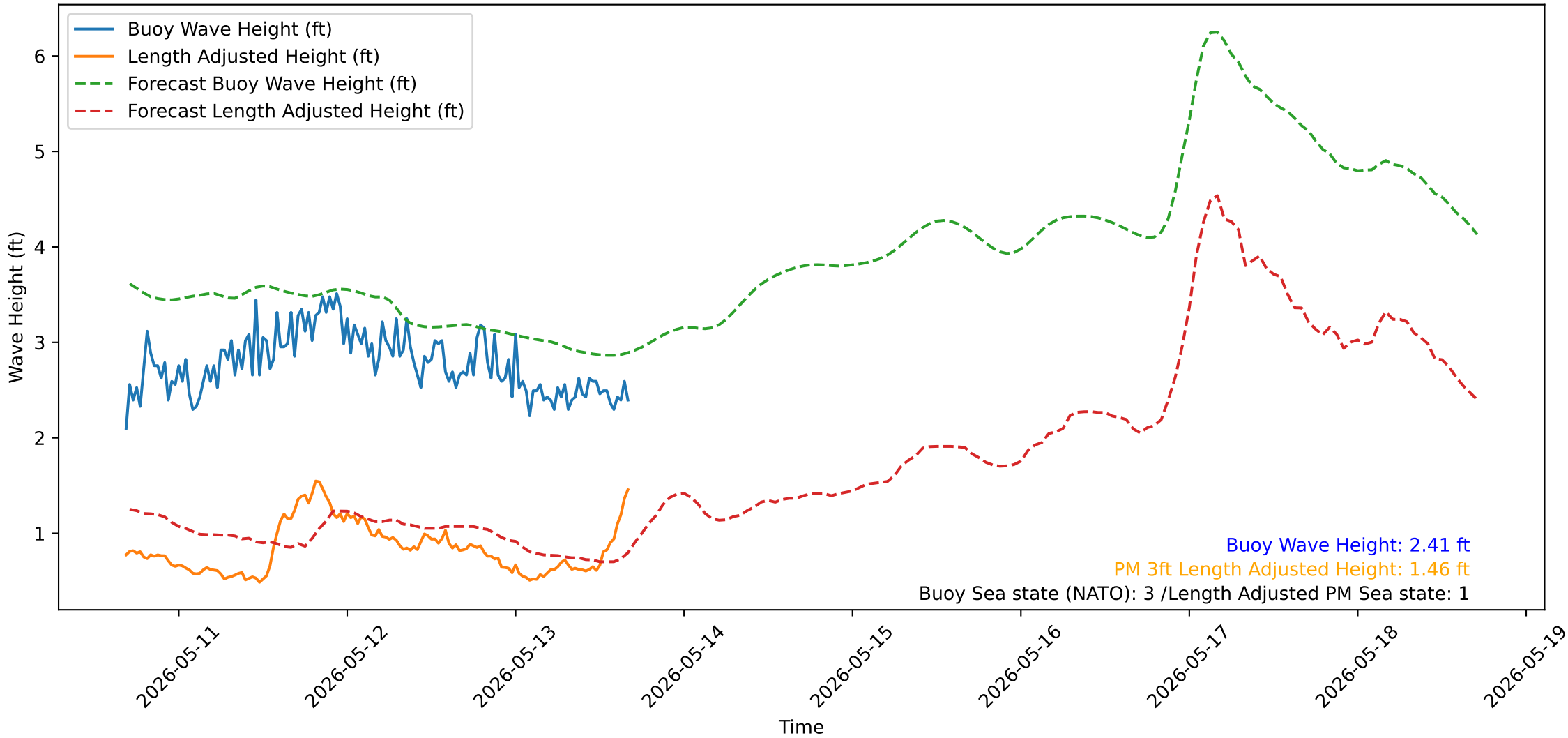
Wave Heights over Time for Green Beach at 2026-05-13 16:41:13
