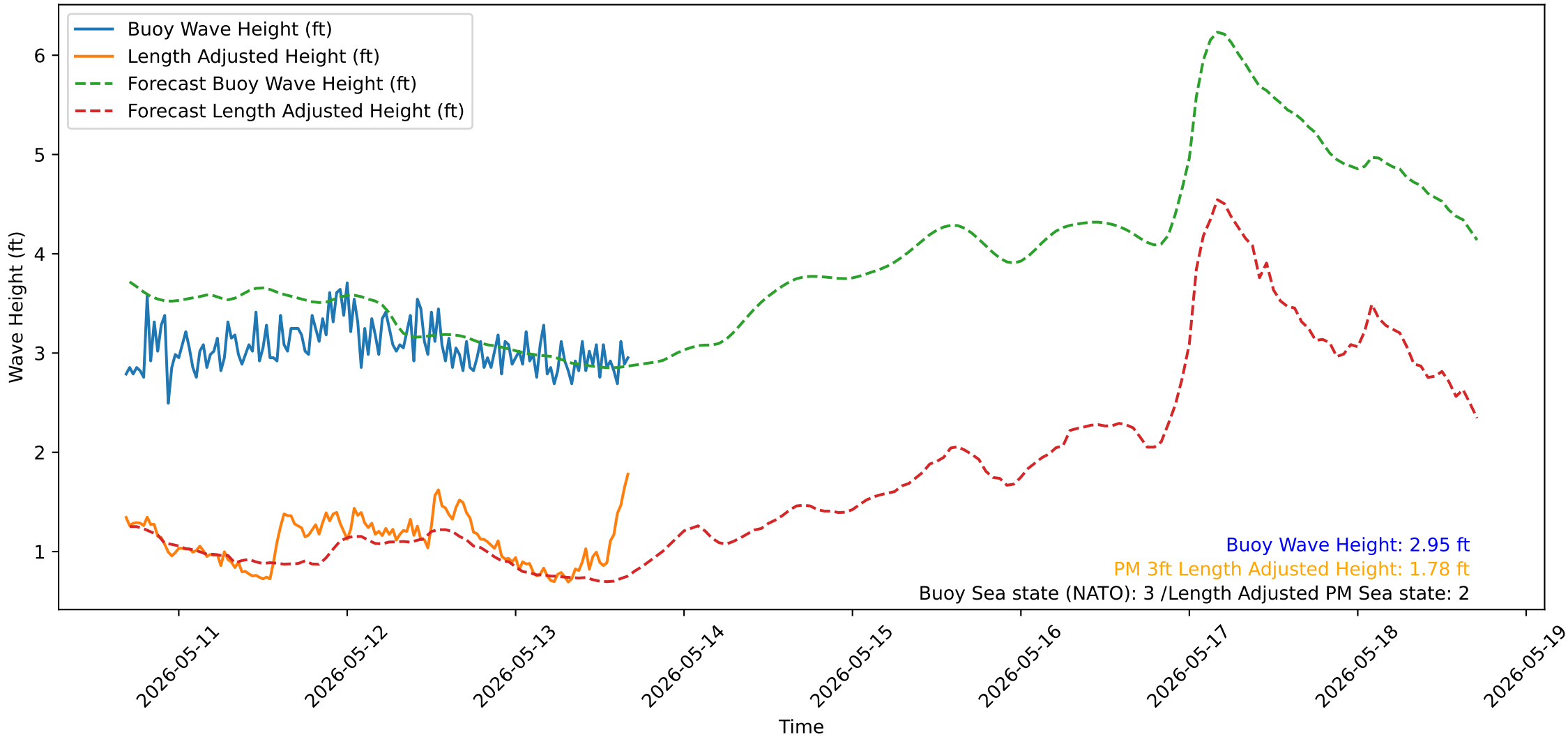
Wave Heights over Time for Oceanside Harbor at 2026-05-13 16:40:31
