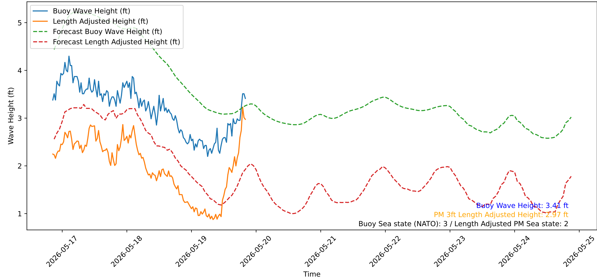
Wave Heights over Time for Oceanside Harbor at 2026-05-19 20:30:31
