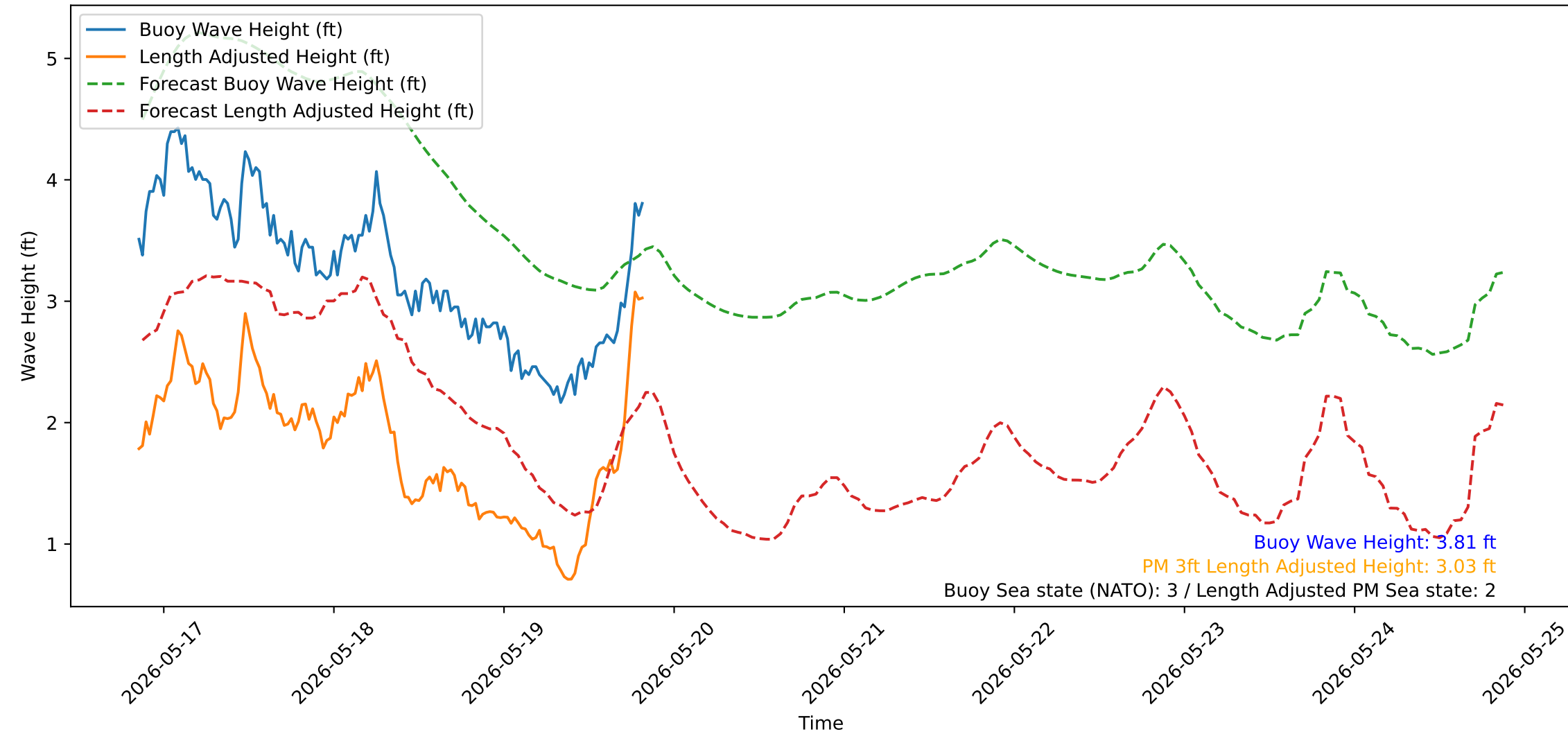
Wave Heights over Time for Green Beach at 2026-05-19 20:31:13
