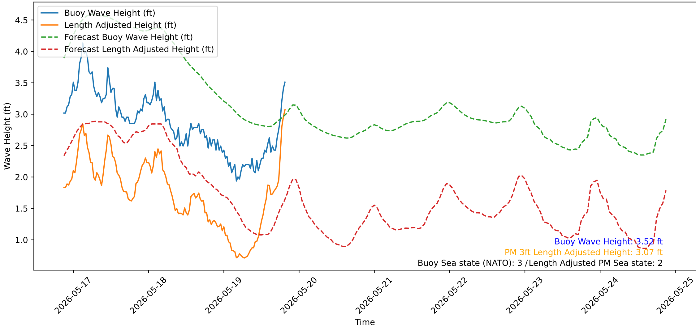
Wave Heights over Time for Red Beach at 2026-05-19 20:30:51
