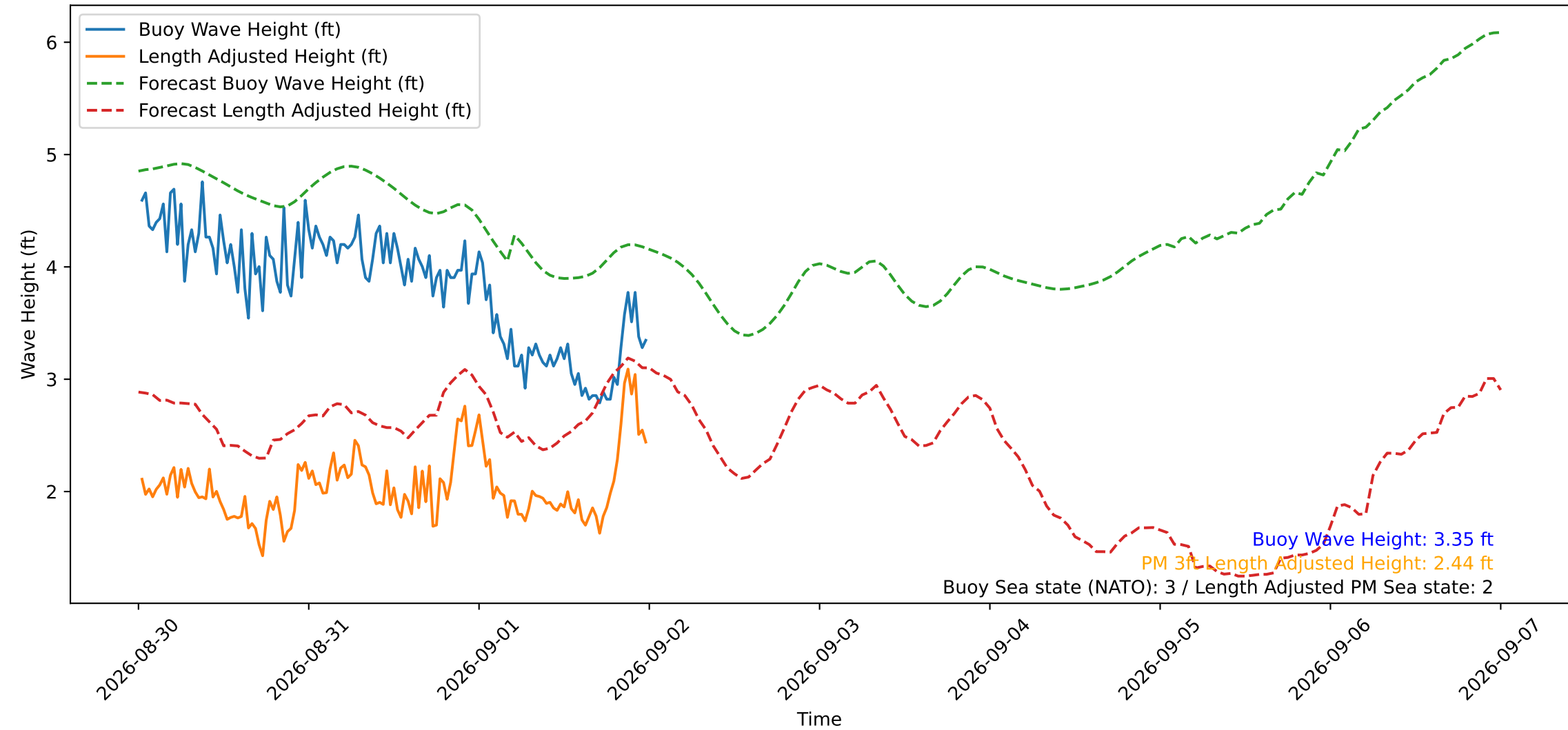
Wave Heights over Time for Green Beach at 2026-09-02 00:11:12
