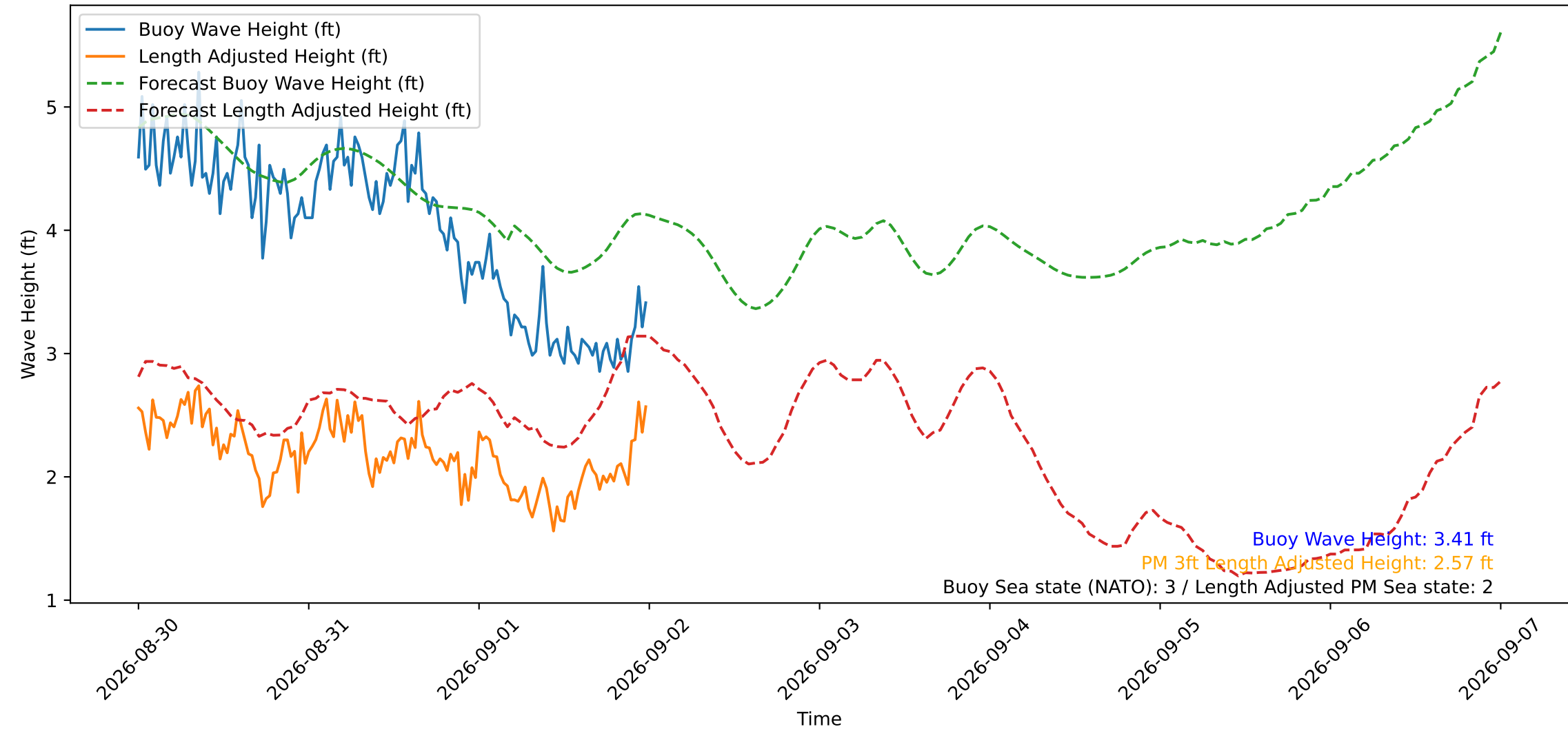
Wave Heights over Time for Oceanside Harbor at 2026-09-02 00:10:30
