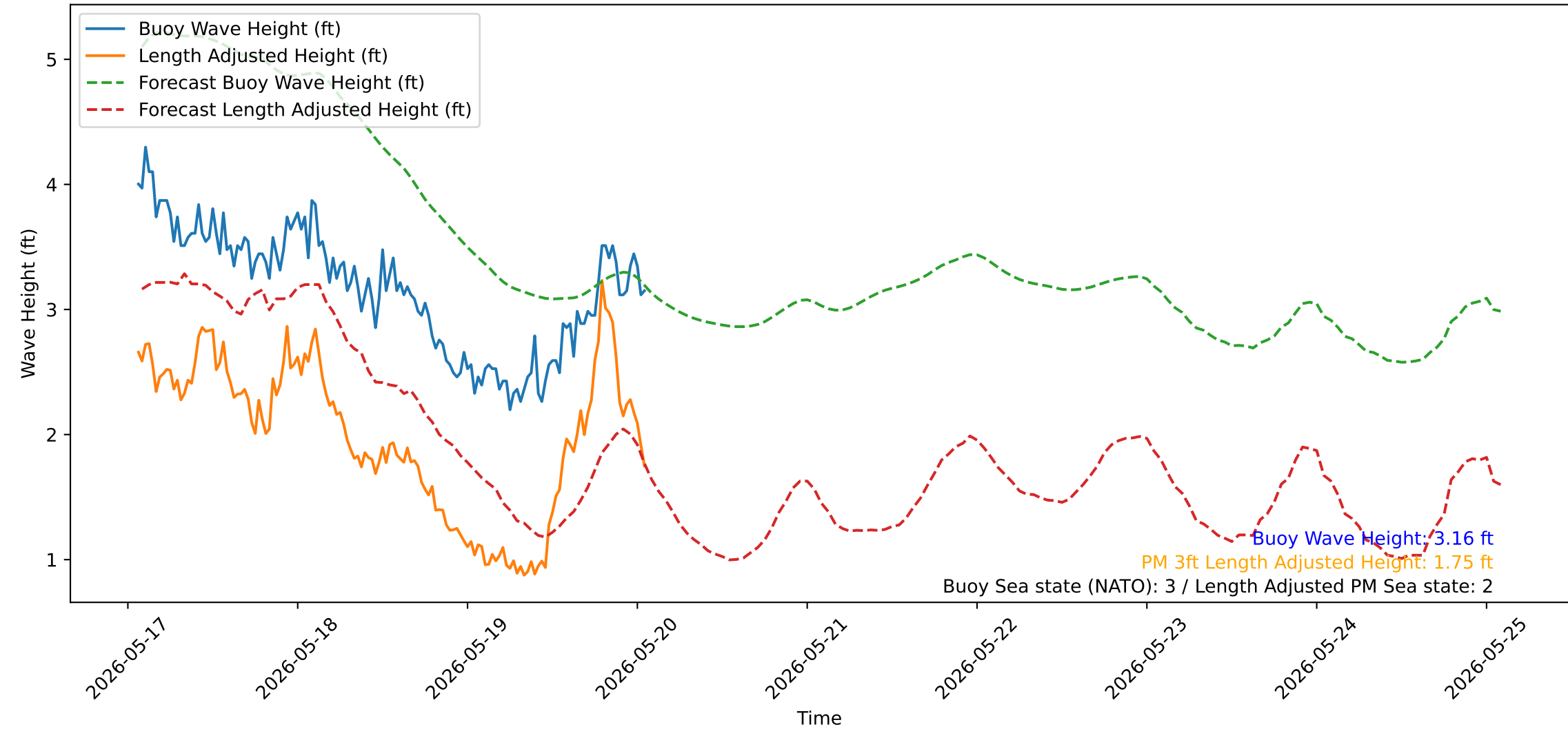
Wave Heights over Time for Oceanside Harbor at 2026-05-20 01:40:31
