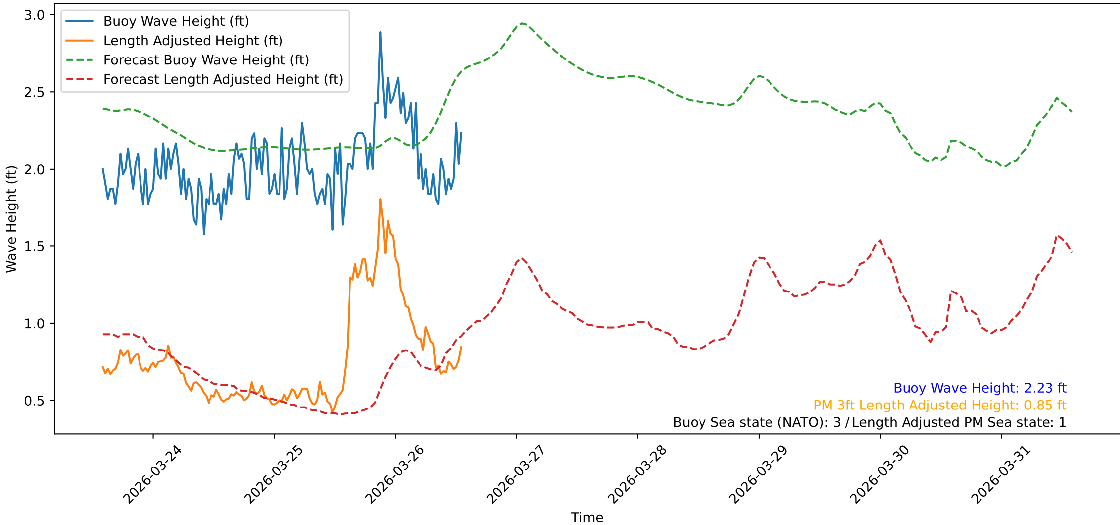
Wave Heights over Time for Oceanside Harbor at 2026-03-26 13:50:31
