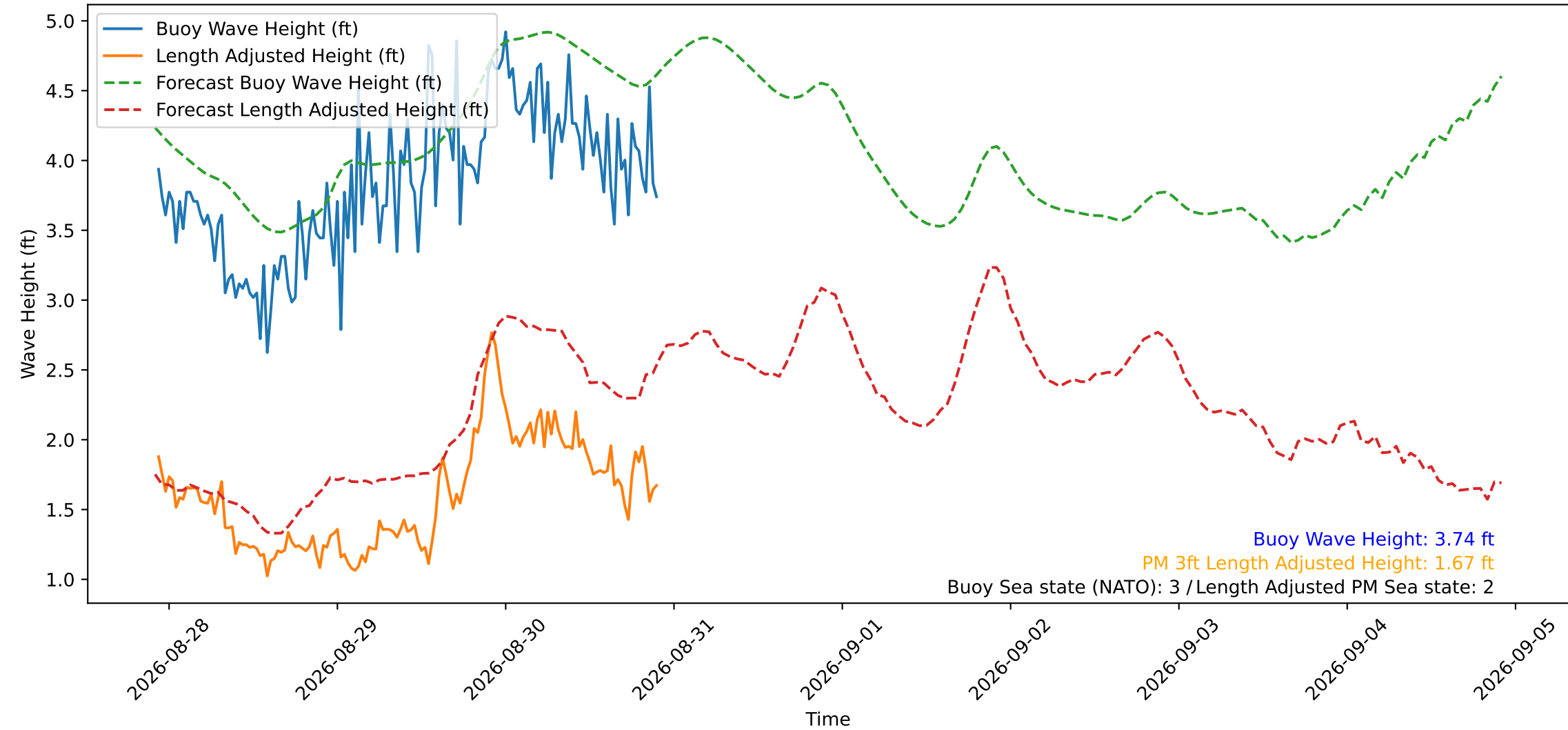
Wave Heights over Time for Green Beach at 2026-08-30 22:11:12
