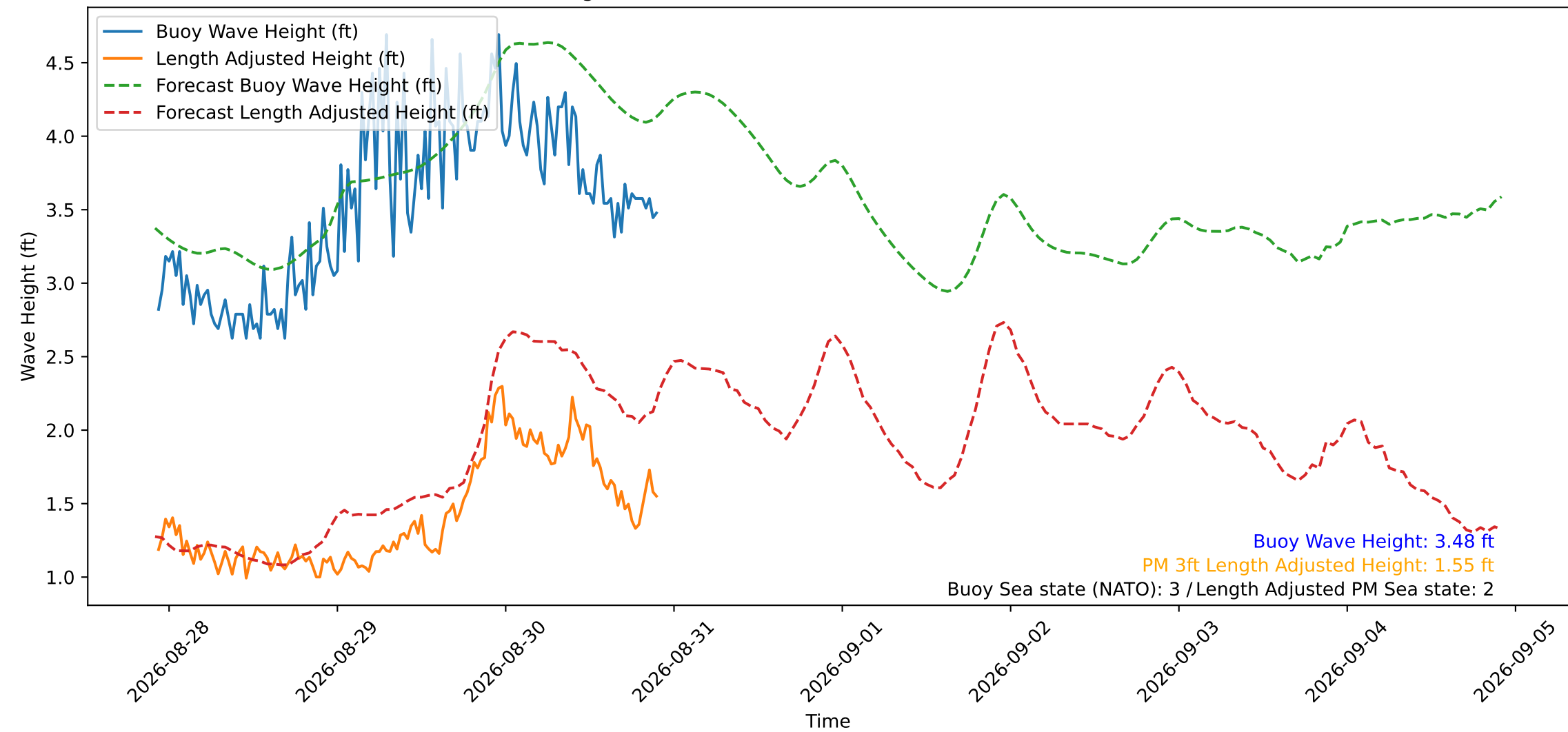
Wave Heights over Time for Red Beach at 2026-08-30 22:10:49
