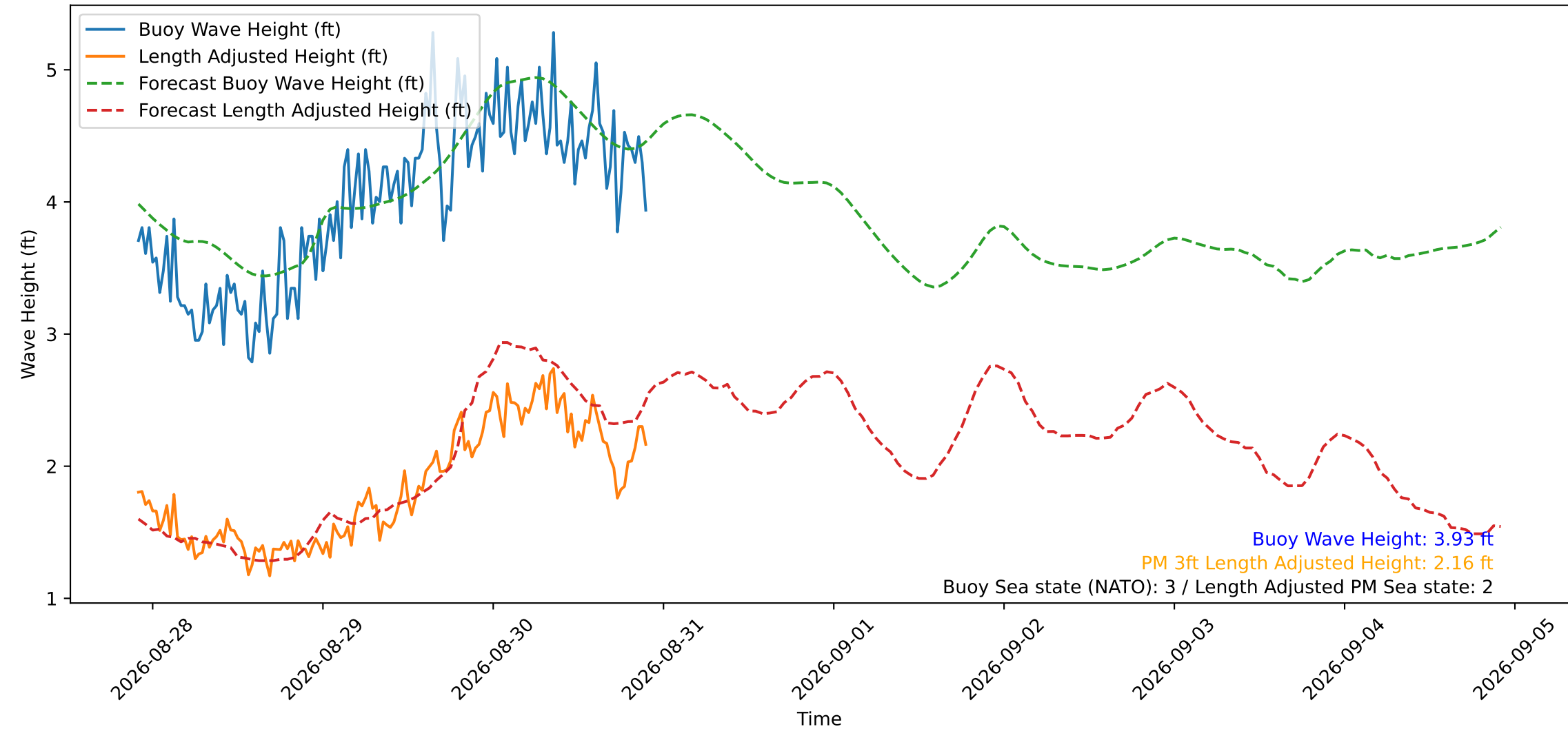
Wave Heights over Time for Oceanside Harbor at 2026-08-30 22:10:29
