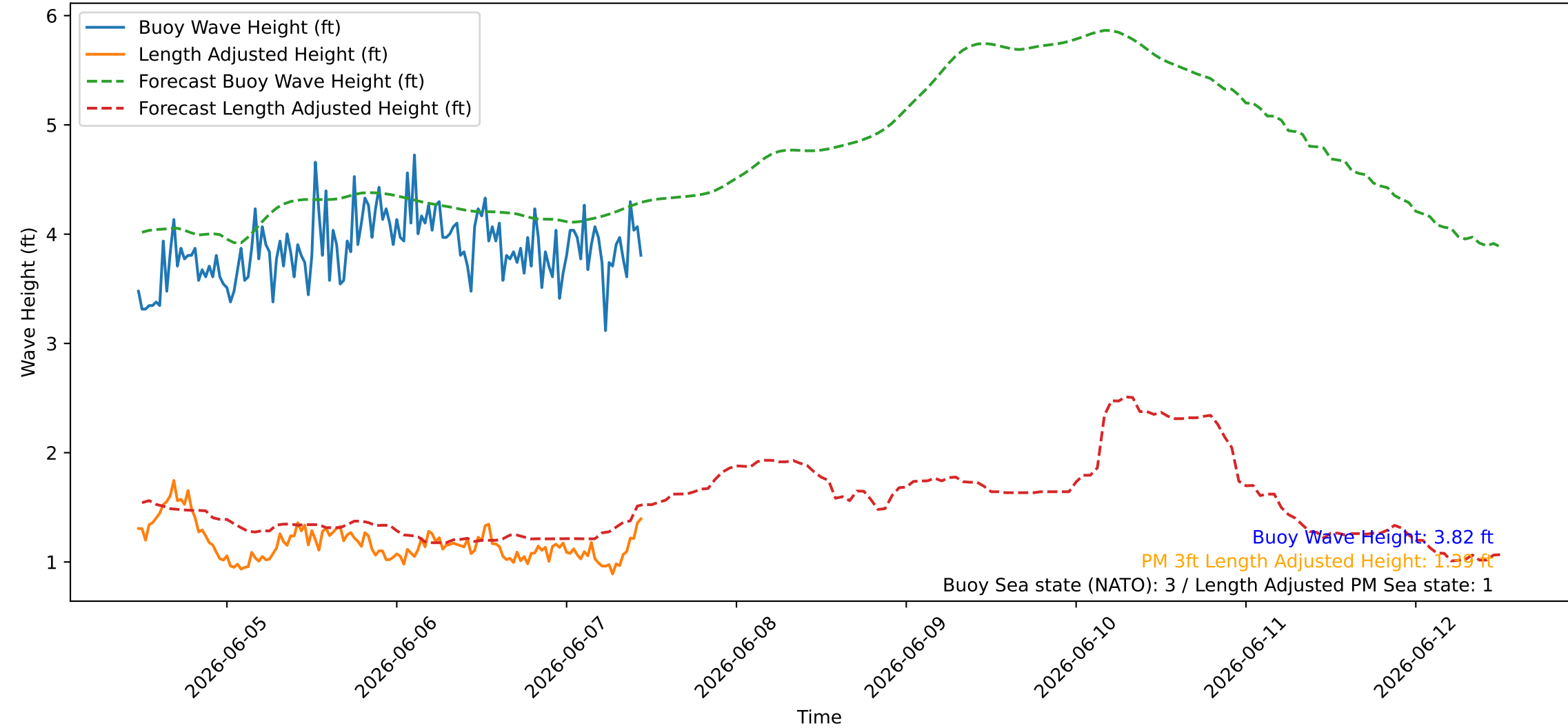
Wave Heights over Time for Green Beach at 2026-06-07 11:31:09
