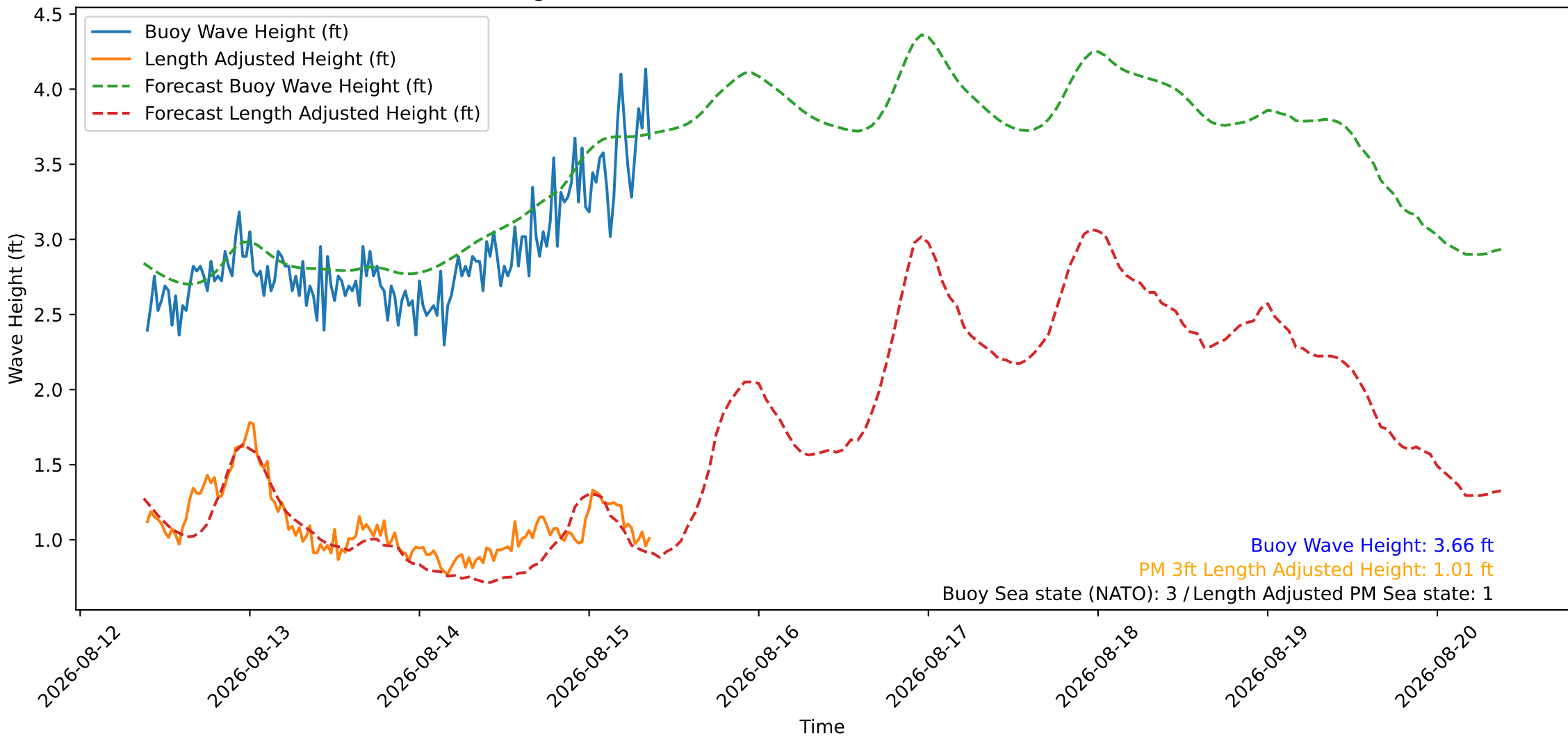
Wave Heights over Time for Oceanside Harbor at 2026-08-15 09:20:26
