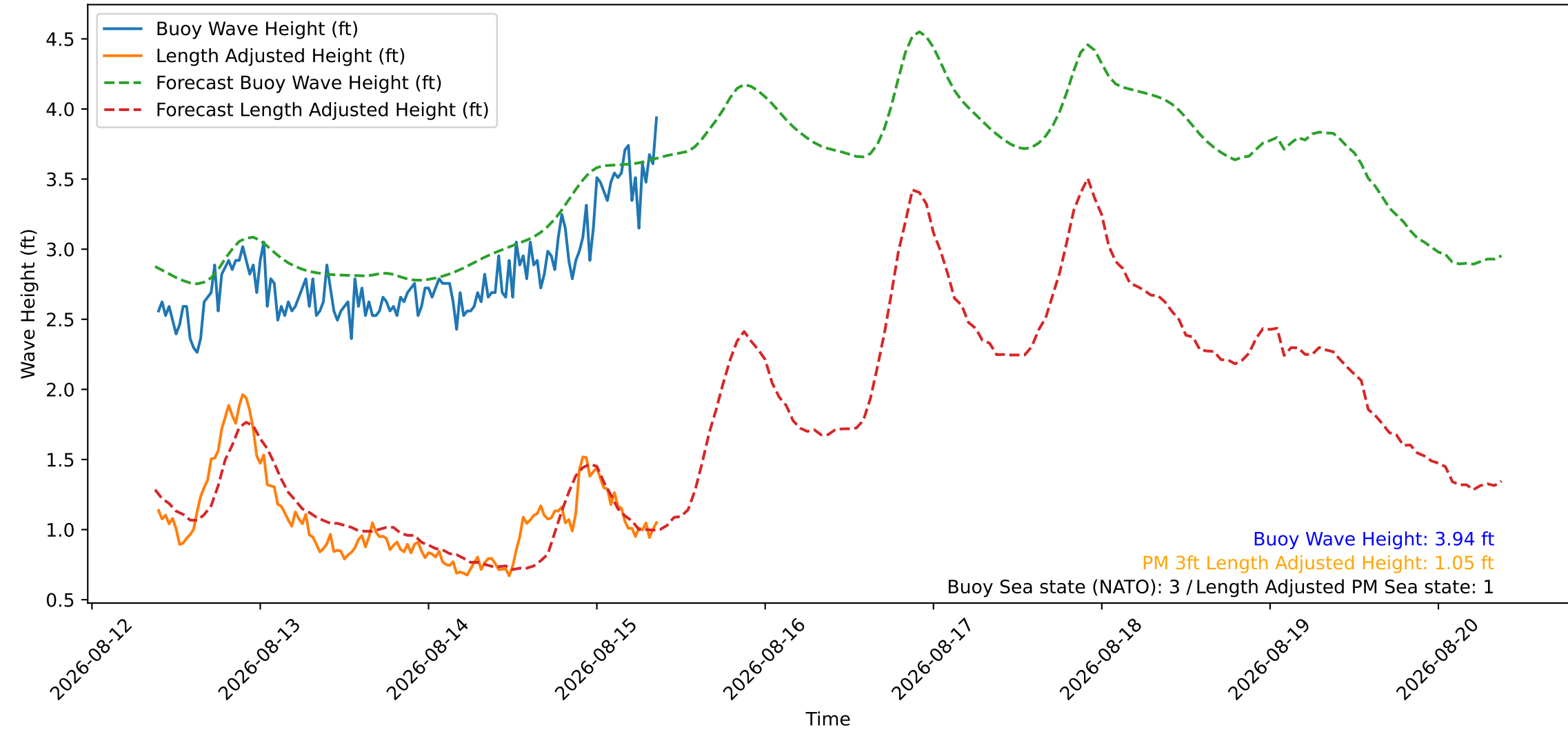
Wave Heights over Time for Green Beach at 2026-08-15 09:21:09
