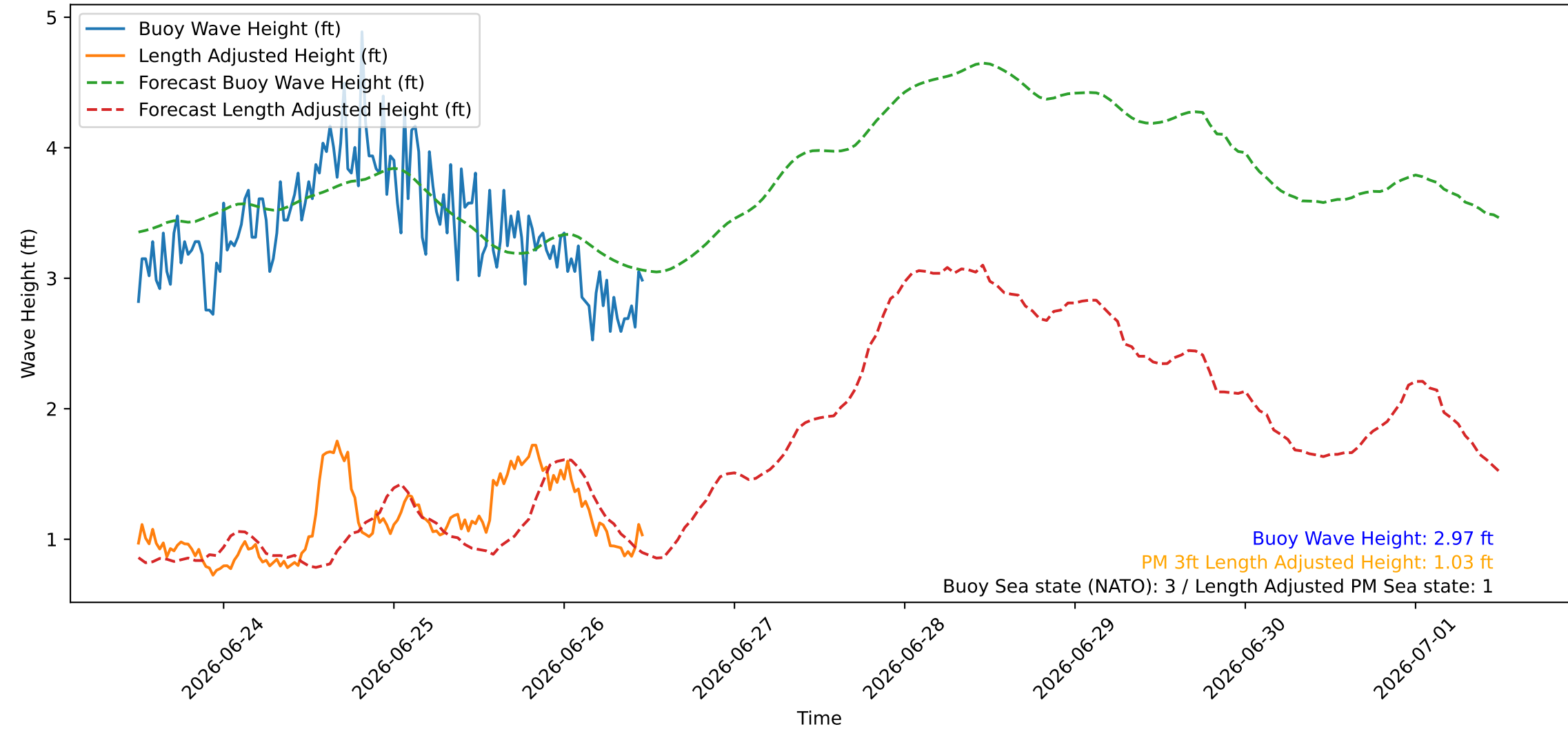
Wave Heights over Time for Oceanside Harbor at 2026-06-26 11:50:26
