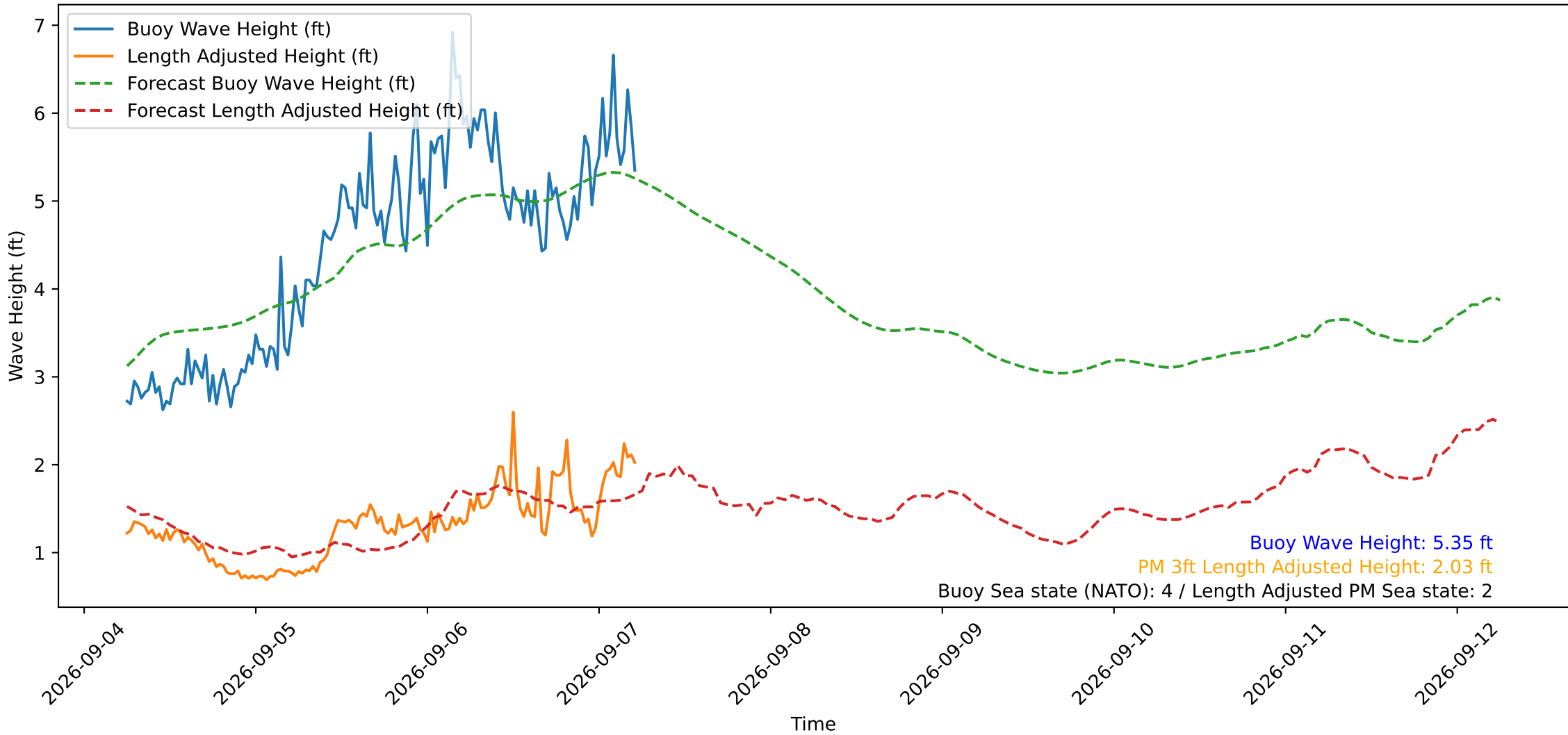
Wave Heights over Time for Red Beach at 2026-09-07 05:50:50
