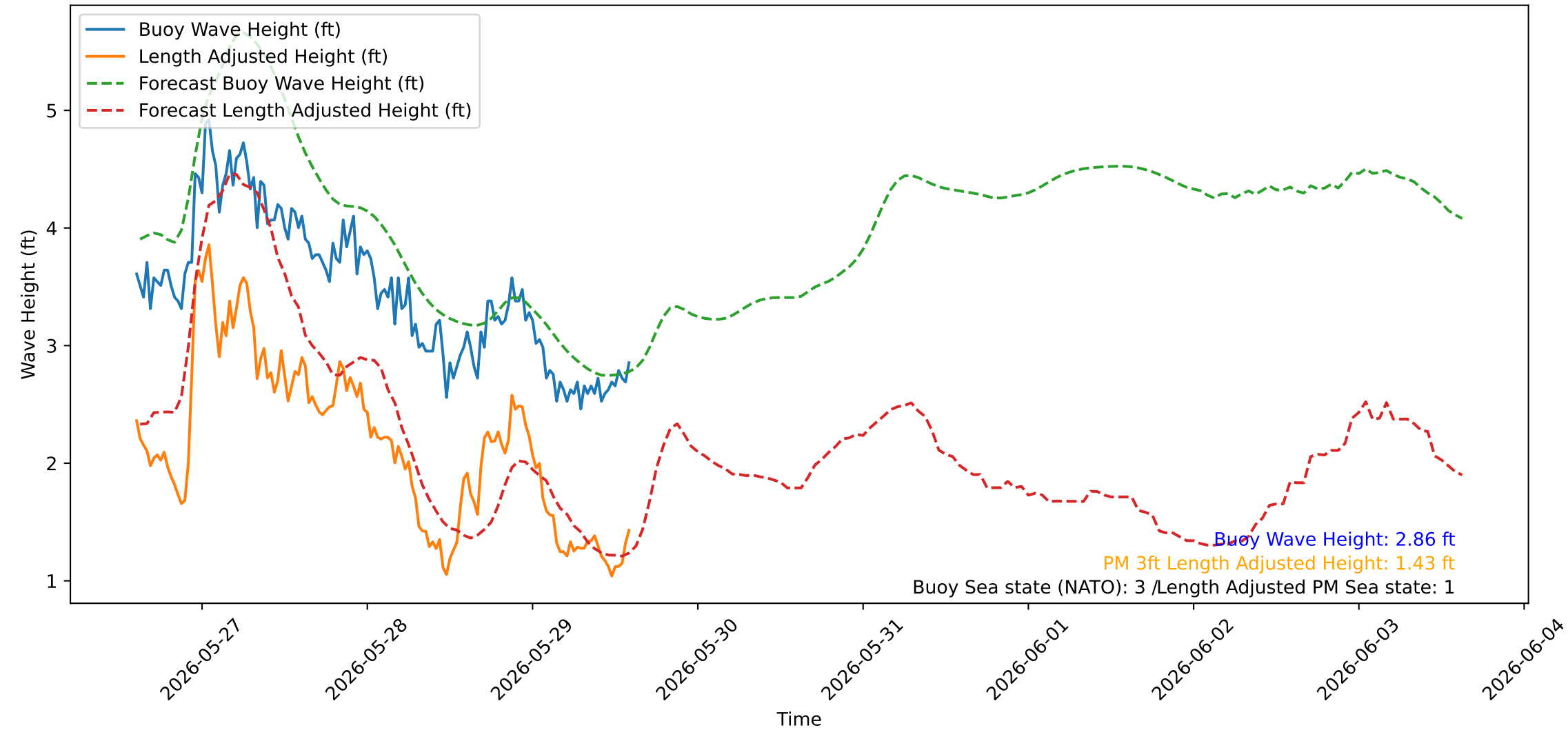
Wave Heights over Time for Green Beach at 2026-05-29 14:41:04
