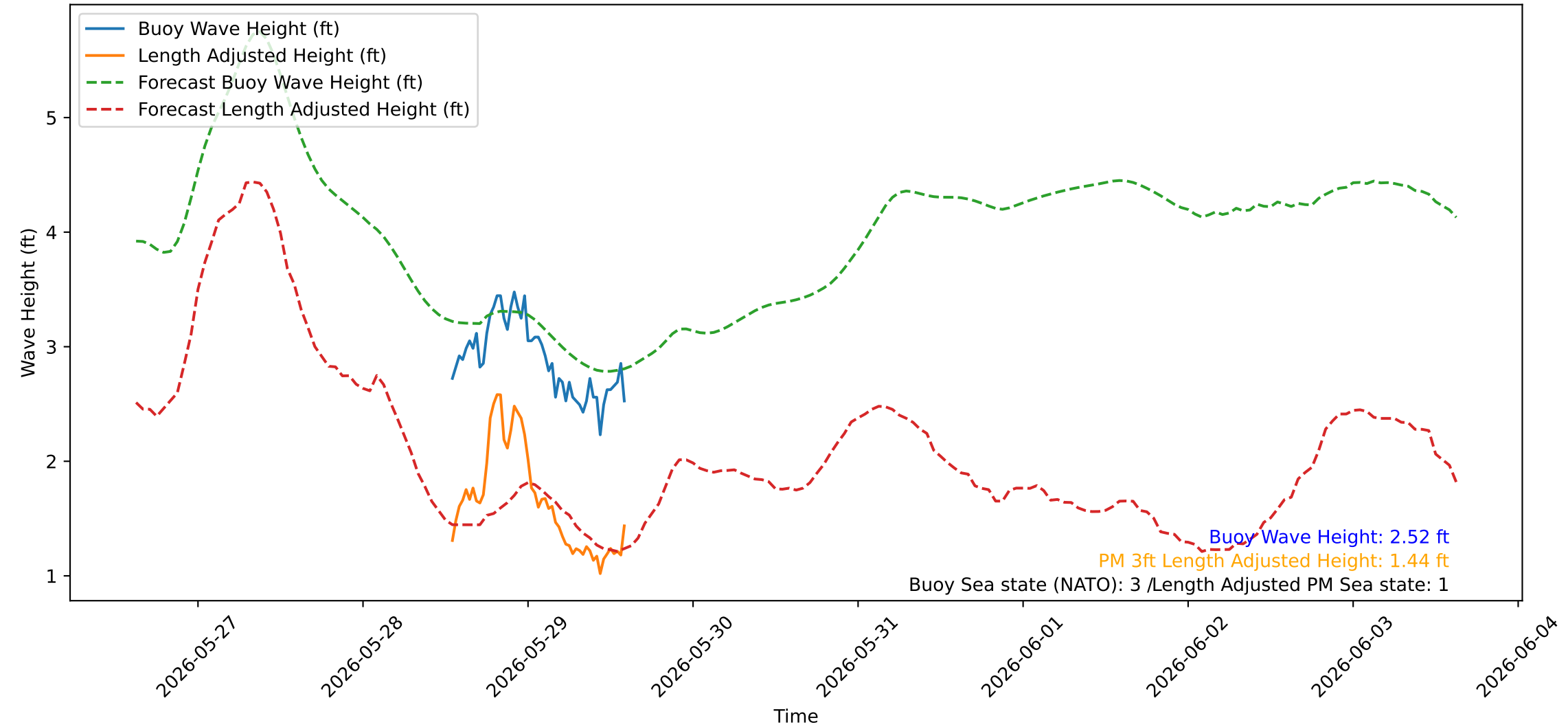
Wave Heights over Time for Oceanside Harbor at 2026-05-29 14:40:22
