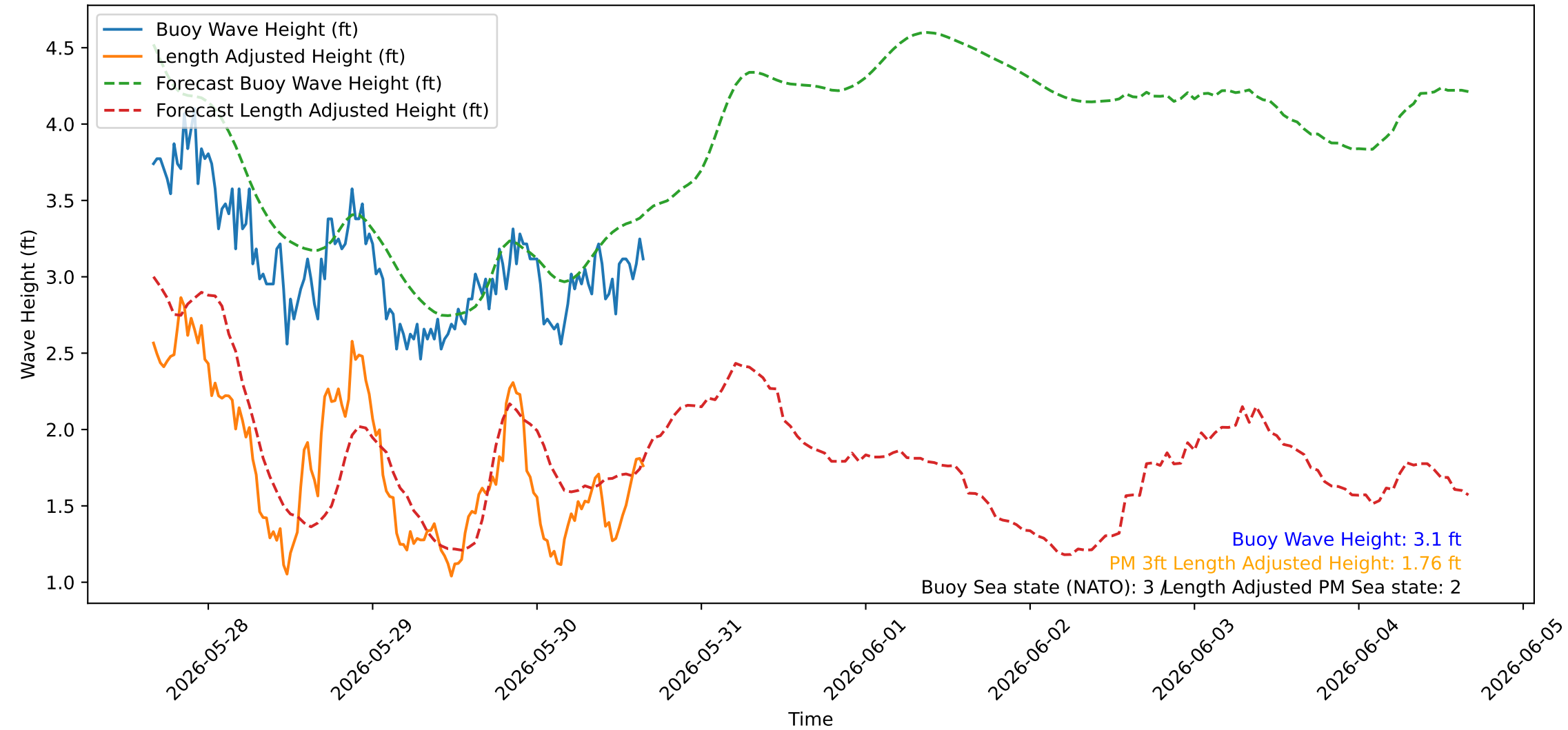
Wave Heights over Time for Green Beach at 2026-05-30 16:11:06
