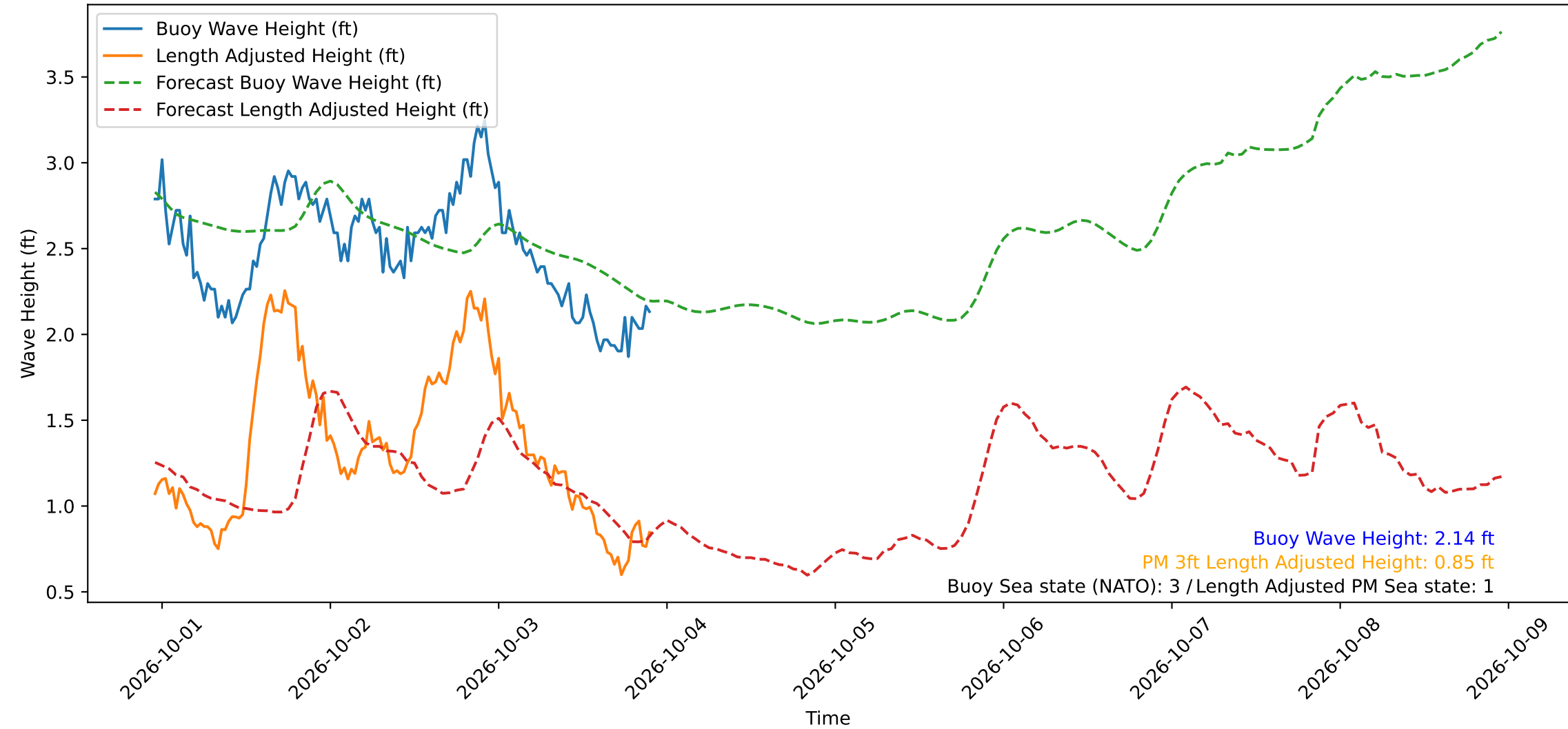
Wave Heights over Time for Red Beach at 2026-10-03 22:30:48
