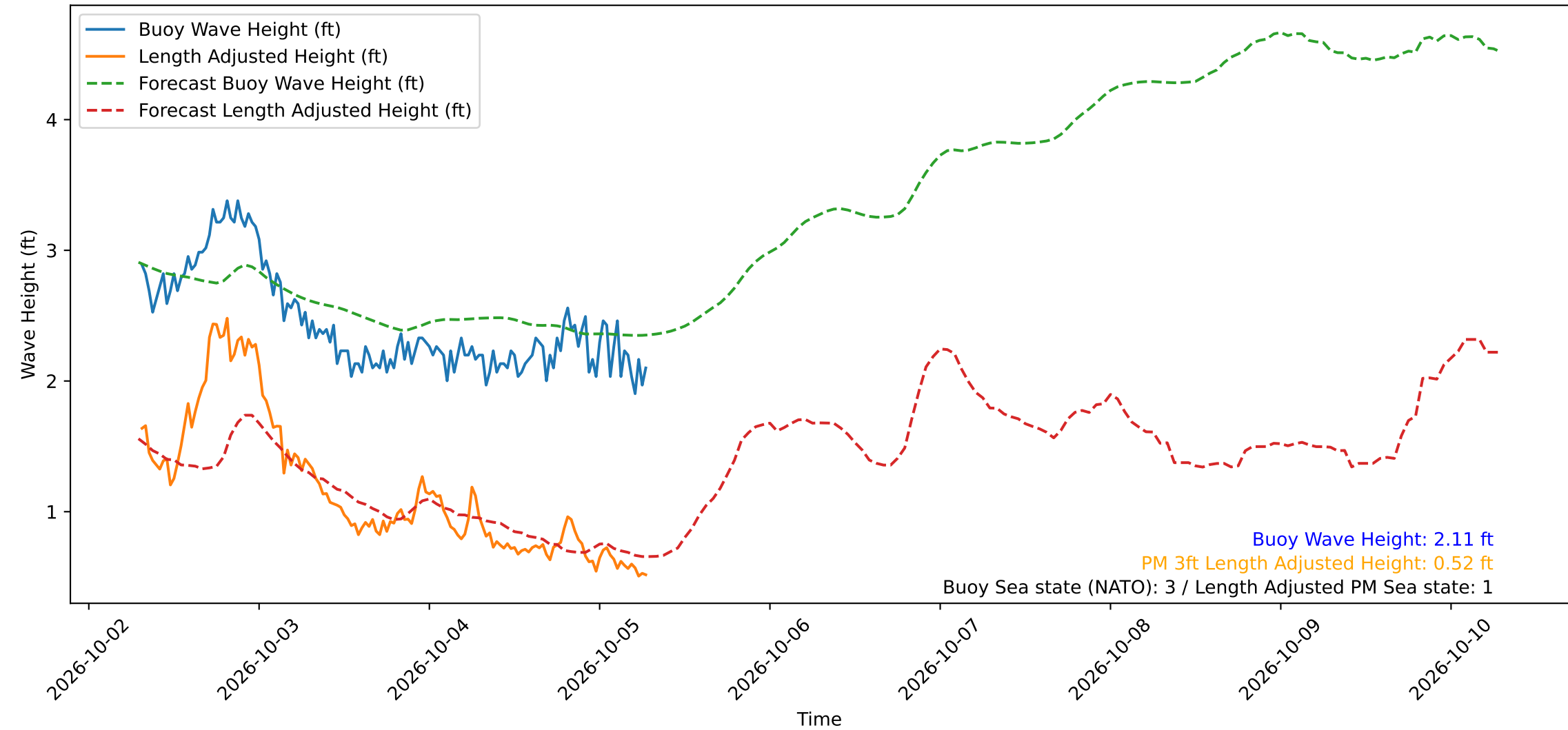
Wave Heights over Time for Green Beach at 2026-10-05 07:11:12
