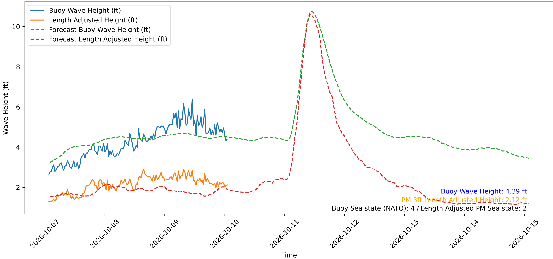
Wave Heights over Time for Oceanside Harbor at 2026-10-10 01:40:30
