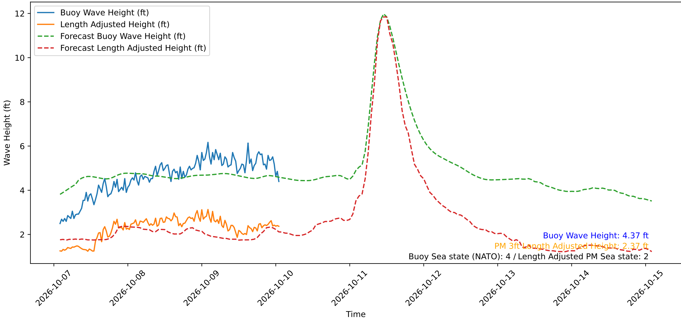
Wave Heights over Time for Green Beach at 2026-10-10 01:41:12
