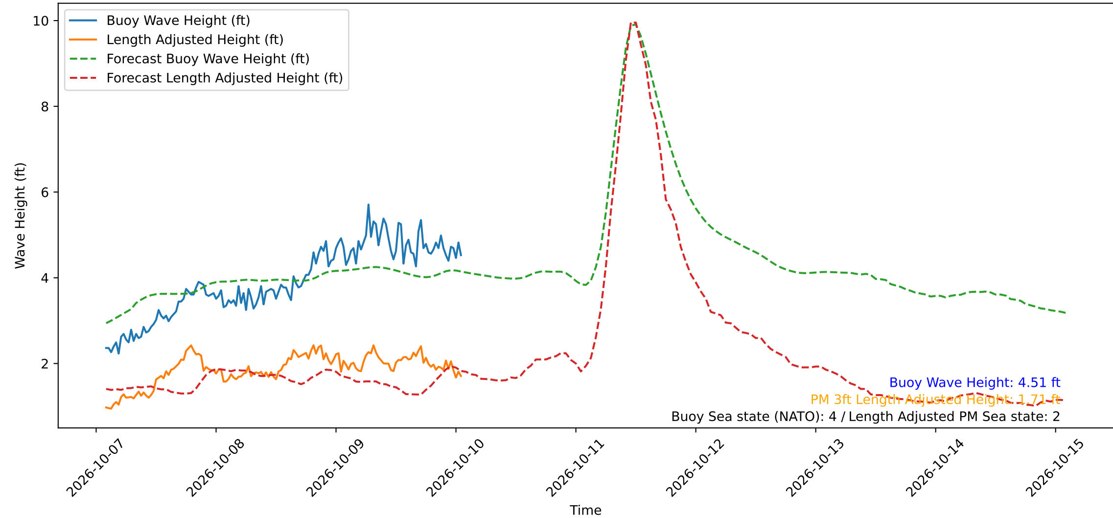
Wave Heights over Time for Red Beach at 2026-10-10 01:40:49
