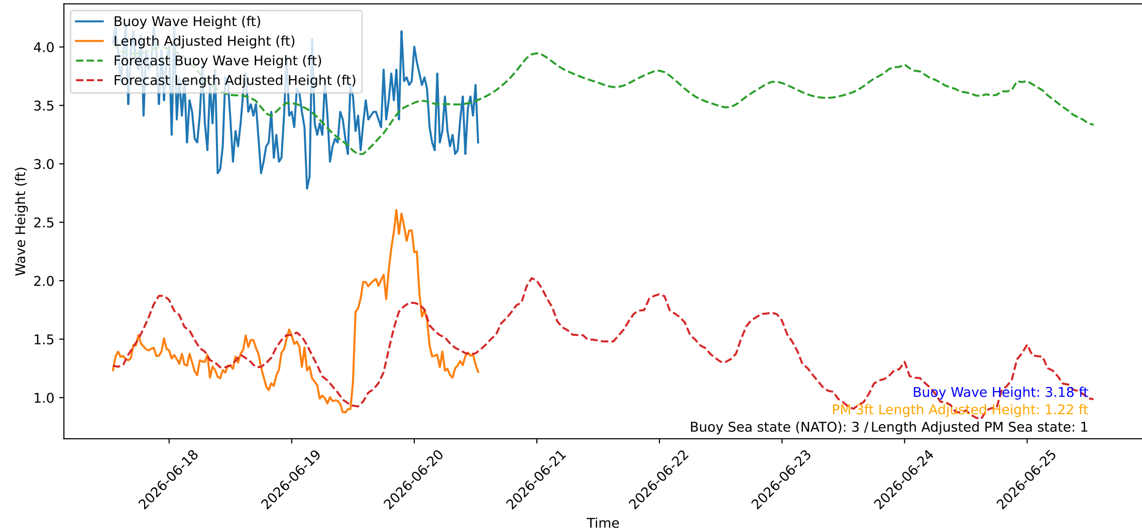
Wave Heights over Time for Oceanside Harbor at 2026-06-20 13:10:25
