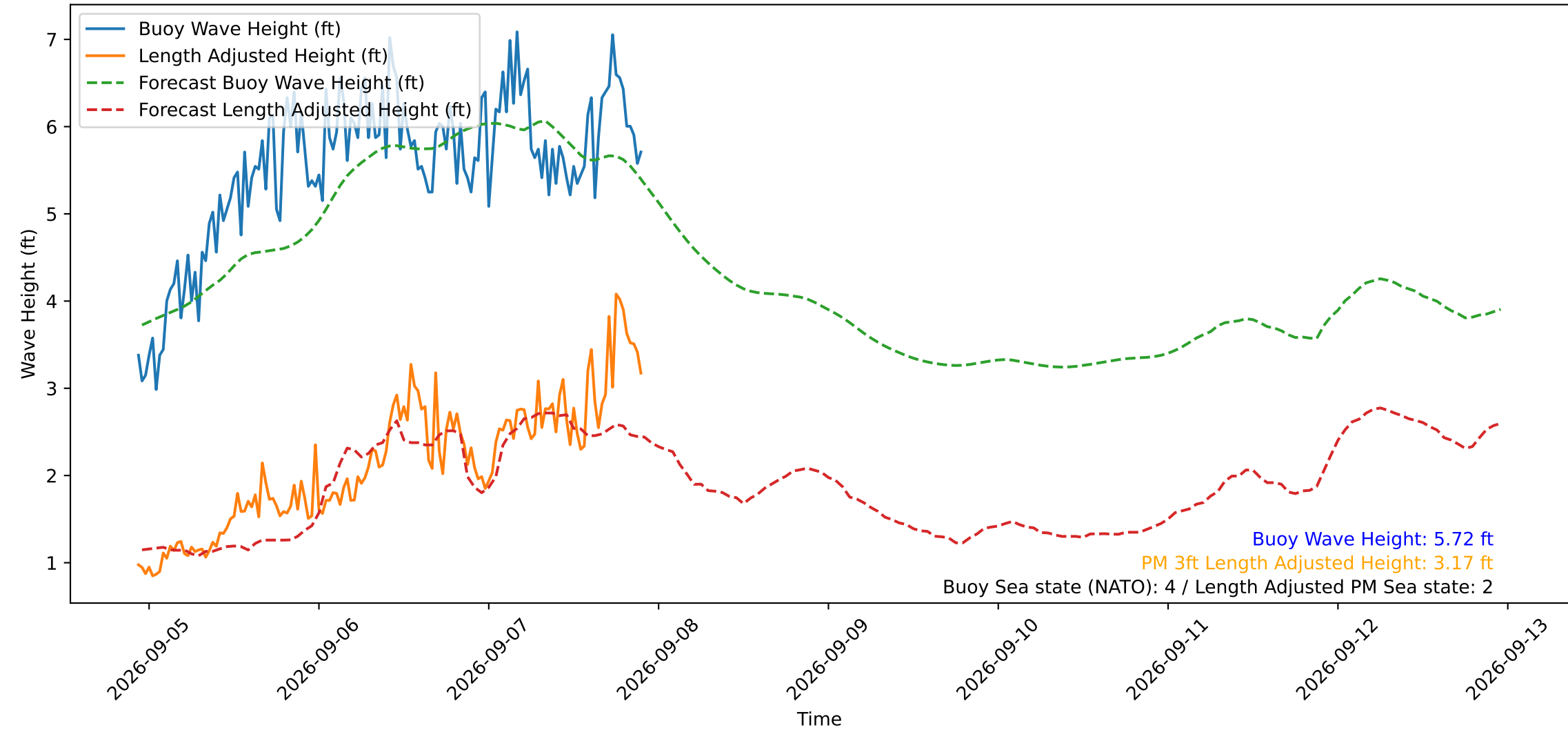
Wave Heights over Time for Oceanside Harbor at 2026-09-07 22:30:30
