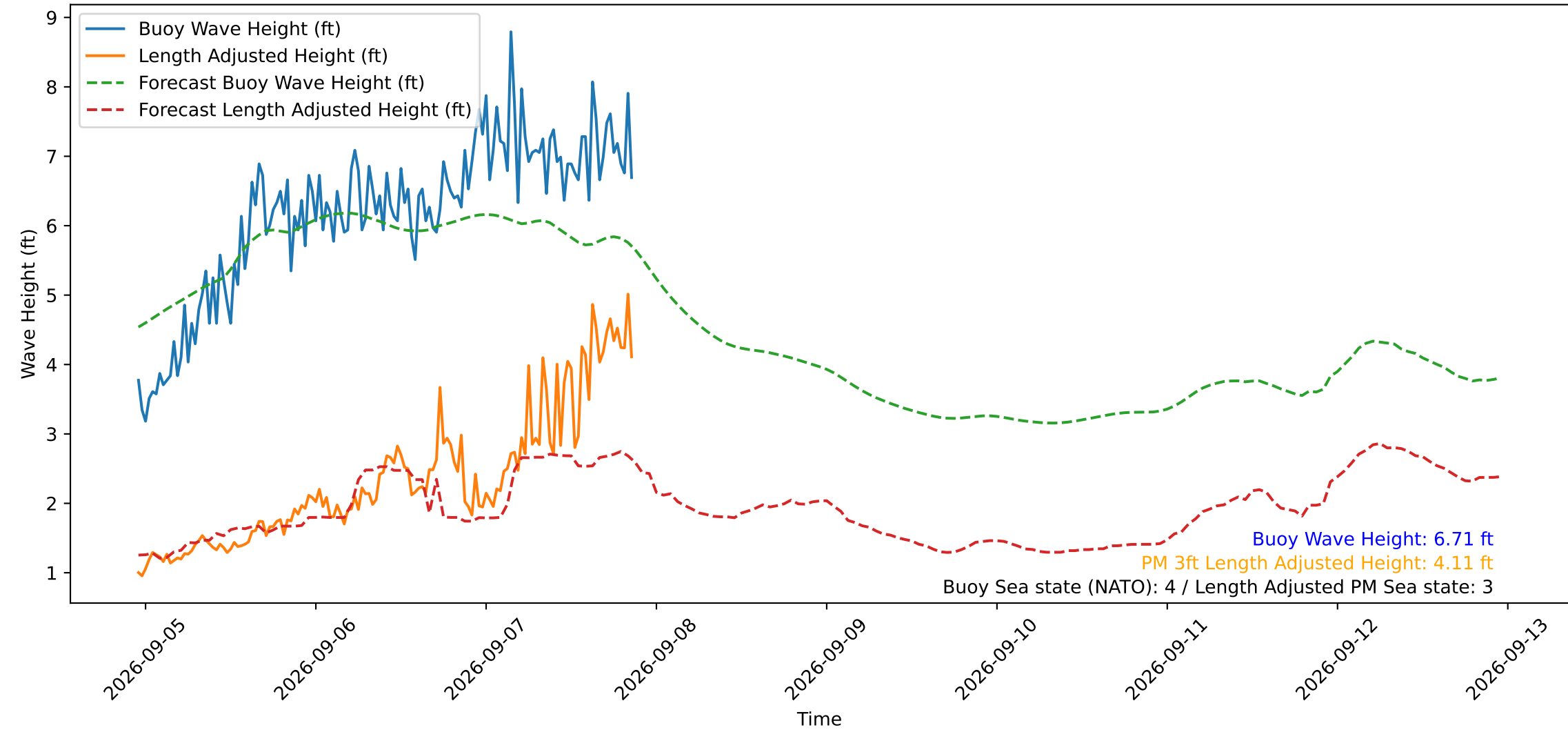
Wave Heights over Time for Green Beach at 2026-09-07 22:31:11
