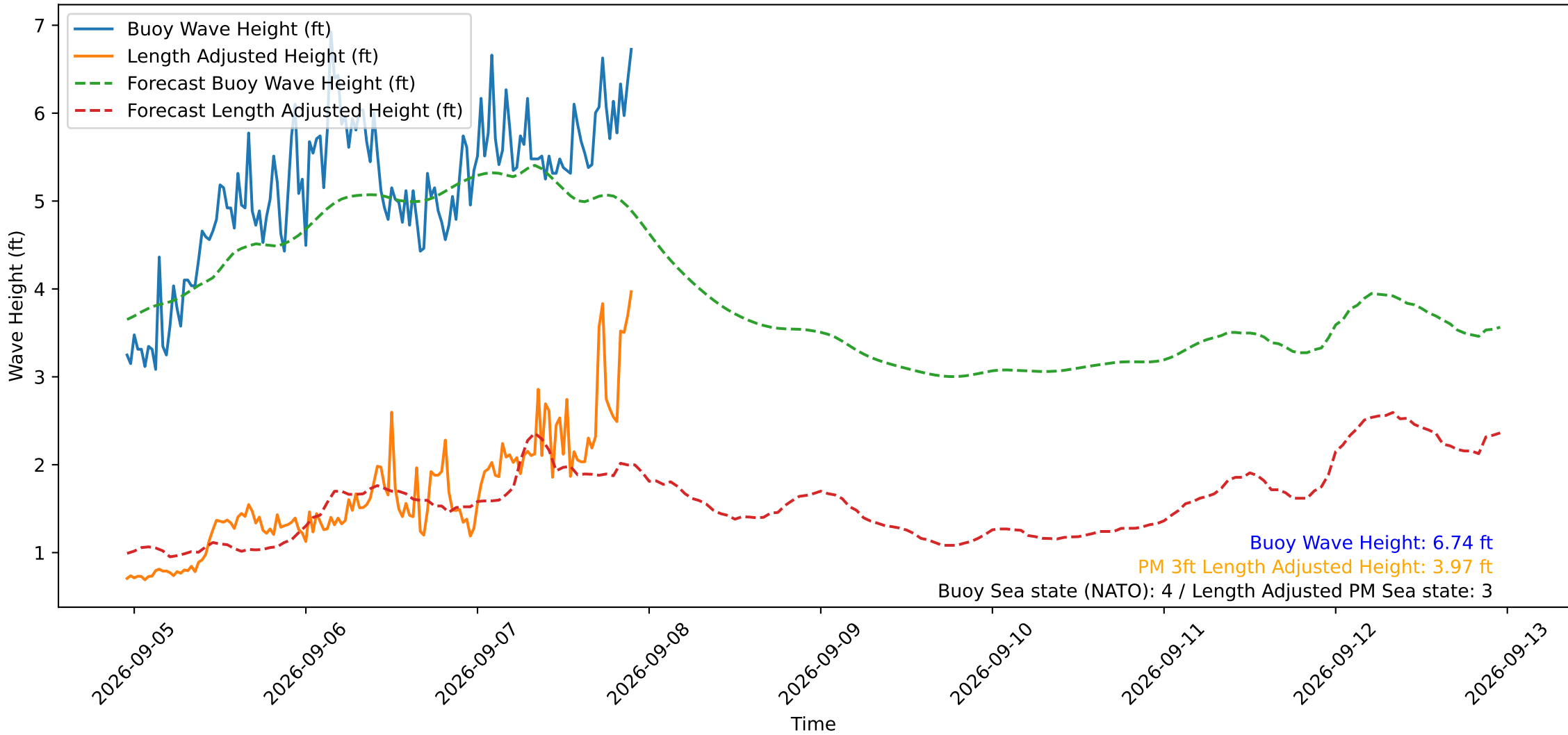
Wave Heights over Time for Red Beach at 2026-09-07 22:30:49
