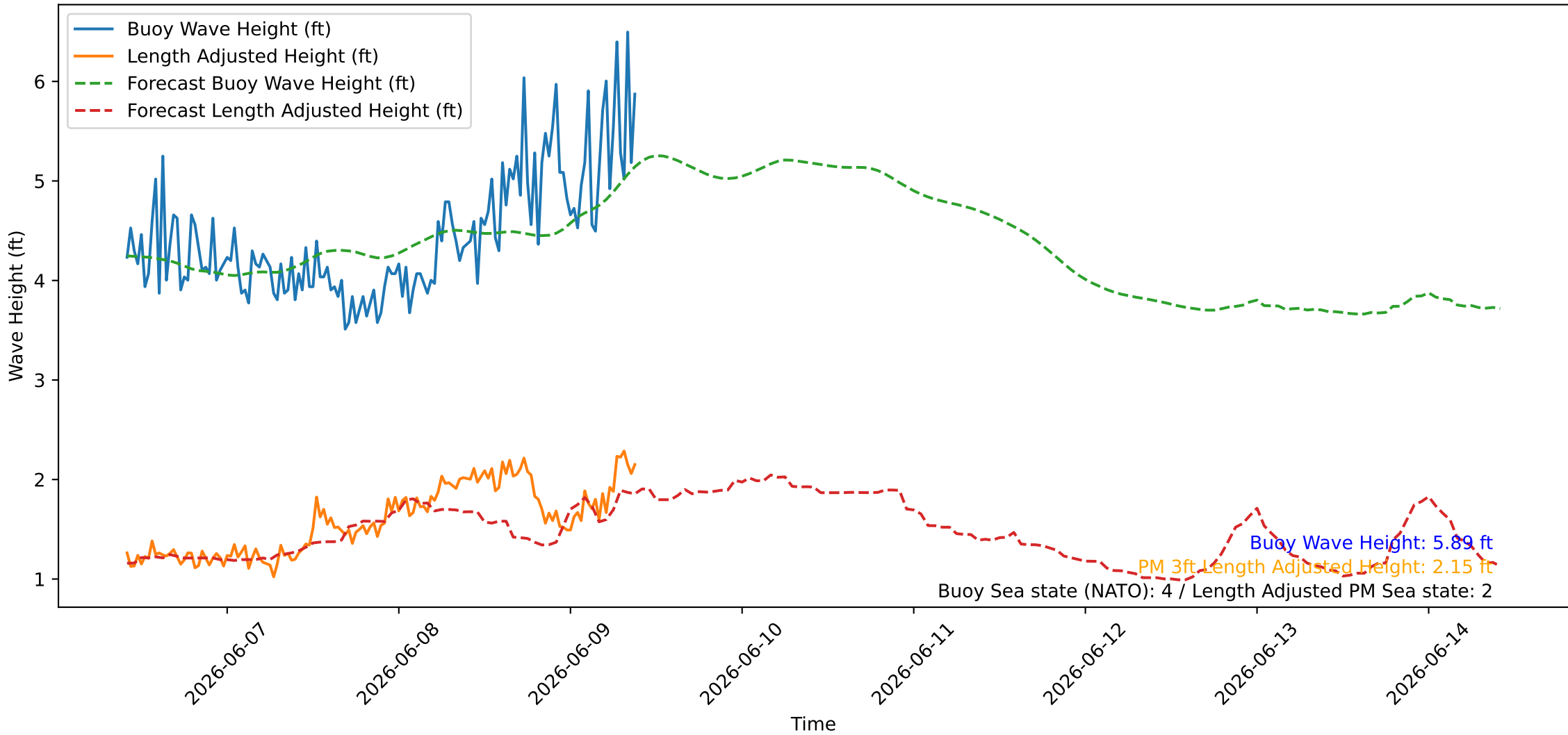
Wave Heights over Time for Oceanside Harbor at 2026-06-09 10:00:26
