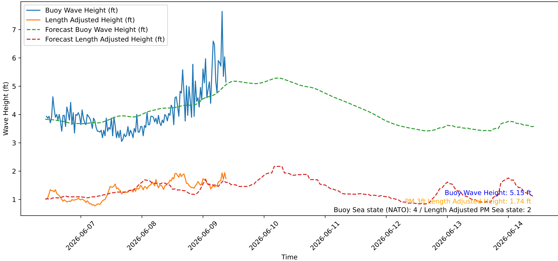
Wave Heights over Time for Red Beach at 2026-06-09 10:00:45
