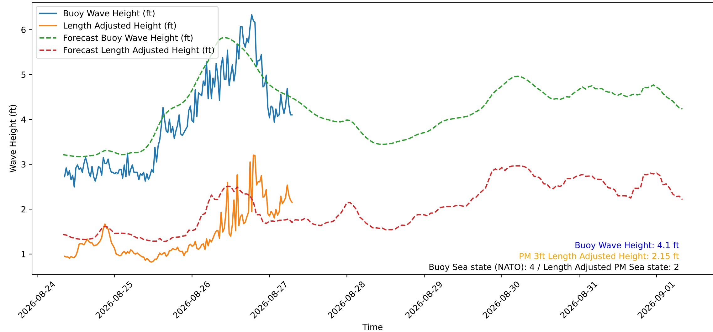
Wave Heights over Time for Green Beach at 2026-08-27 08:01:11
