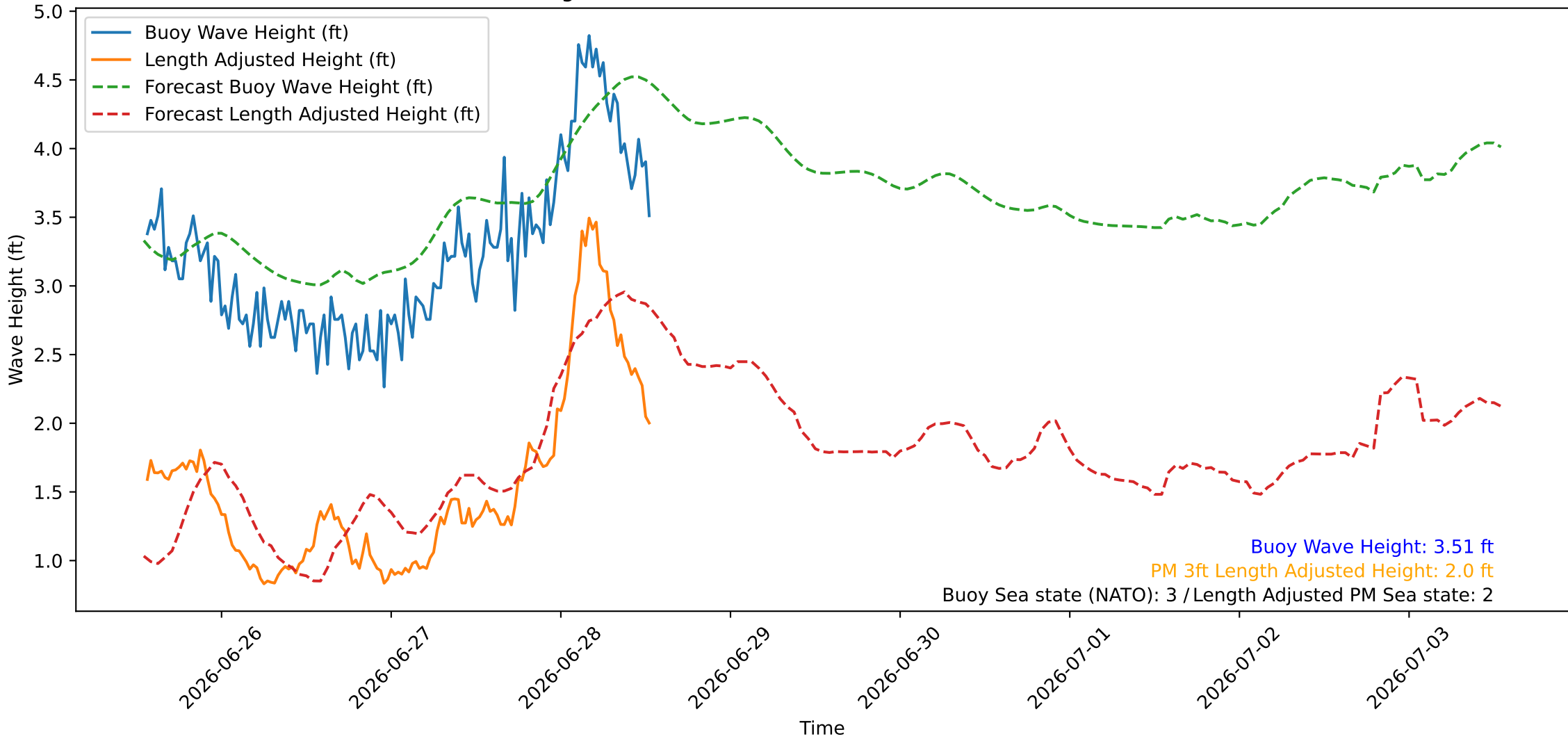
Wave Heights over Time for Green Beach at 2026-06-28 13:21:10
