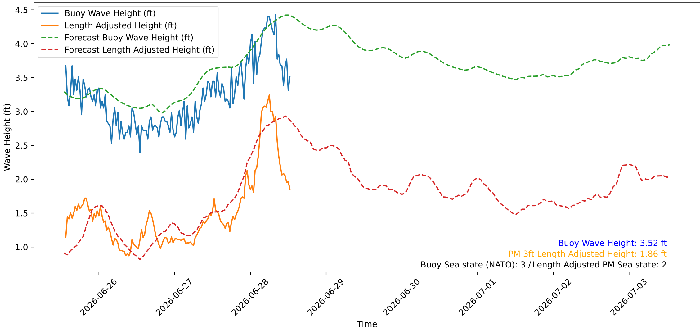
Wave Heights over Time for Oceanside Harbor at 2026-06-28 13:20:26
