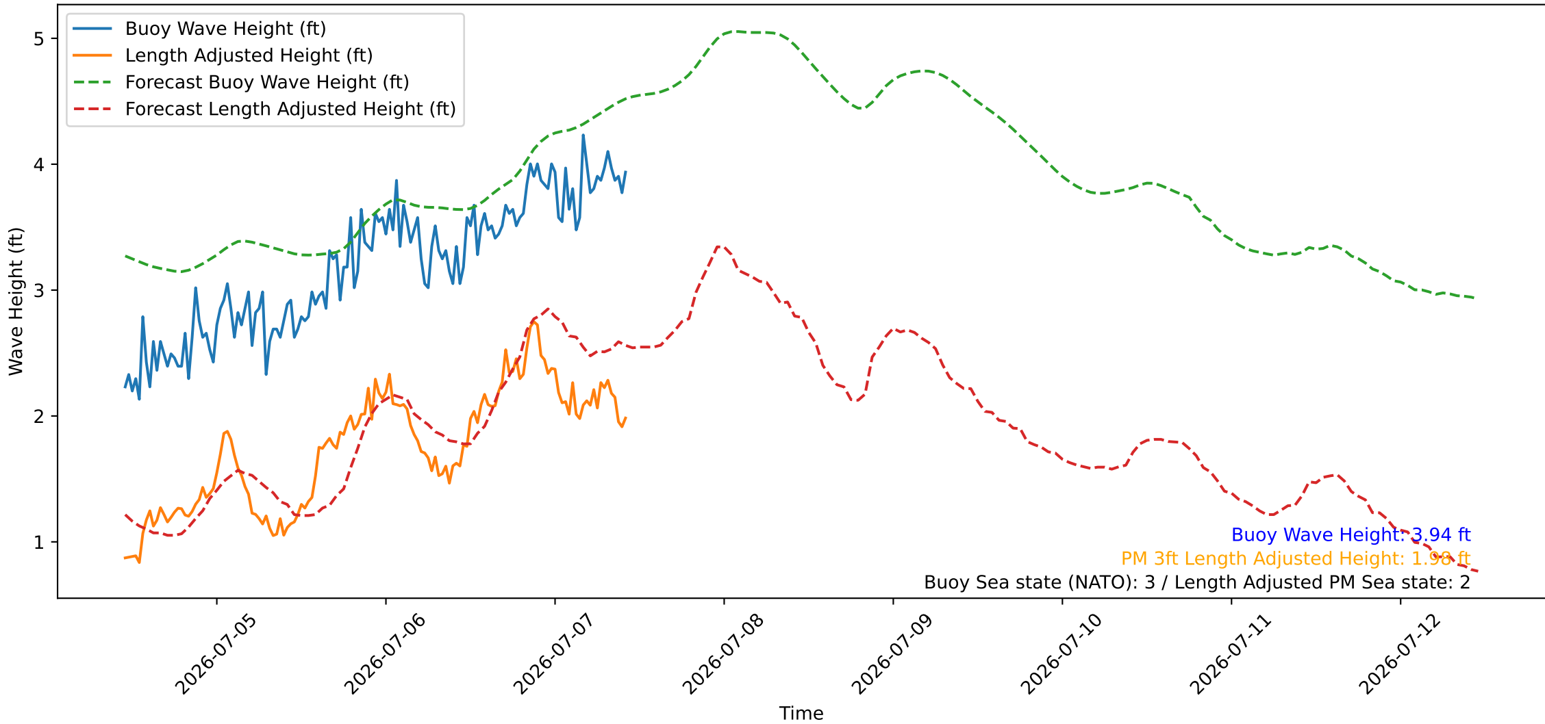
Wave Heights over Time for Oceanside Harbor at 2026-07-07 10:50:26
