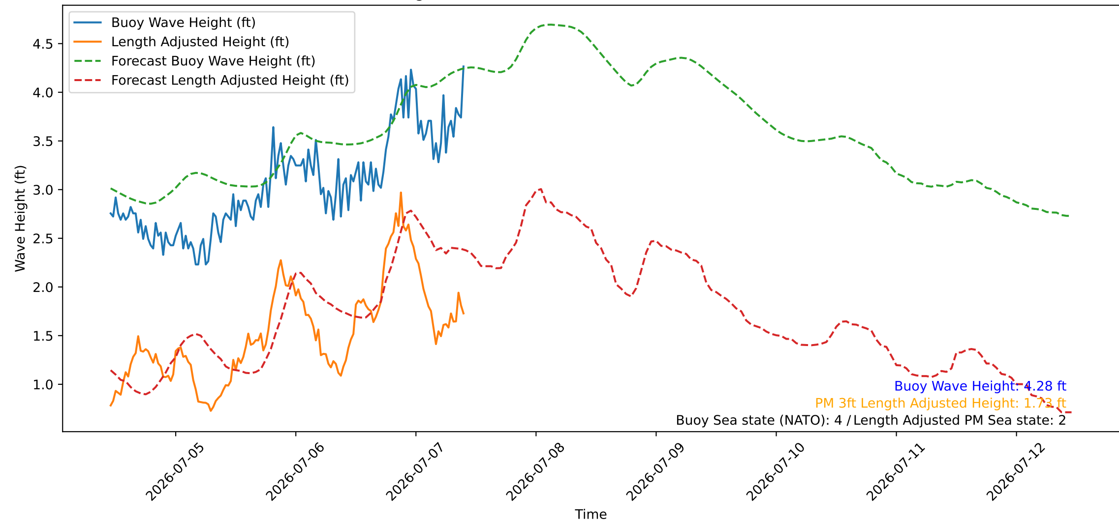
Wave Heights over Time for Red Beach at 2026-07-07 10:50:47
