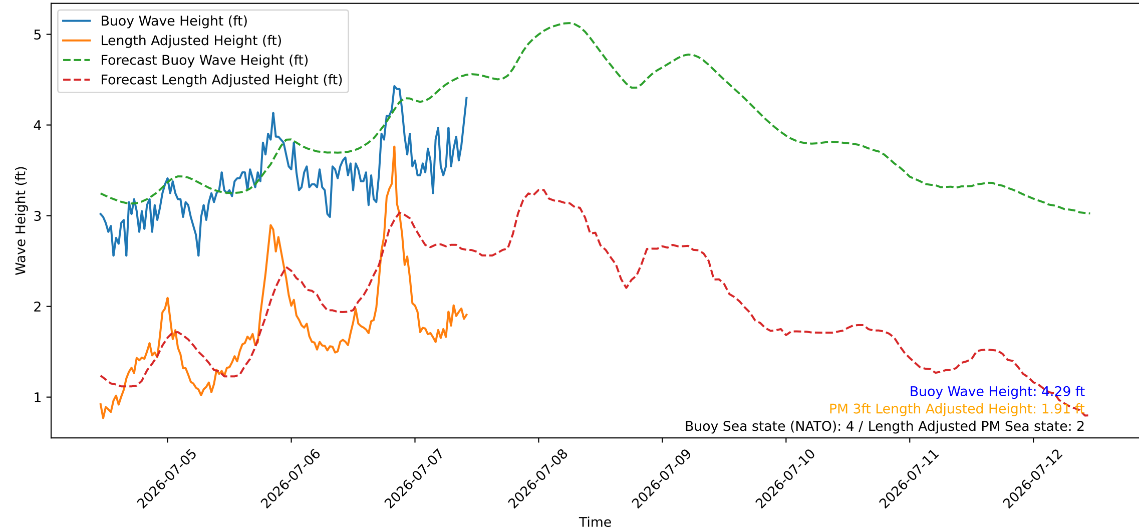
Wave Heights over Time for Green Beach at 2026-07-07 10:51:09
