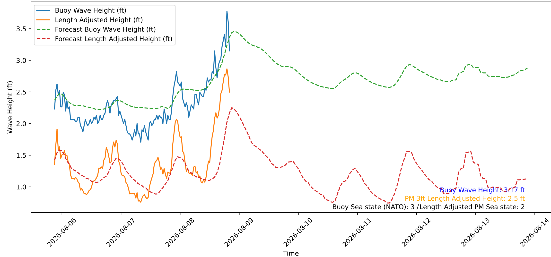
Wave Heights over Time for Green Beach at 2026-08-08 21:01:08
