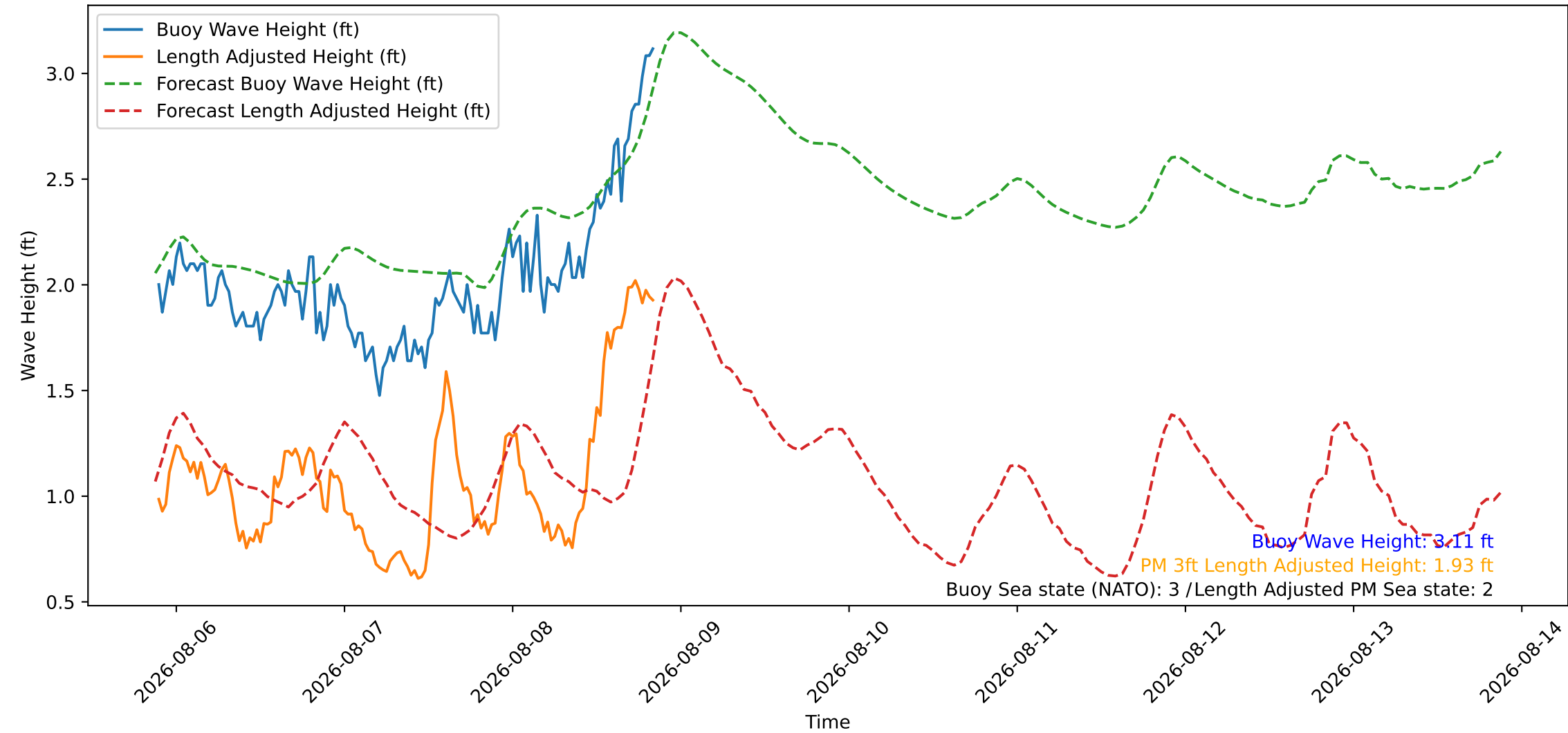
Wave Heights over Time for Red Beach at 2026-08-08 21:00:45
