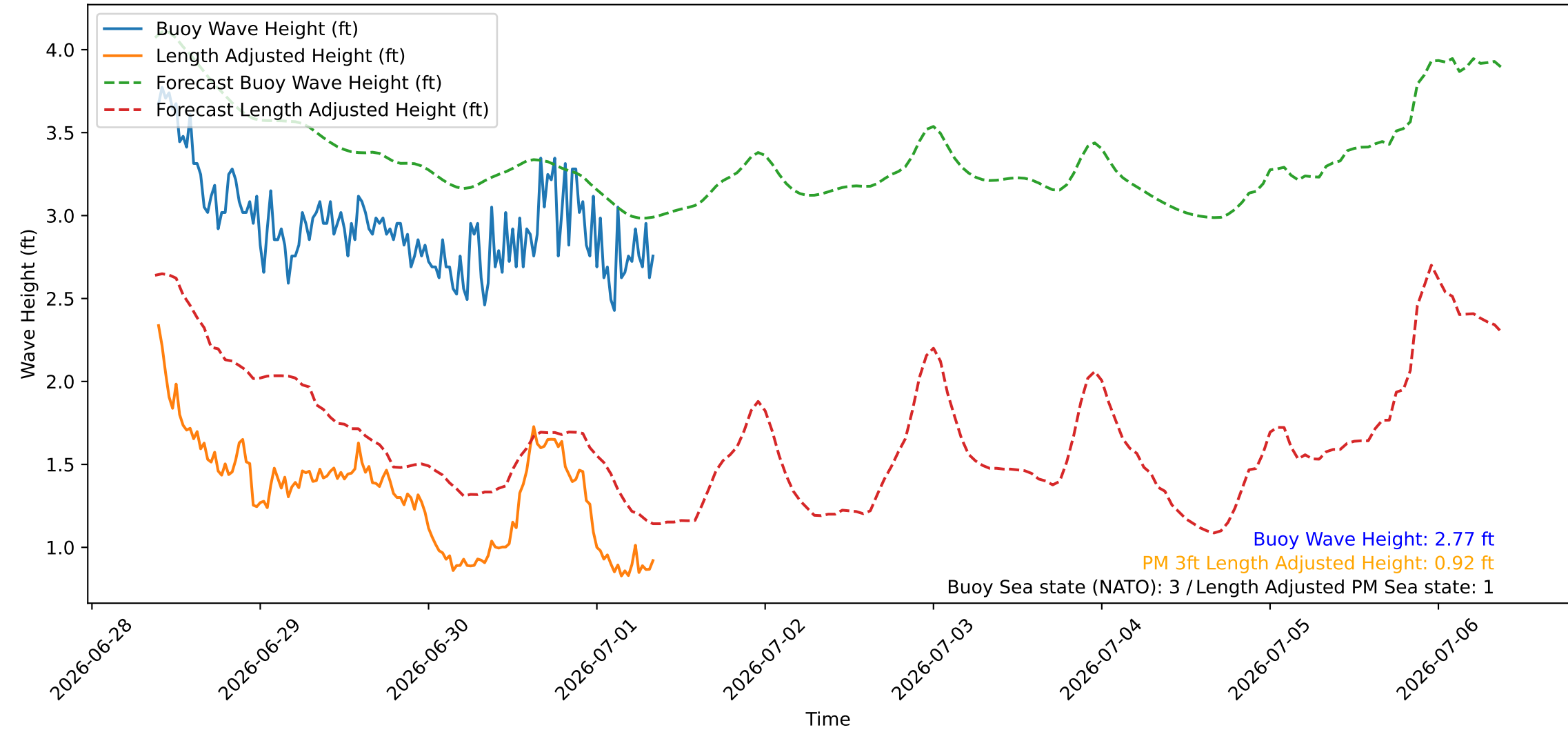
Wave Heights over Time for Red Beach at 2026-07-01 09:10:45
