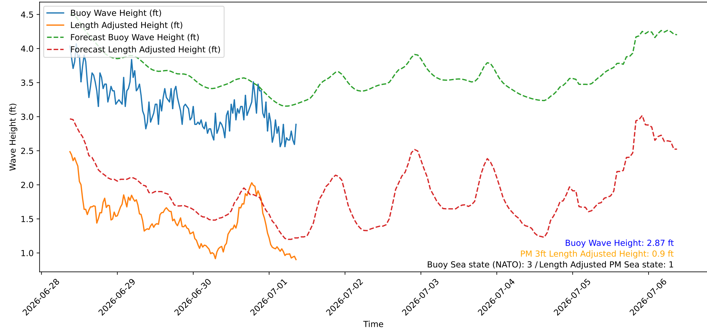
Wave Heights over Time for Green Beach at 2026-07-01 09:11:07
