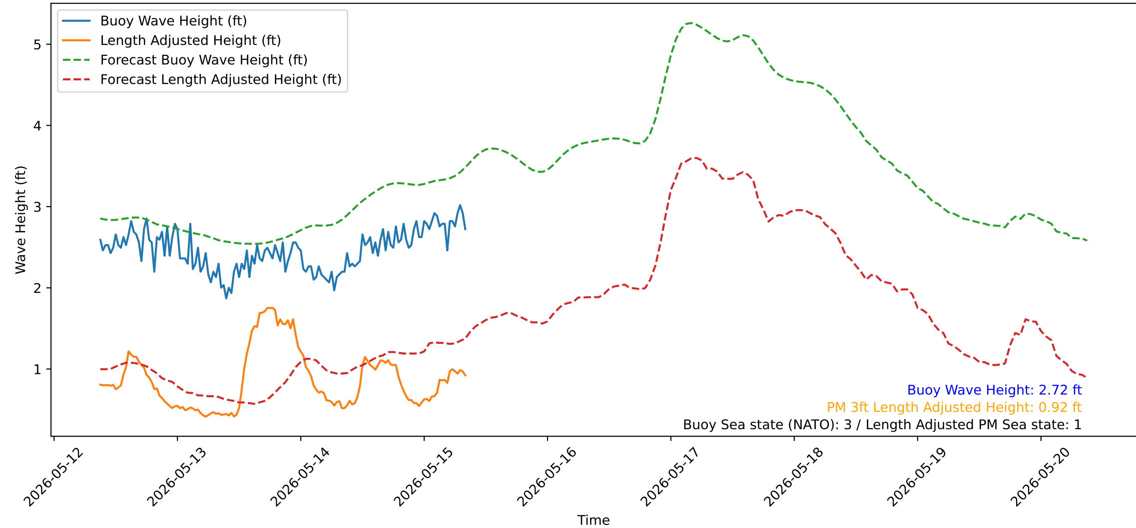
Wave Heights over Time for Red Beach at 2026-05-15 08:40:50
