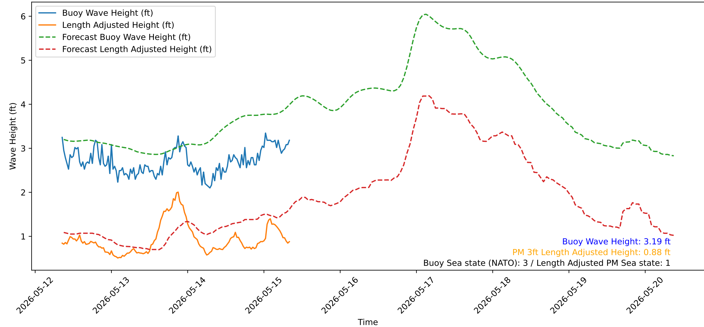
Wave Heights over Time for Green Beach at 2026-05-15 08:41:14
