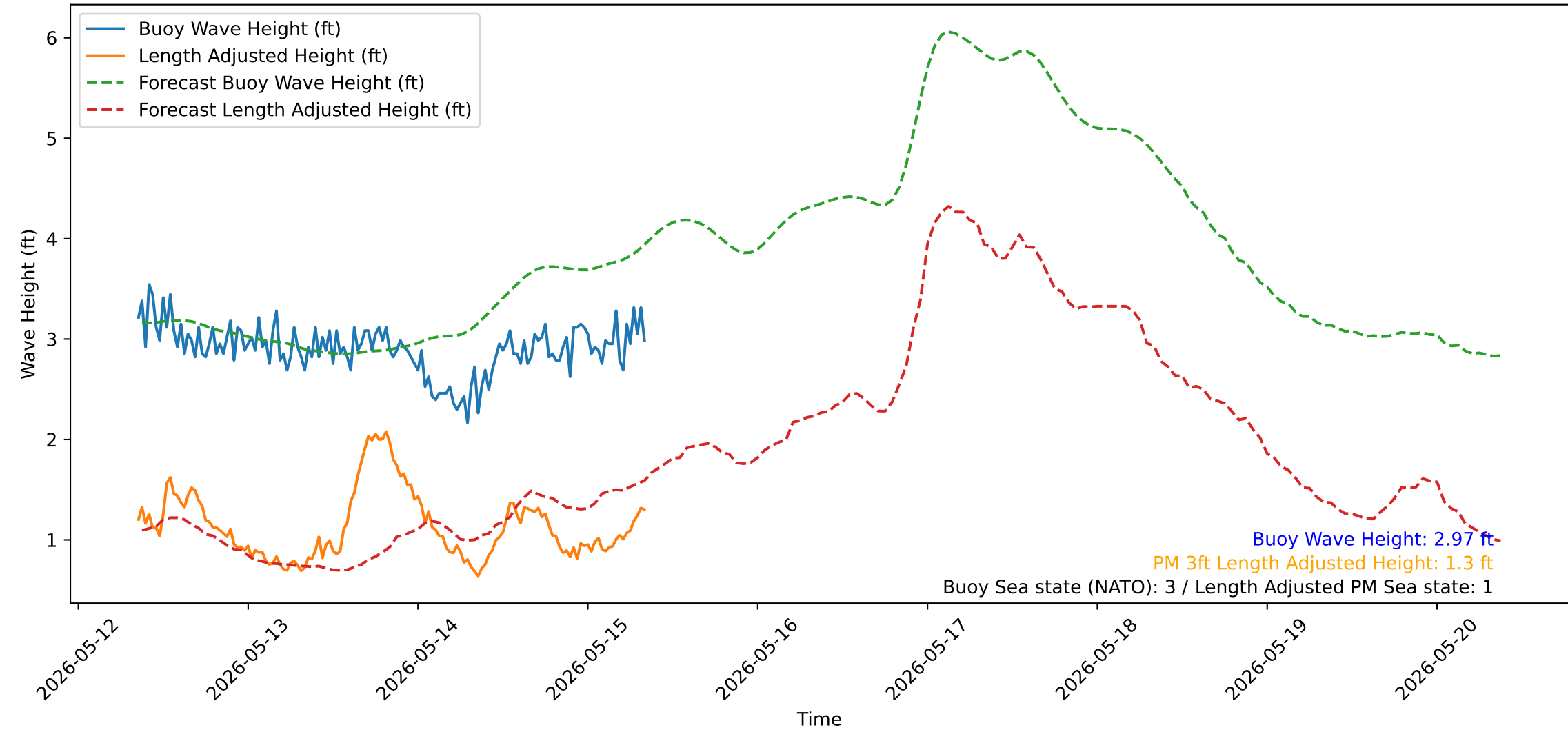
Wave Heights over Time for Oceanside Harbor at 2026-05-15 08:40:31
