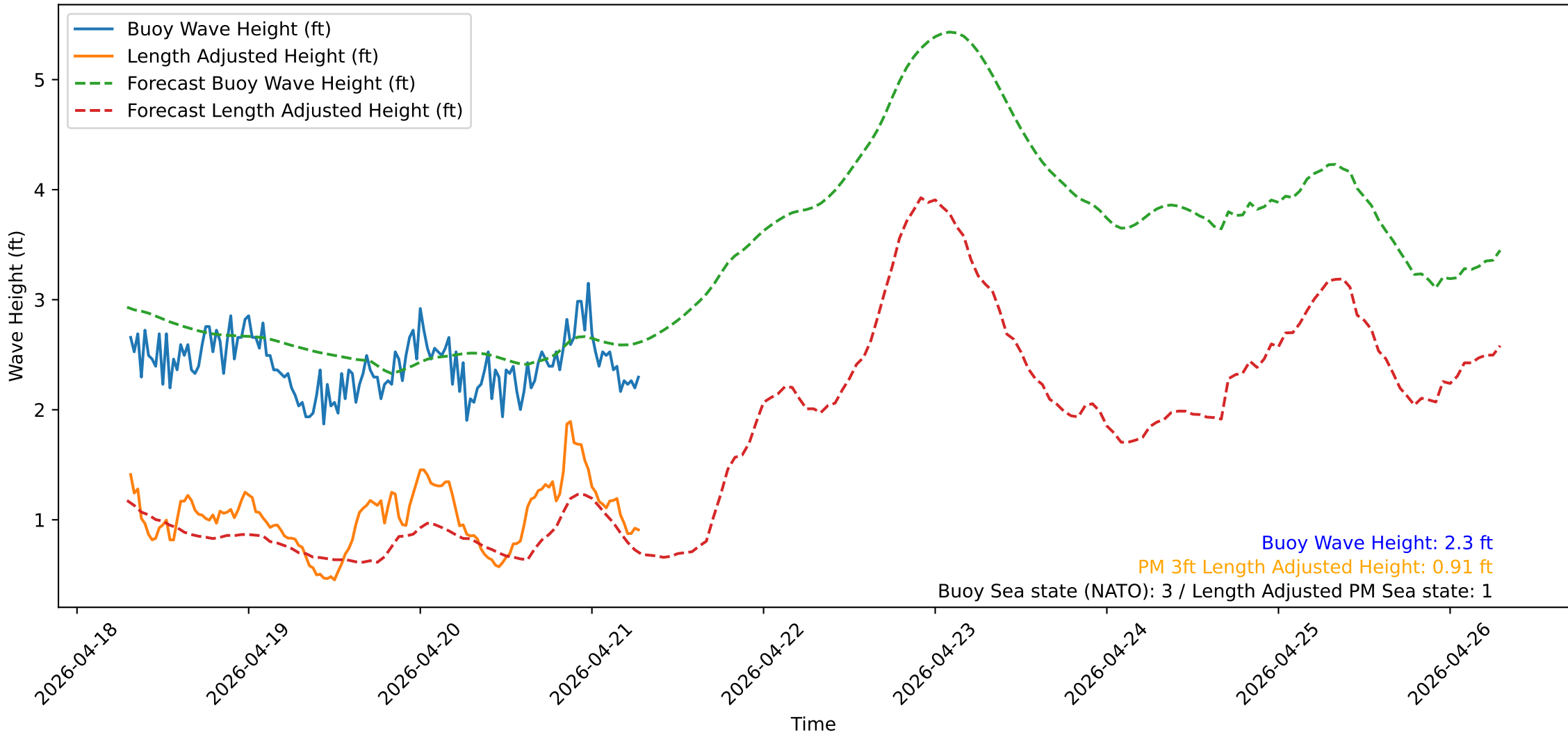
Wave Heights over Time for Green Beach at 2026-04-21 07:21:13
