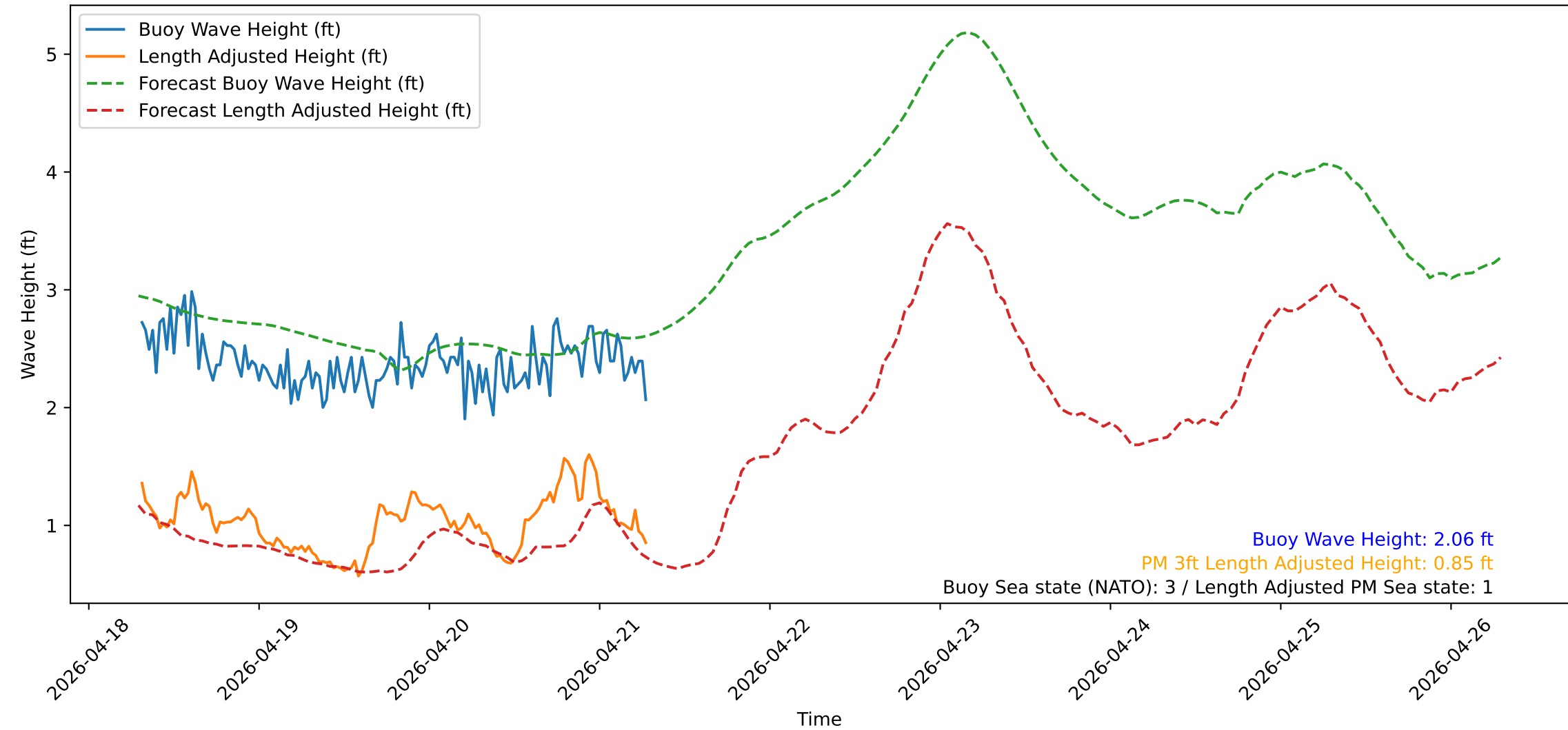
Wave Heights over Time for Oceanside Harbor at 2026-04-21 07:20:31
