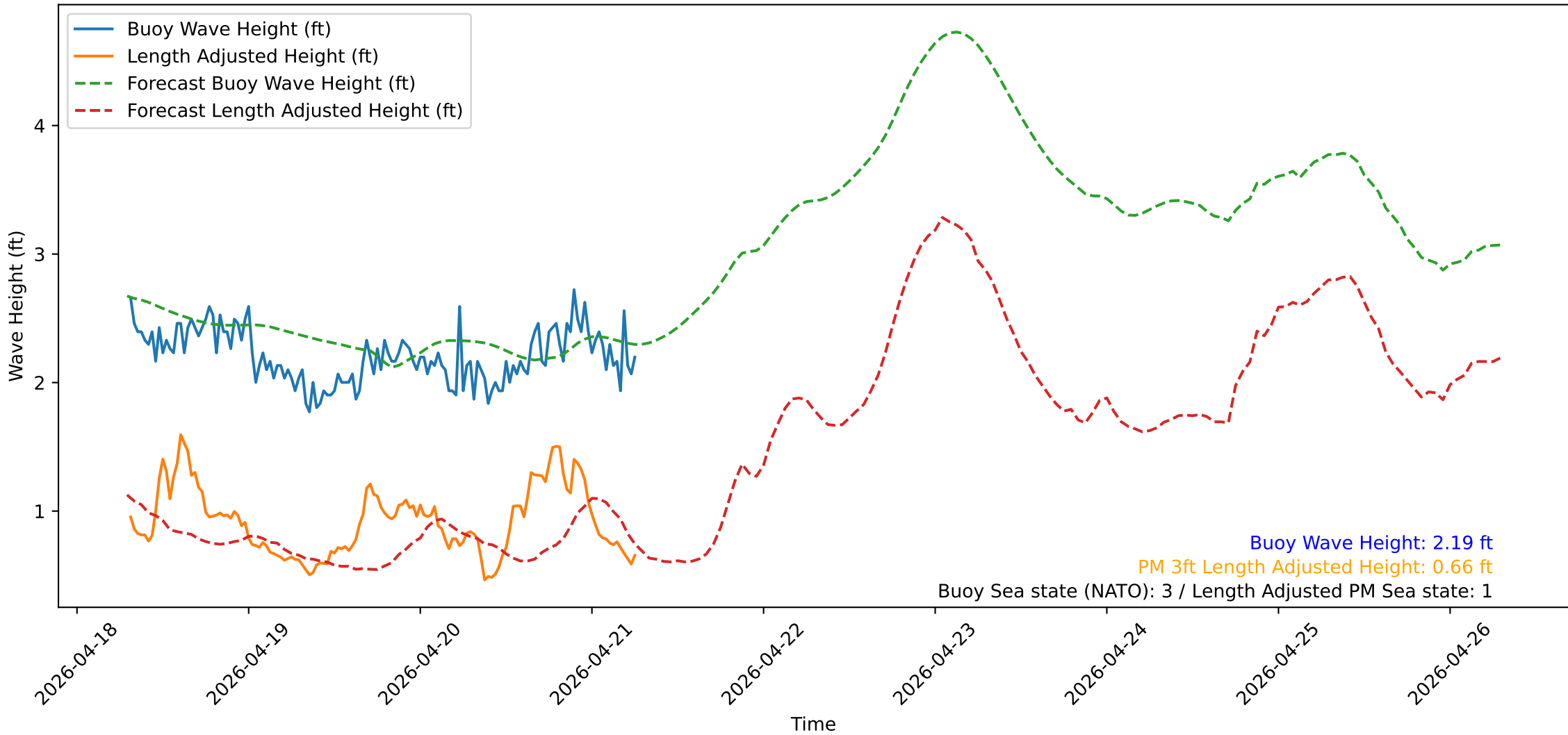
Wave Heights over Time for Red Beach at 2026-04-21 07:20:51
