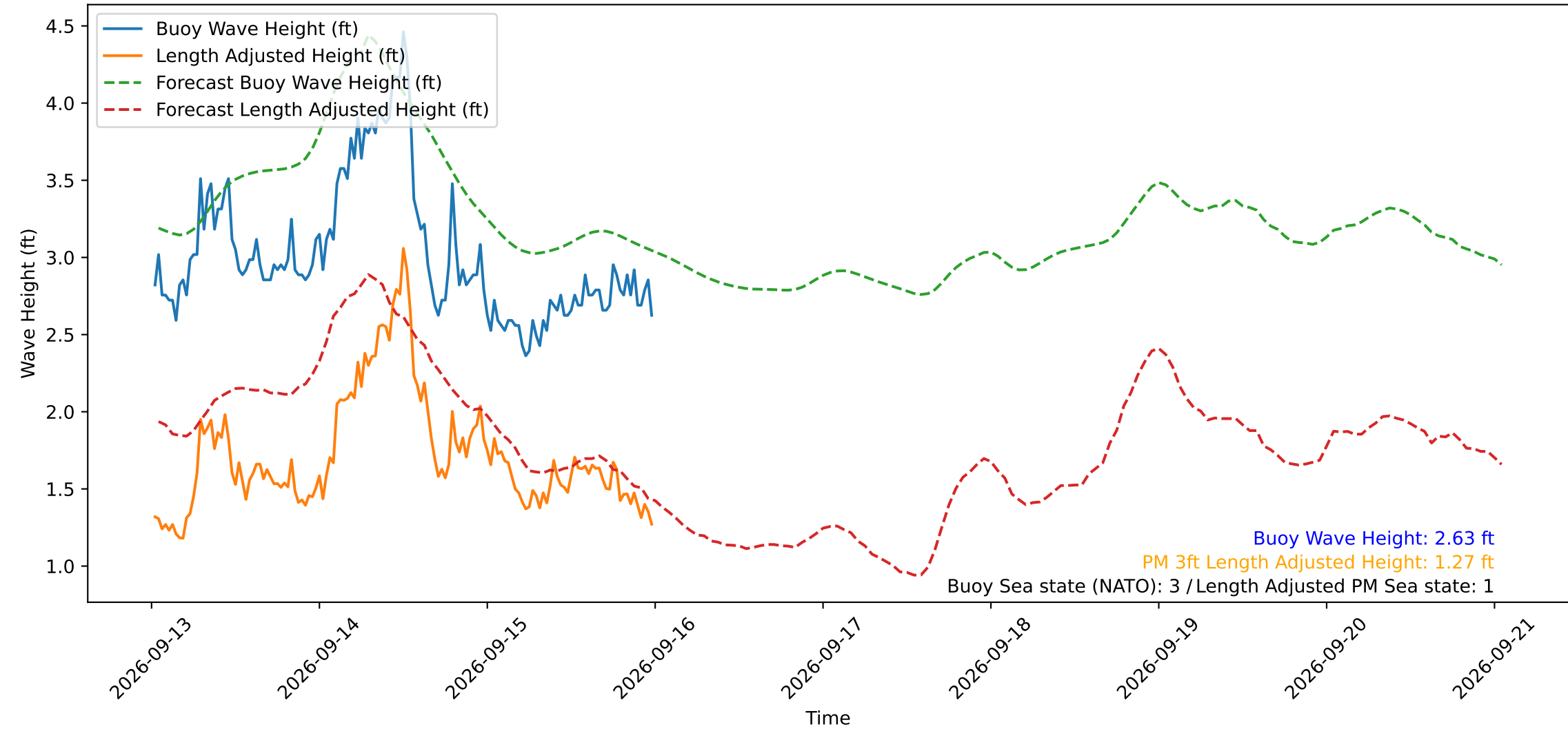
Wave Heights over Time for Oceanside Harbor at 2026-09-16 00:30:30
