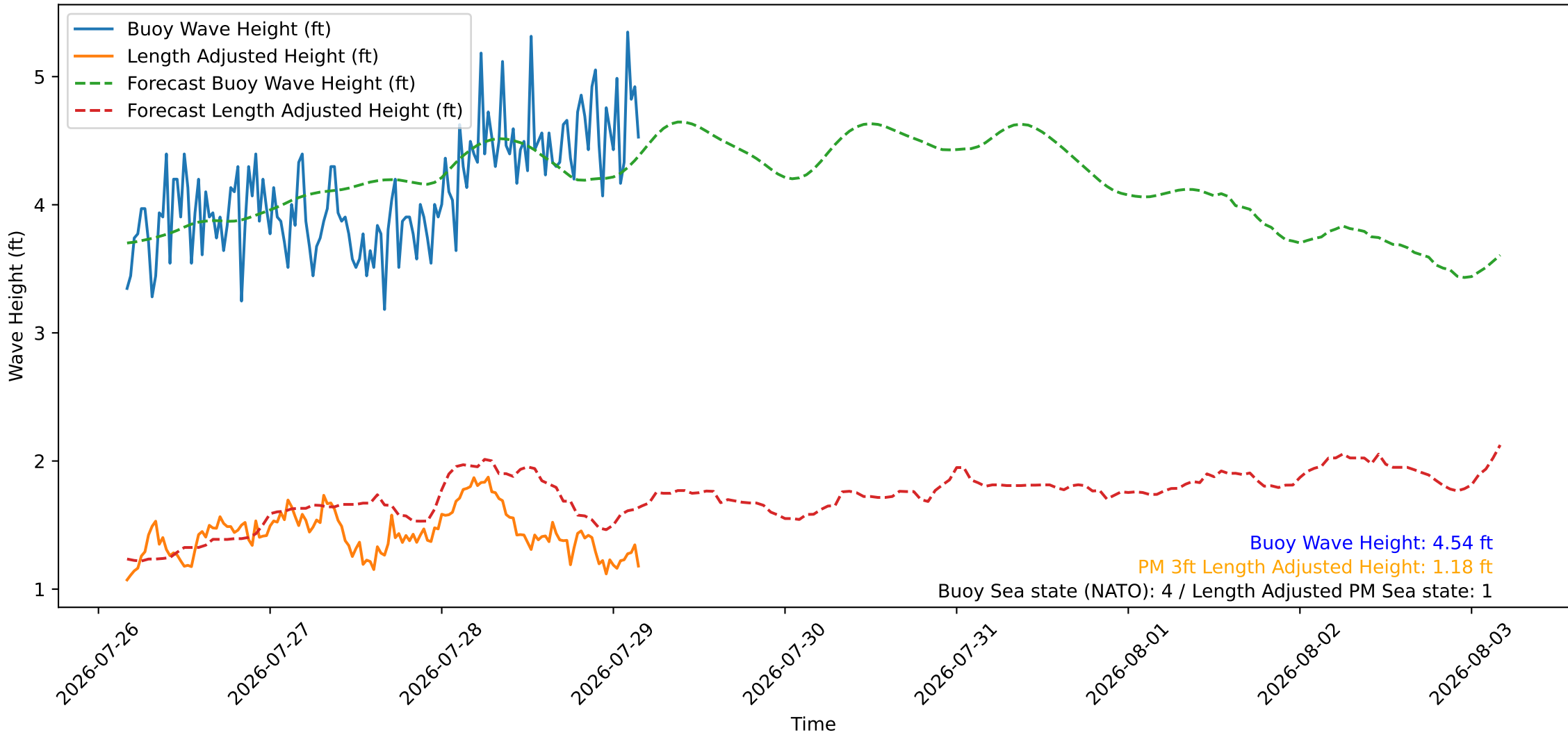
Wave Heights over Time for Oceanside Harbor at 2026-07-29 04:00:26
