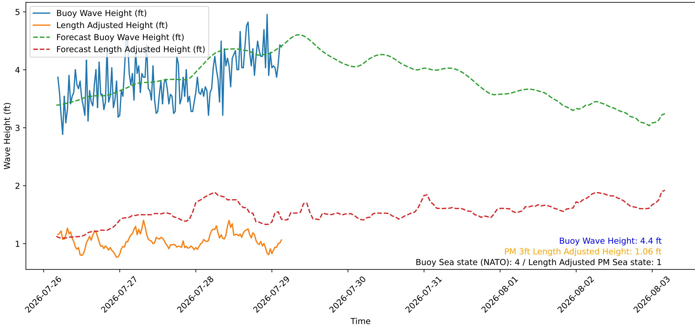
Wave Heights over Time for Red Beach at 2026-07-29 04:00:46
