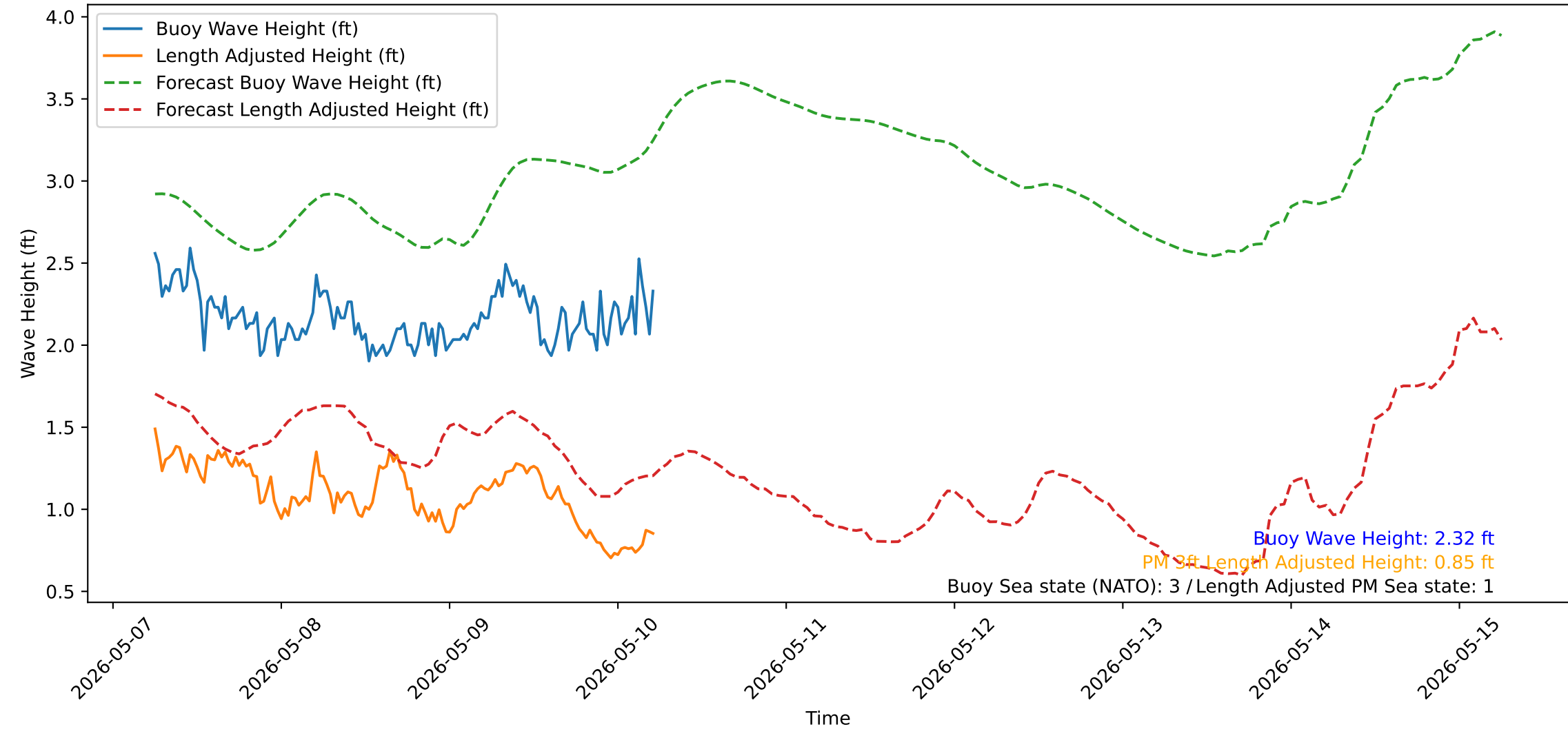
Wave Heights over Time for Red Beach at 2026-05-10 05:50:51
