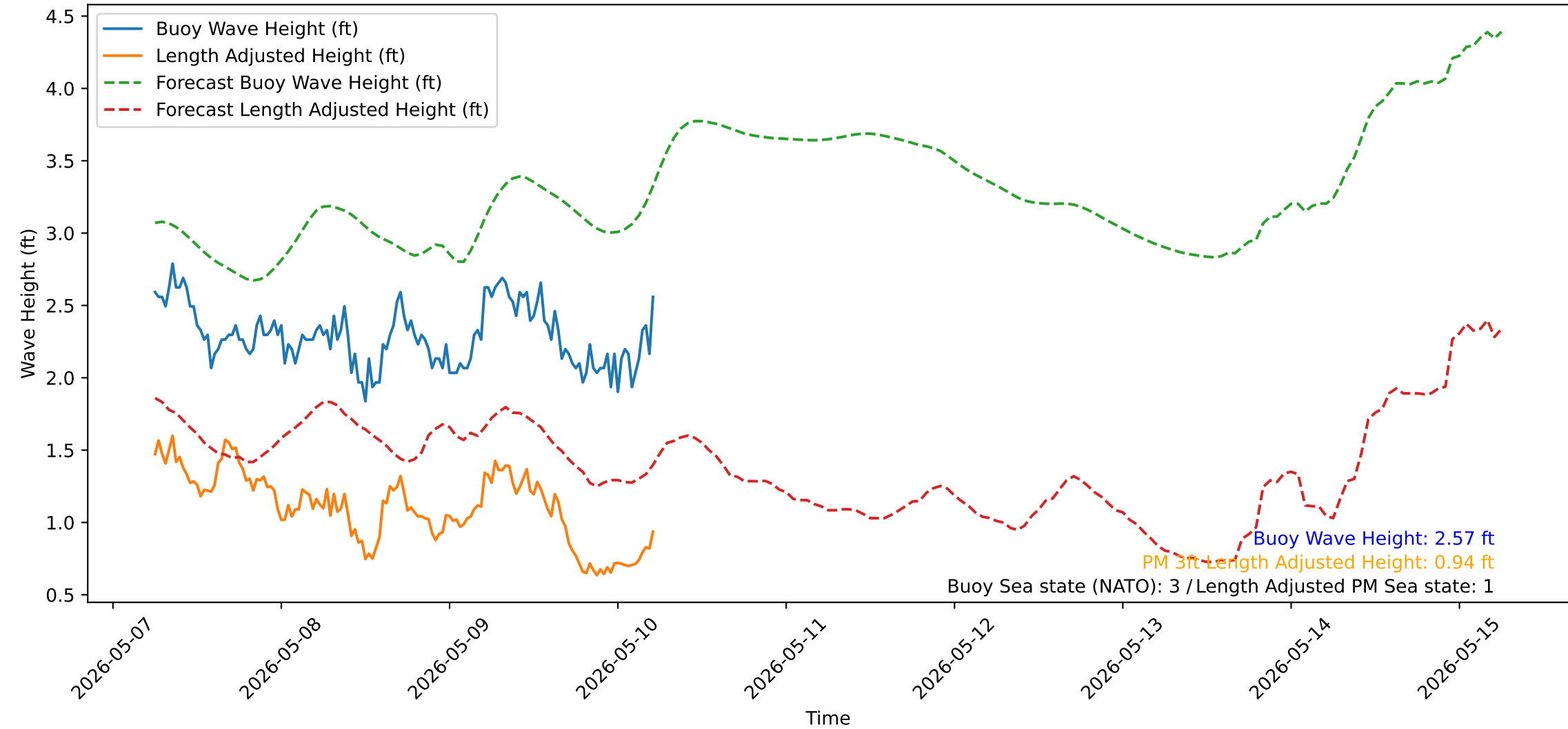
Wave Heights over Time for Green Beach at 2026-05-10 05:51:14
