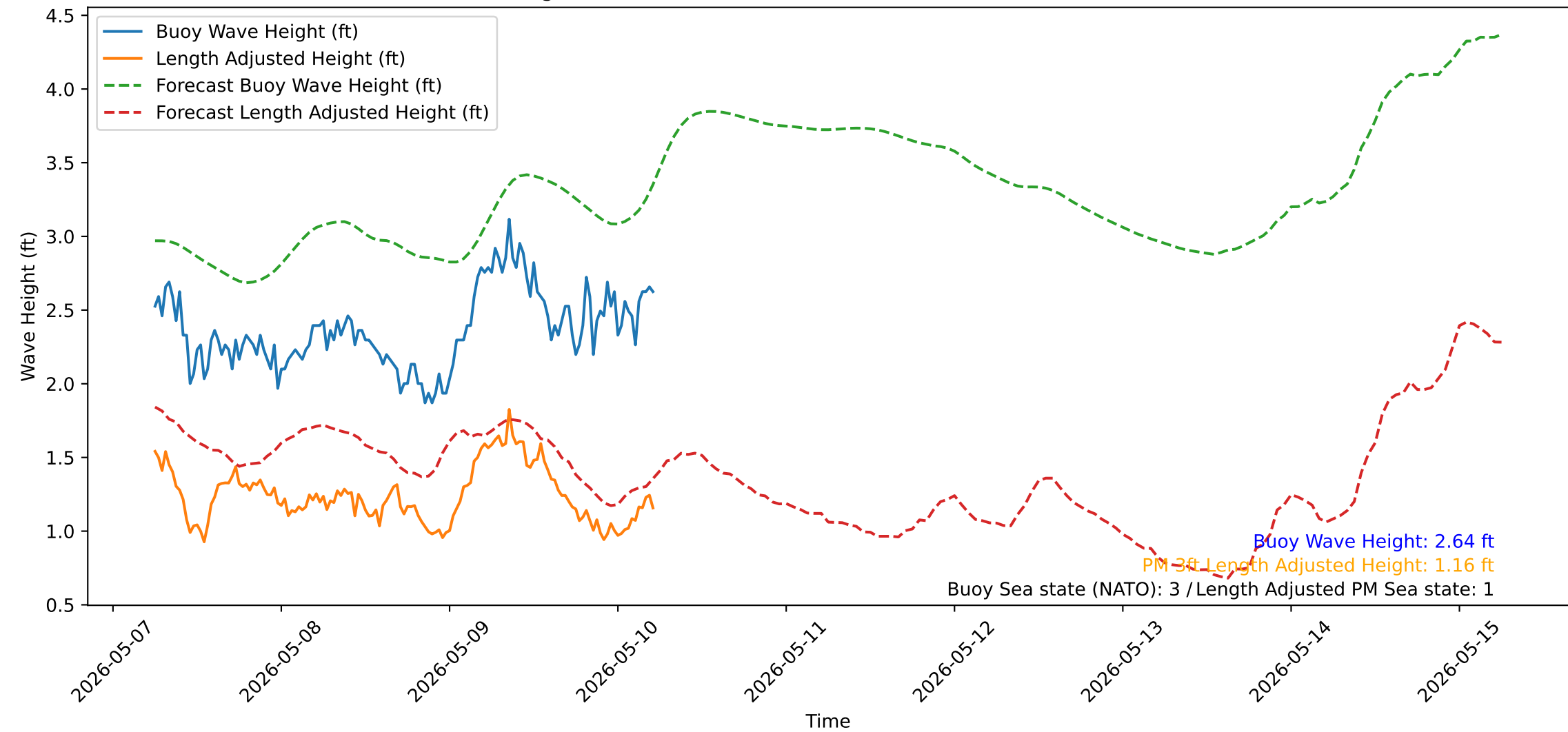
Wave Heights over Time for Oceanside Harbor at 2026-05-10 05:50:30
