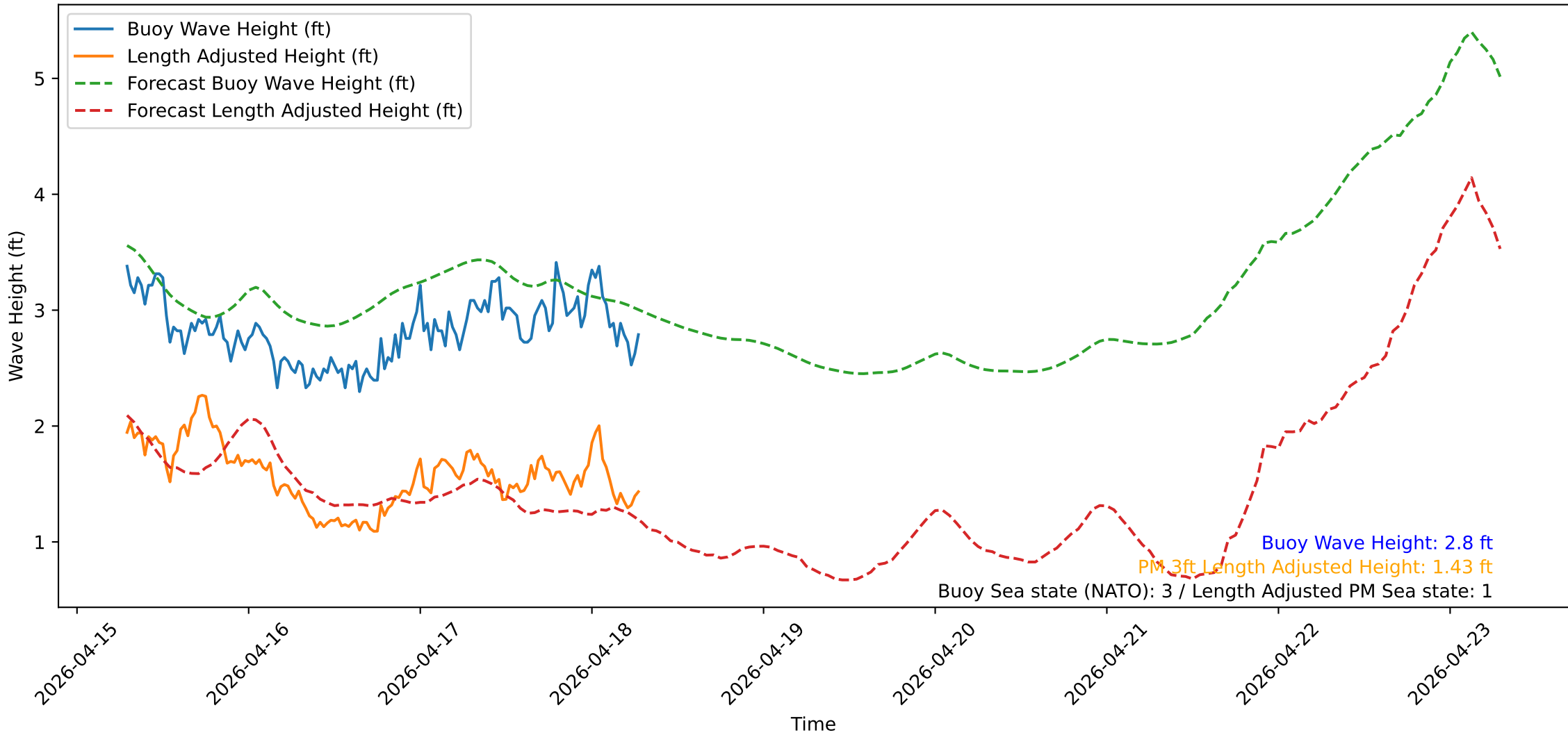
Wave Heights over Time for Oceanside Harbor at 2026-04-18 07:00:31
