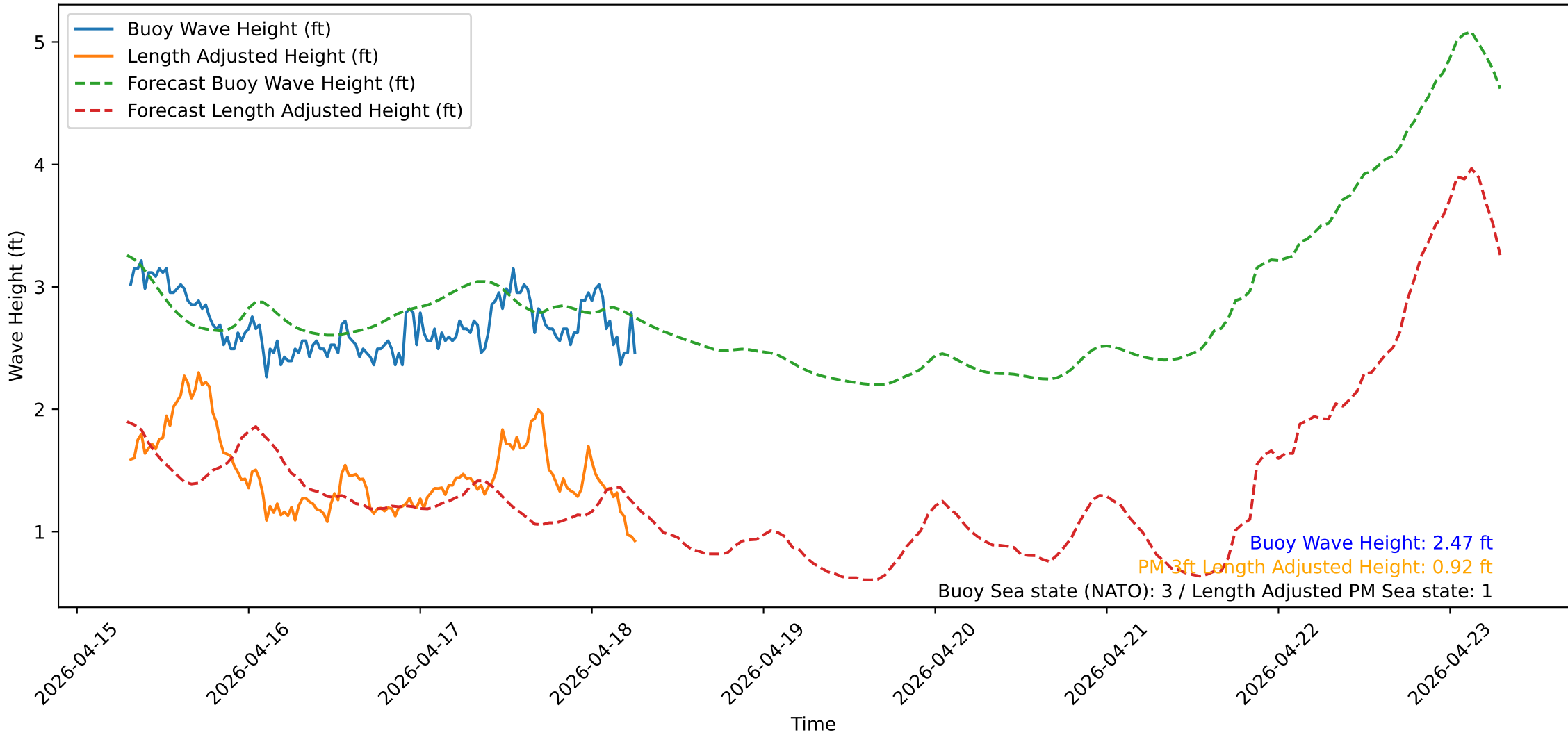
Wave Heights over Time for Red Beach at 2026-04-18 07:00:50
