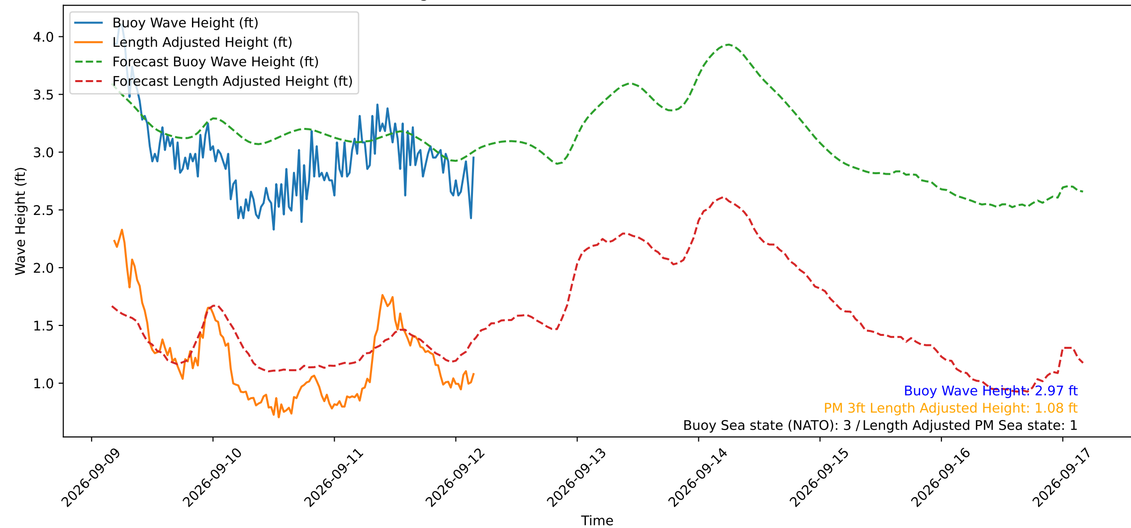
Wave Heights over Time for Red Beach at 2026-09-12 04:10:49
