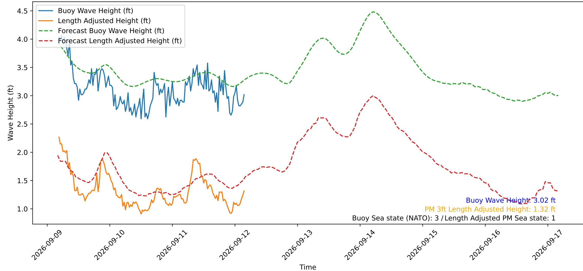
Wave Heights over Time for Green Beach at 2026-09-12 04:11:12
