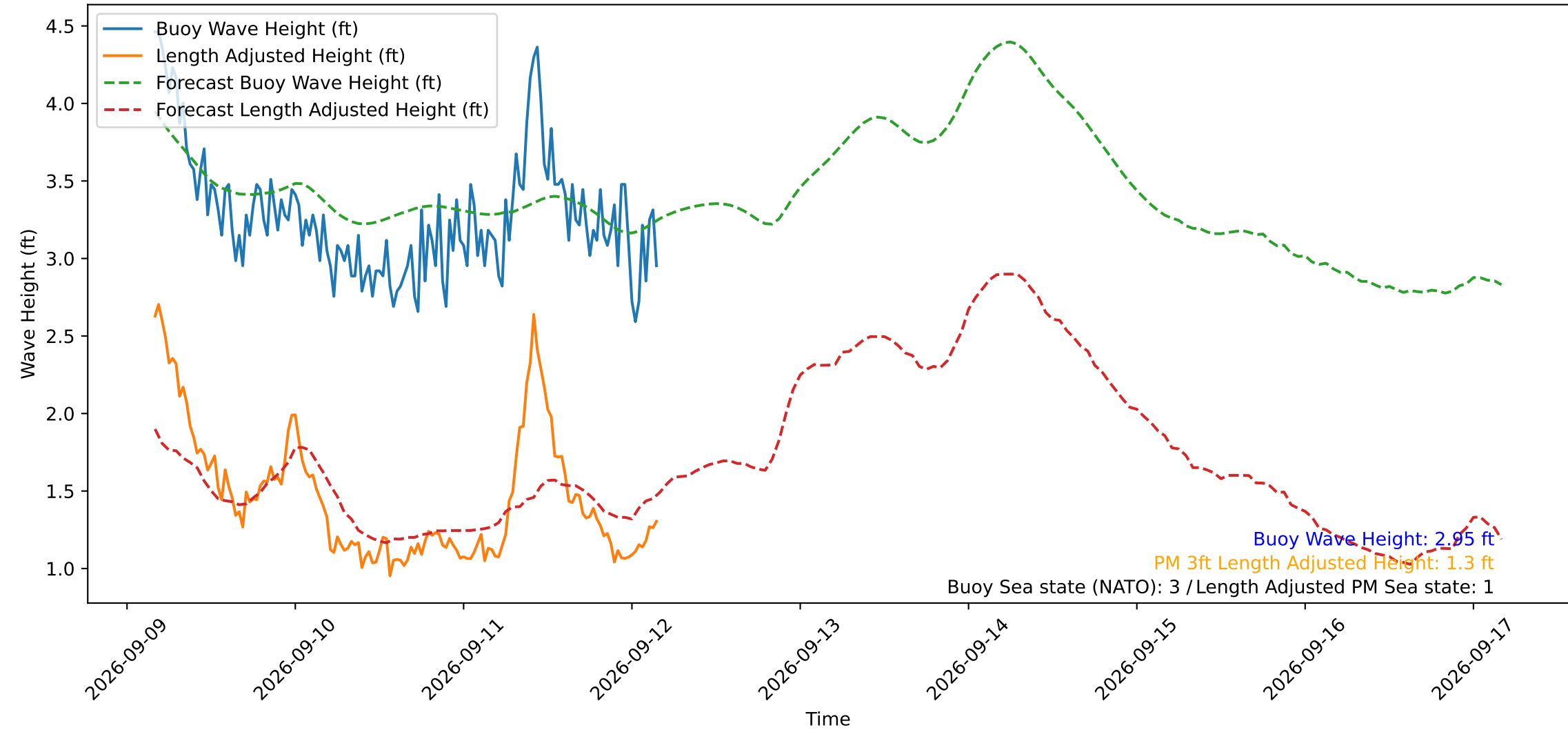
Wave Heights over Time for Oceanside Harbor at 2026-09-12 04:10:30
