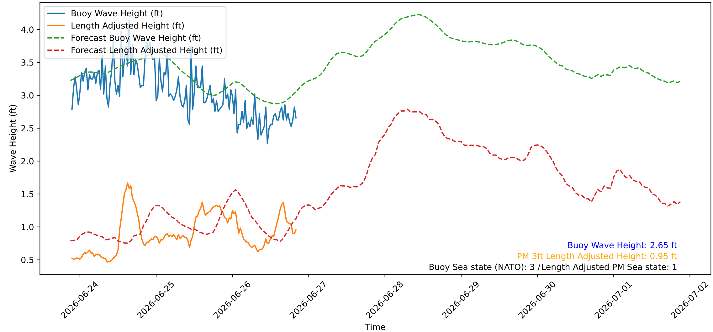
Wave Heights over Time for Red Beach at 2026-06-26 21:20:46
