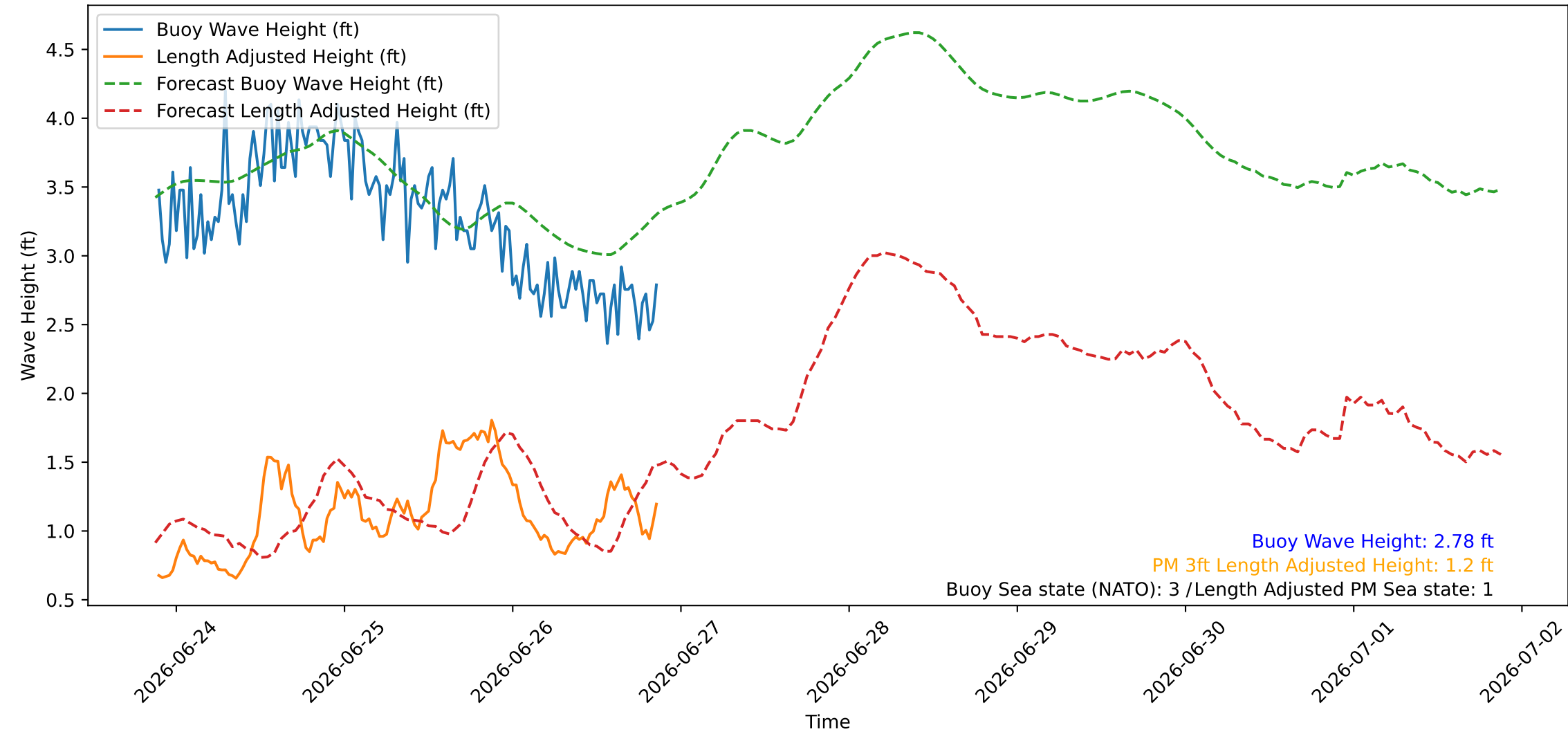
Wave Heights over Time for Green Beach at 2026-06-26 21:21:09
