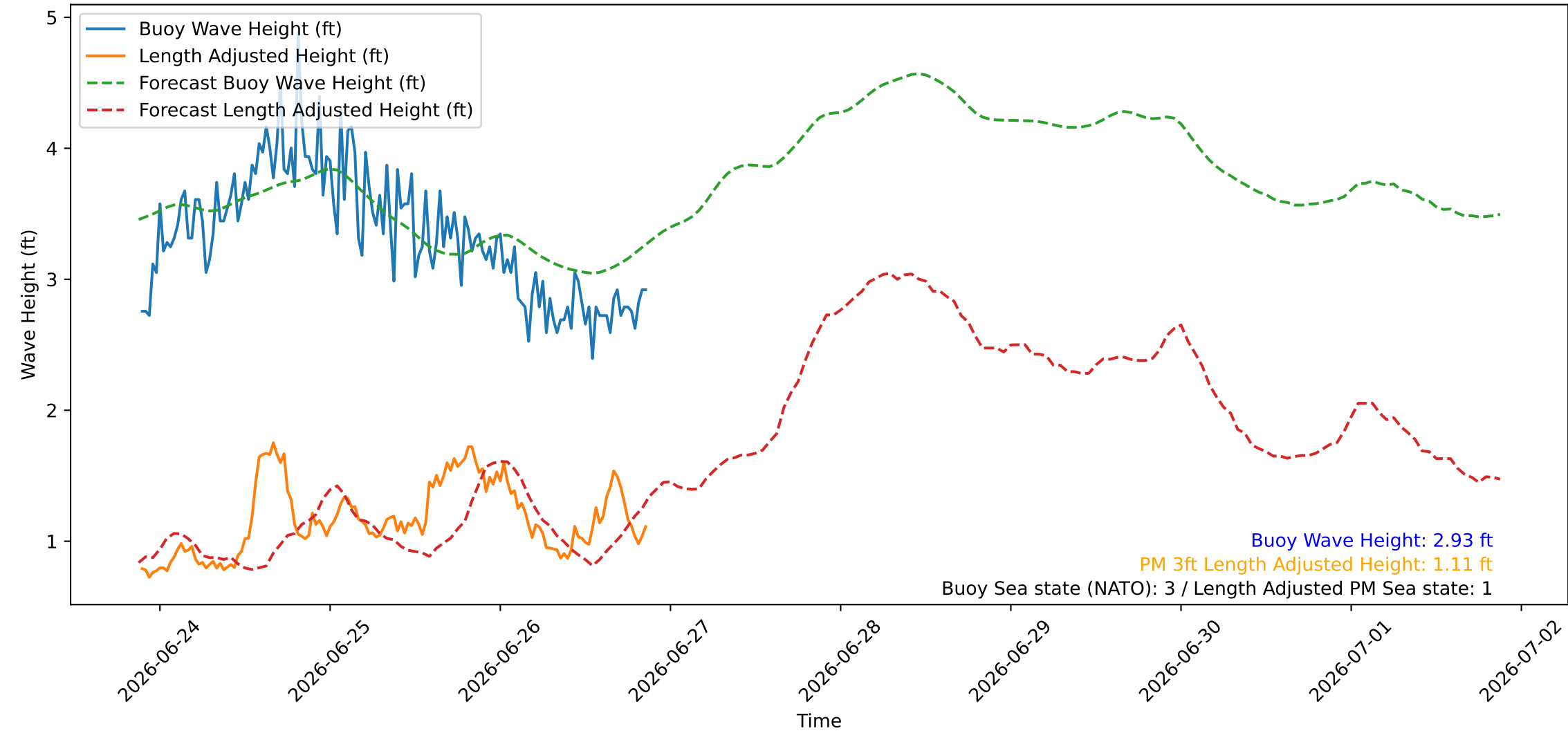
Wave Heights over Time for Oceanside Harbor at 2026-06-26 21:20:25
