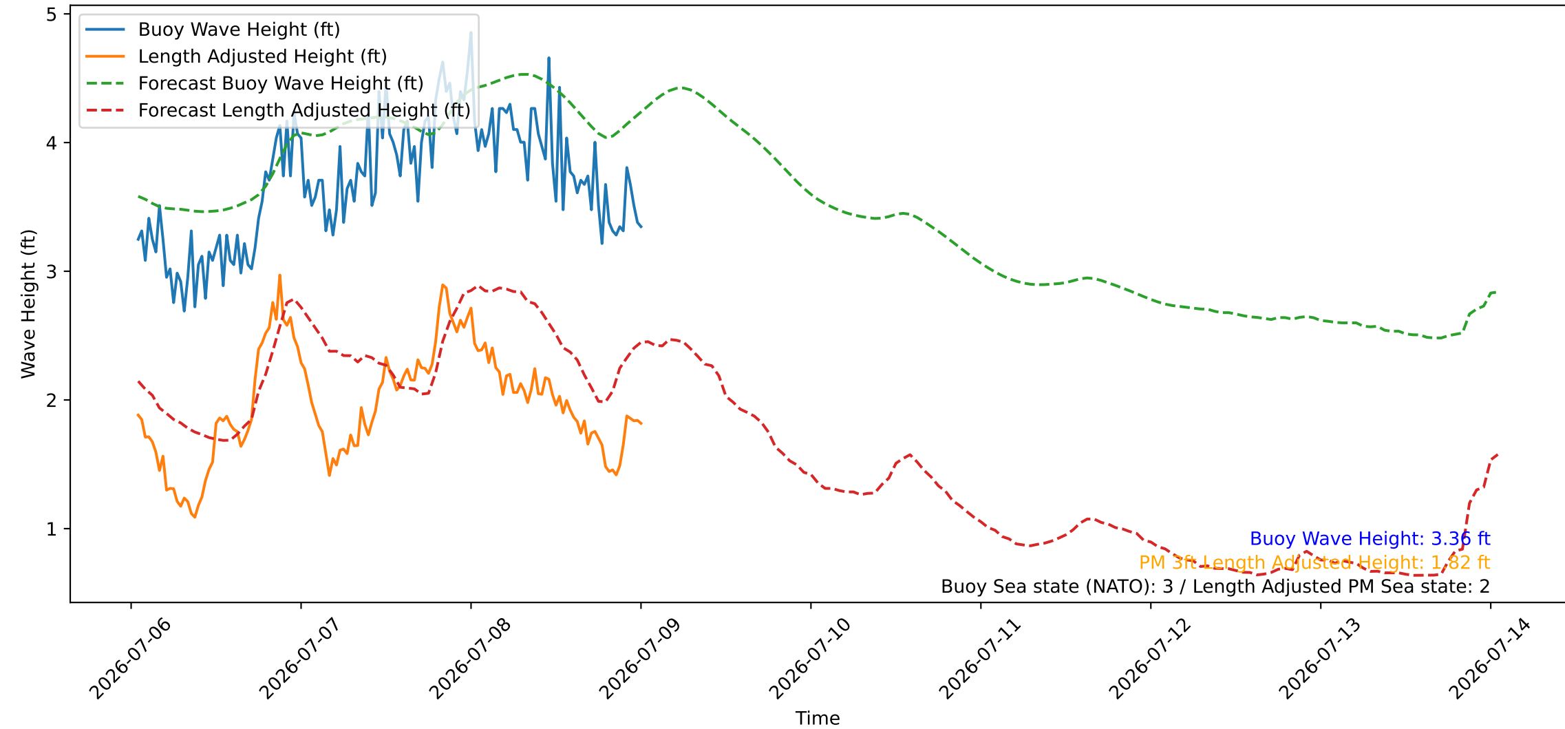
Wave Heights over Time for Red Beach at 2026-07-09 00:50:47
